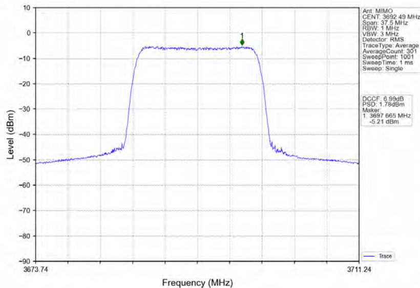
n78d_30kHz_MIMO_NTNV_15MHz_CP-OFDM_16_QAM_3692.49MHz_Inner_Full
