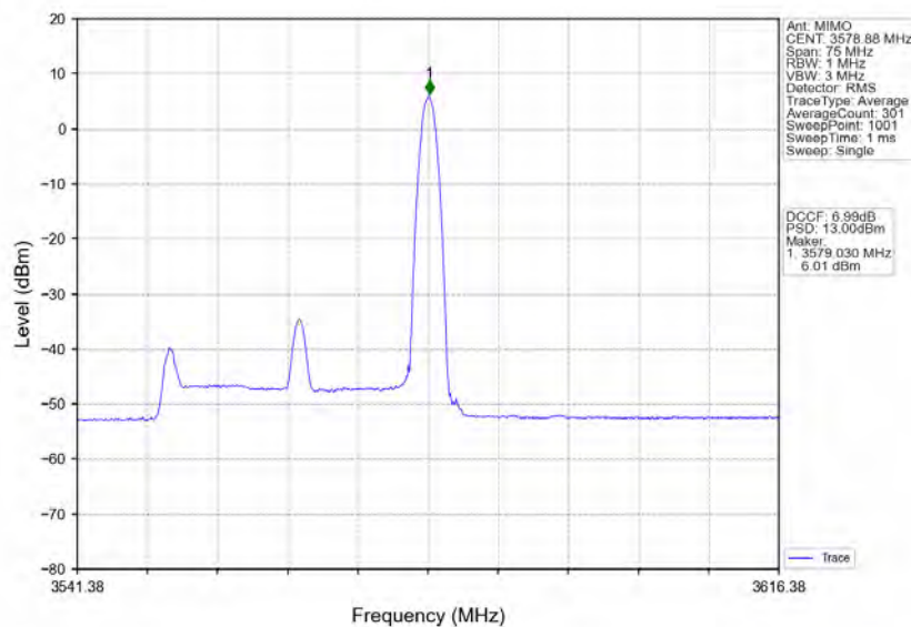
n78d_30kHz_MIMO_NTNV_30MHz_CP-OFDM_256_QAM_3565.02MHz_Edge_1RB_Right
