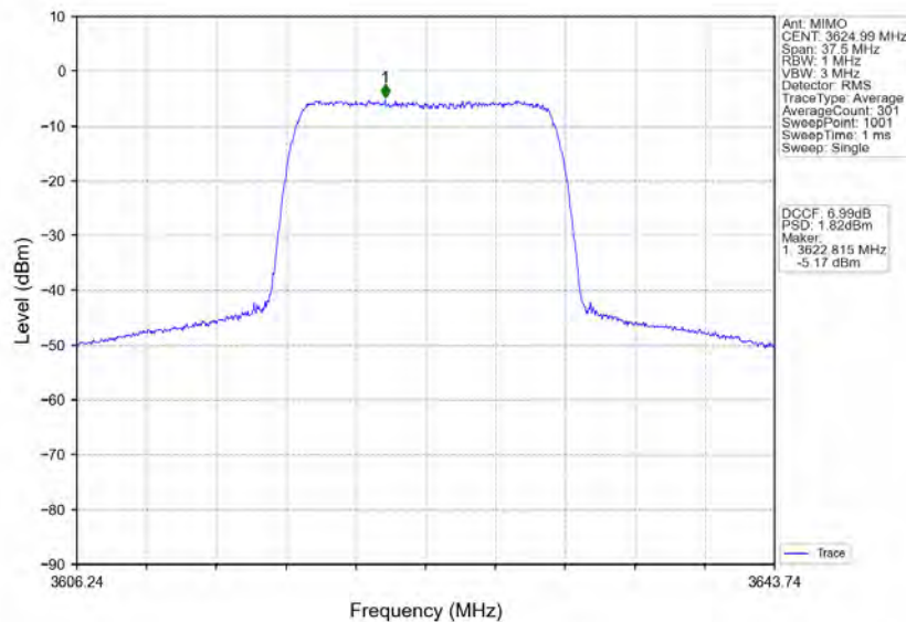
n78d_30kHz_MIMO_NTNV_15MHz_CP-OFDM_16_QAM_3624.99MHz_Inner_Full
