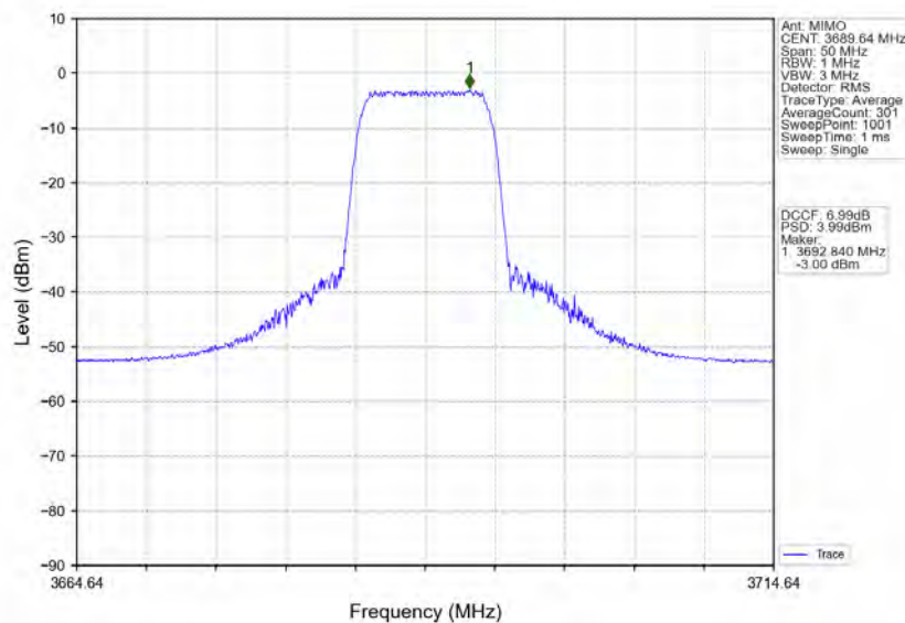
n78d_30kHz_MIMO_NTNV_20MHz_CP-OFDM_16_QAM_3690MHz_Inner_Full
