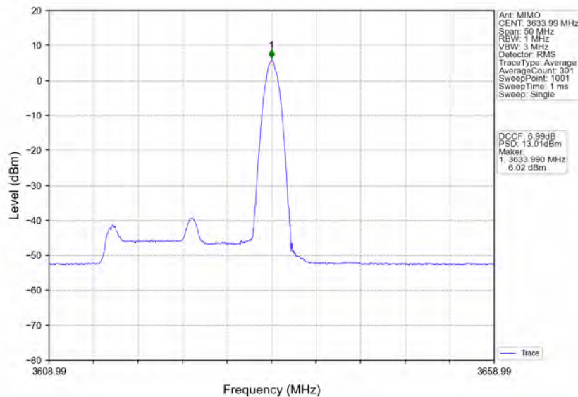
n78d_30kHz_MIMO_NTNV_20MHz_CP-OFDM 16 QAM_3624.99MHz_Edge_1RB_Right
