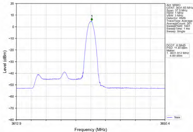
n78d_30kHz_MIMO_NTNV_15MHz_CP-OFDM_QPSK_3624.99MHz_Edge_1RB_Right
