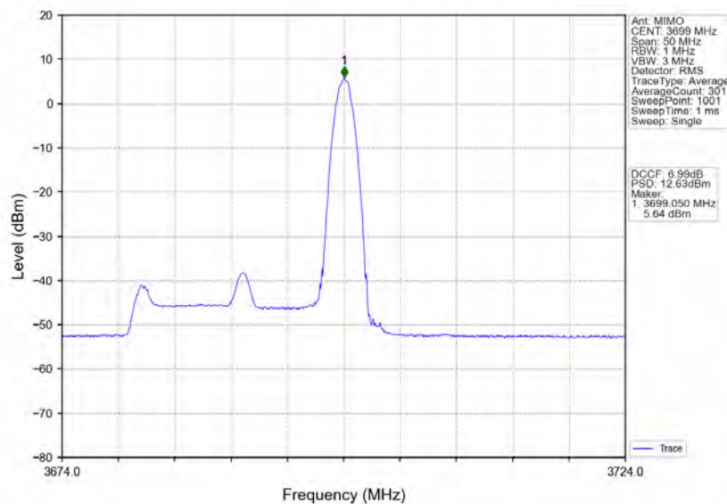
n78d_30kHz_MIMO_NTNV_20MHz_CP-OFDM 16 QAM_3690MHz_Edge_1RB_Right
