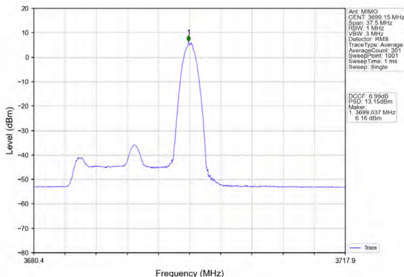
n78d_30kHz_MIMO_NTNV_15MHz_CP-OFDM_256_QAM_3692.49MHz_Edge_1RB_Right
