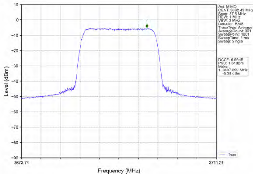
n78d_30kHz_MIMO_NTNV_15MHz_CP-OFDM 64 QAM_3692.49MHz_Inner_Full
