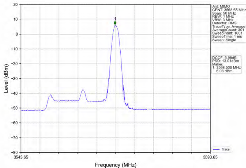
n78d_30kHz_MIMO_NTNV_20MHz_CP-OFDM 16 QAM_3560.01MHz_Inner_1RB_Right
