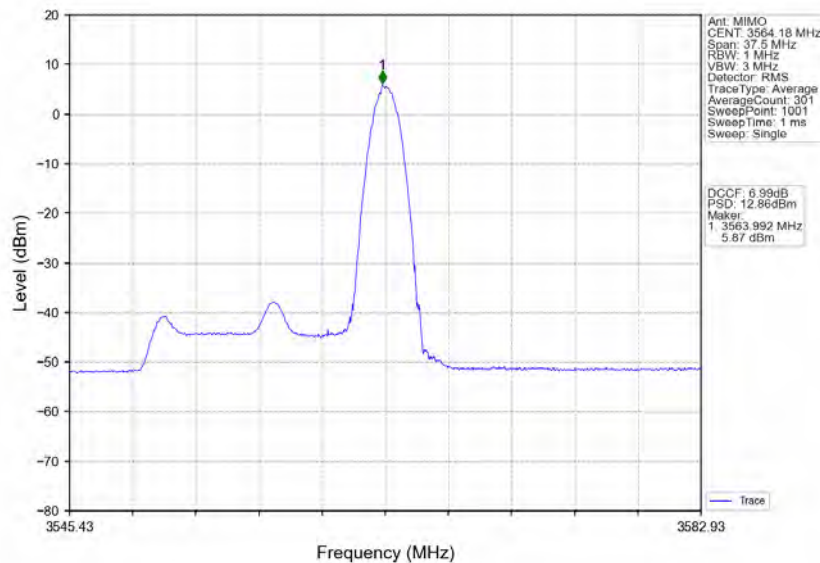
n78d_30kHz_MIMO_NTNV_15MHz_CP-OFDM_16_QAM_3557.52MHz_Edge_1RB_Right
