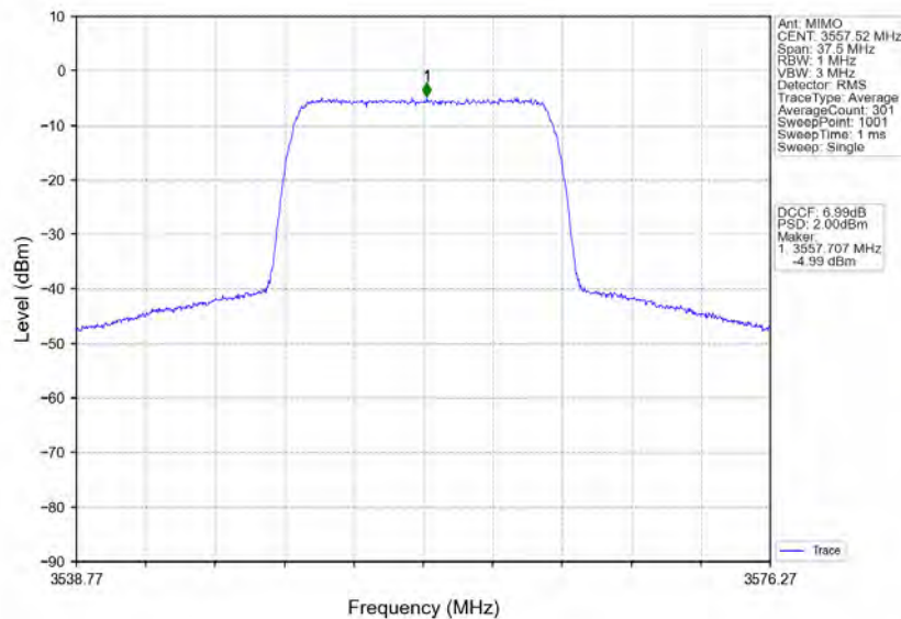
n78d_30kHz_MIMO_NTNV_15MHz_CP-OFDM_256_QAM_3557.52MHz_Inner_Full
