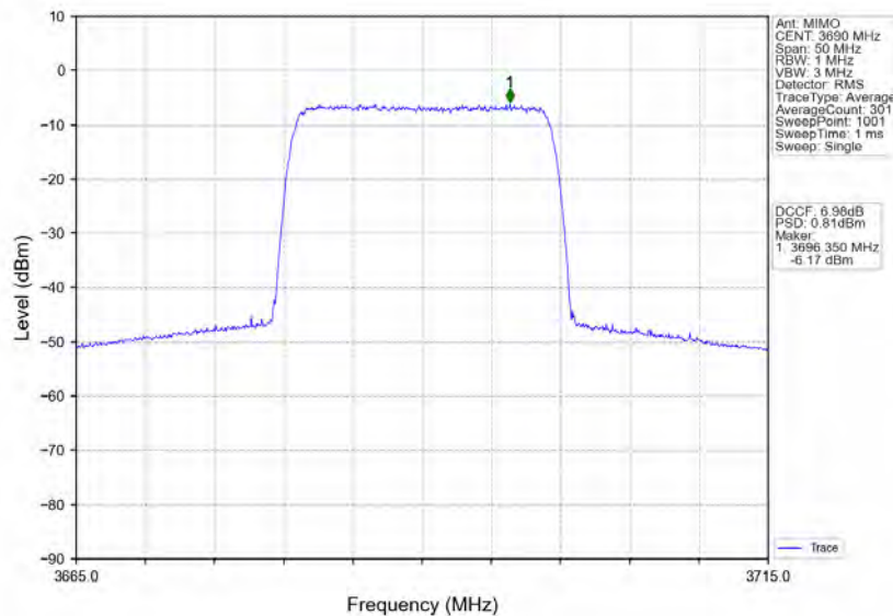
n78d_30kHz_MIMO_NTNV_20MHz_CP-OFDM_256_QAM_3690MHz_Inner_Full
