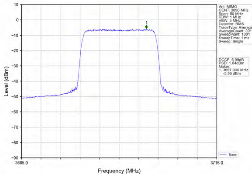
n78d_30kHz_MIMO_NTNV_20MHz_CP-OFDM_64_QAM_3690MHz_Inner_Full
