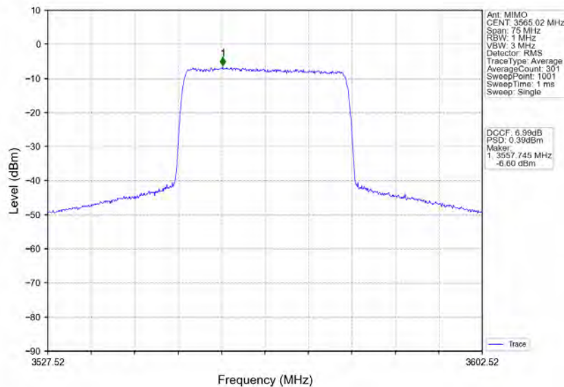
n78d_30kHz_MIMO_NTNV_30MHz_CP-OFDM 64 QAM_3565.02MHz_Inner_Full
