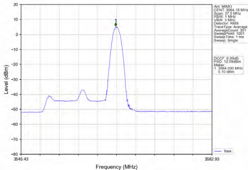
n78d_30kHz_MIMO_NTNV_15MHz_CP-OFDM 64 QAM_3557.52MHz_Edge_1RB_Right
