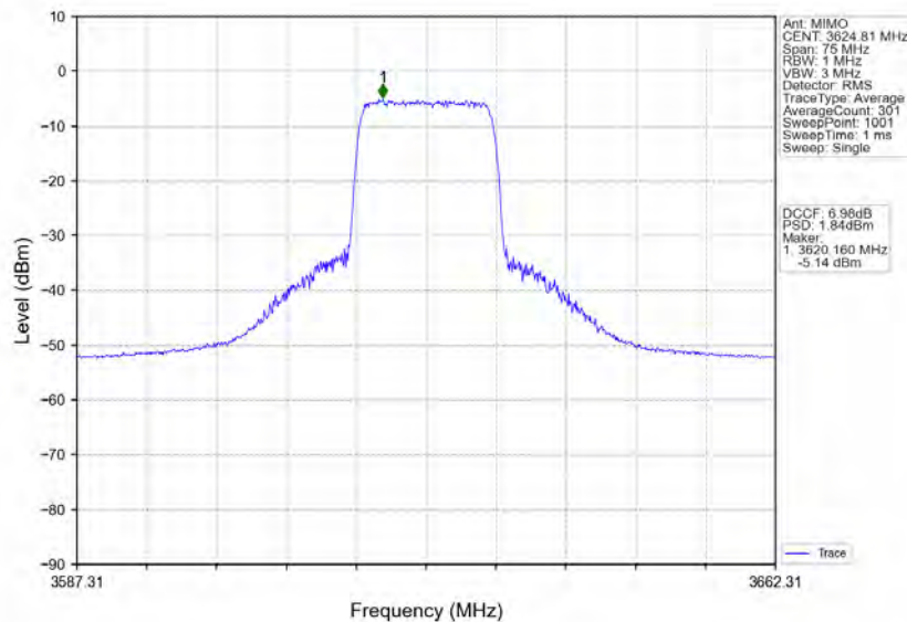
n78d_30kHz_MIMO_NTNV_30MHz_CP-OFDM QPSK_3624.99MHz_Inner_Full
