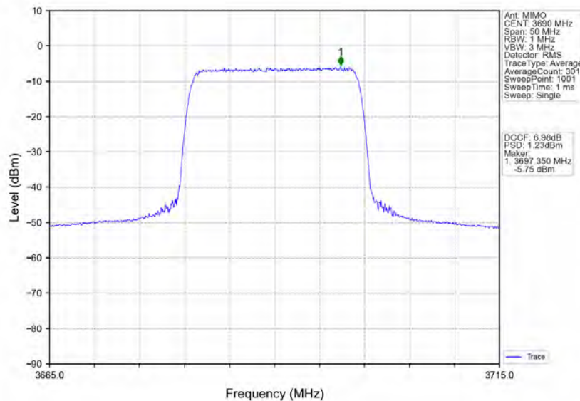
n78d_30kHz_MIMO_NTNV_20MHz_CP-OFDM_QPSK_3690MHz_Inner_Full
