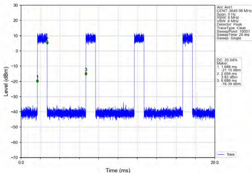
n78d_30kHz_MIMO_NTNV_100MHz_CP-OFDM_256_QAM_3649.98MHz_Inner_Full
