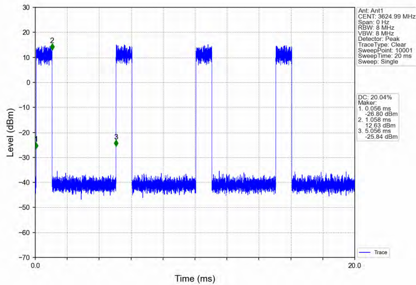
n78d_30kHz_MIMO_NTNV_100MHz_CP-OFDM_64_QAM_3624.99MHz_Inner_Full
