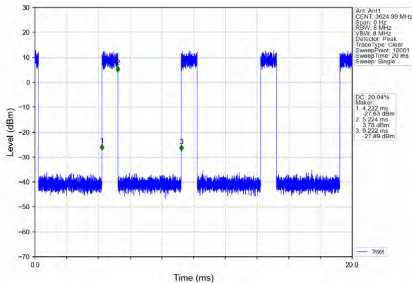
n78d_30kHz_MIMO_NTNV_90MHz_CP-OFDM_256_QAM_3624.99MHz_Inner_Full
