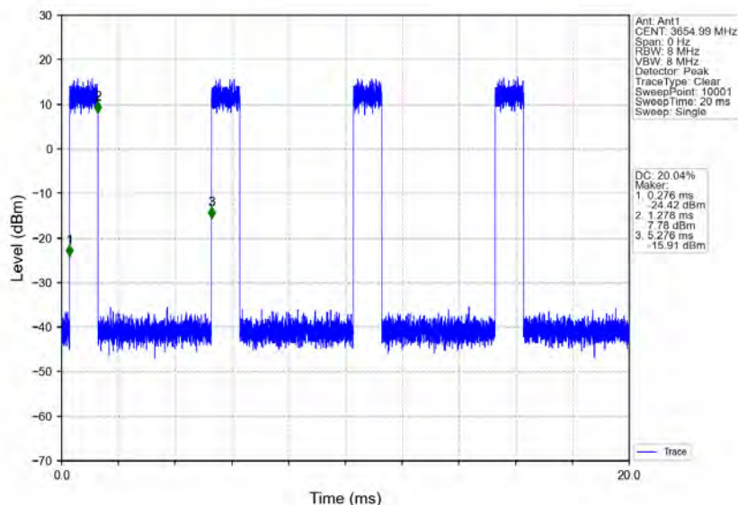
n78d_30kHz_MIMO_NTNV_90MHz_CP-OFDM_256_QAM_3654.99MHz_Inner_Full
