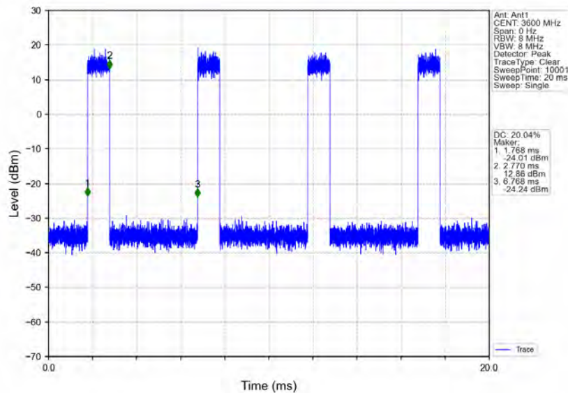
n78d_30kHz_MIMO_NTNV_100MHz_CP-OFDM_64_QAM_3600MHz_Inner_Full
