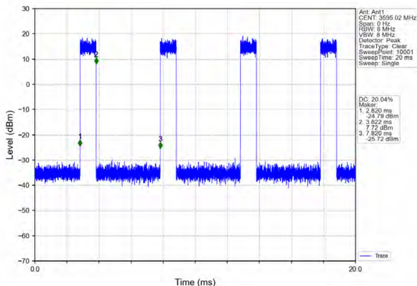
n78d_30kHz_MIMO_NTNV_90MHz_CP-OFDM 64 QAM_3595.02MHz_Inner_Full
