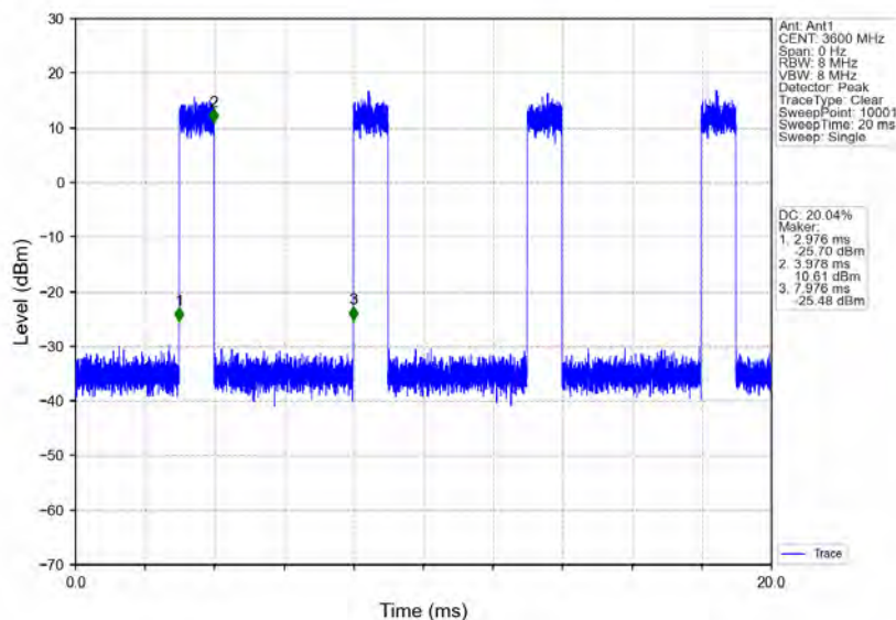
n78d_30kHz_MIMO_NTNV_100MHz_CP-OFDM_16_QAM_3600MHz_Inner_Full
