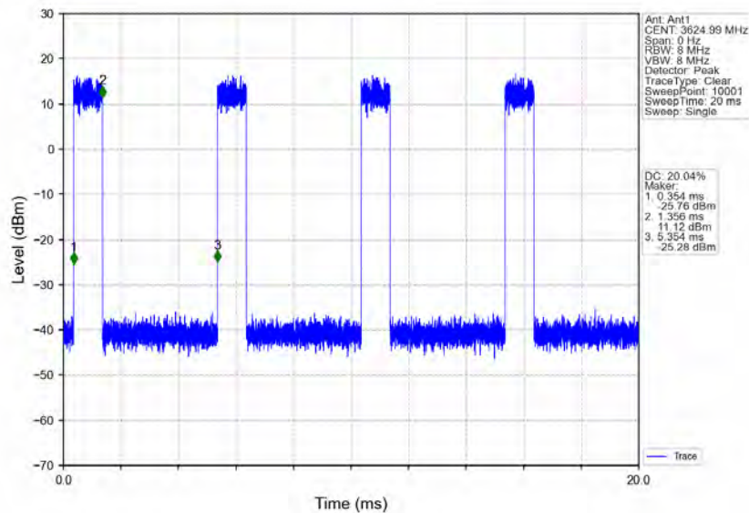
n78d_30kHz_MIMO_NTNV_90MHz_CP-OFDM_16_QAM_3624.99MHz_Inner_Full
