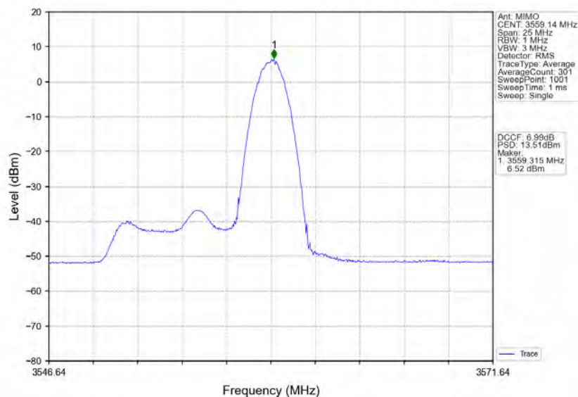
n78d_30kHz_MIMO_NTNV_10MHz_CP-OFDM QPSK_3555MHz_Edge_1RB_Right
