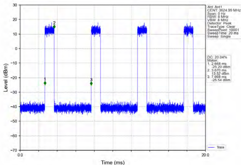
n78d_30kHz_MIMO_NTNV_80MHz_CP-OFDM_16_QAM_3624.99MHz_Inner_Full
