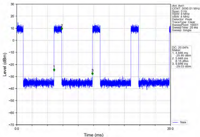
n78d_30kHz_MIMO_NTNV_80MHz_CP-OFDM_256_QAM_3590.01MHz_Inner_Full
