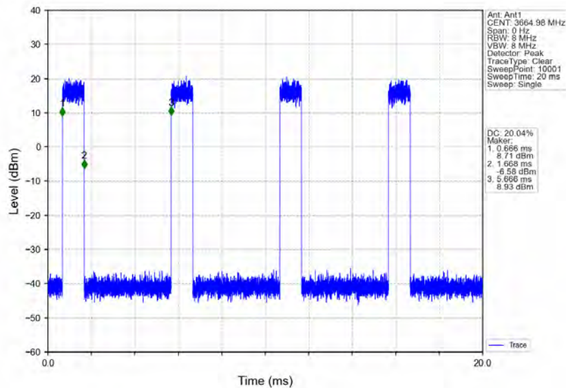
n78d_30kHz_MIMO_NTNV_70MHz_CP-OFDM 64 QAM_3664.98MHz_Inner_Full
