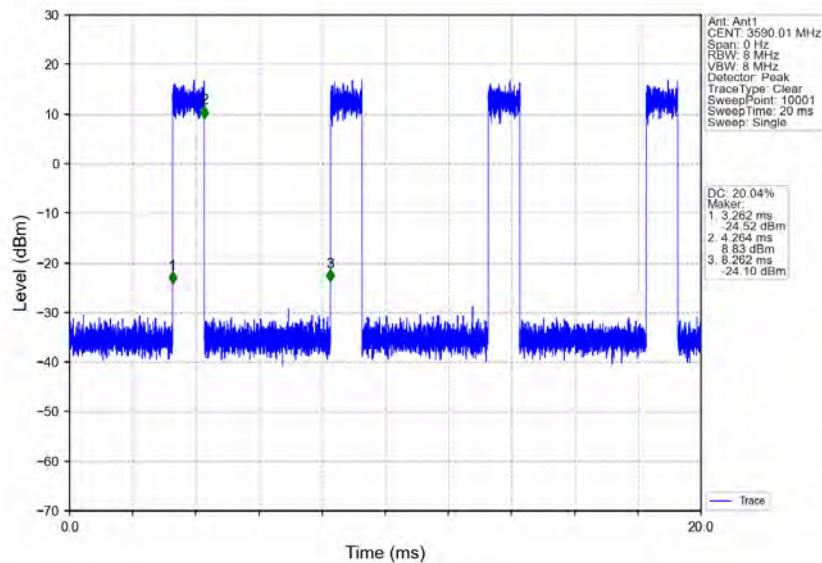
n78d_30kHz_MIMO_NTNV_80MHz_CP-OFDM_QPSK_3590.01MHz_Inner_Full
