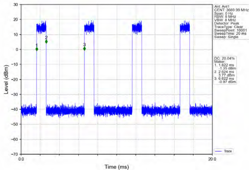
n78d_30kHz_MIMO_NTNV_60MHz_CP-OFDM_QPSK_3669.99MHz_Inner_Full
