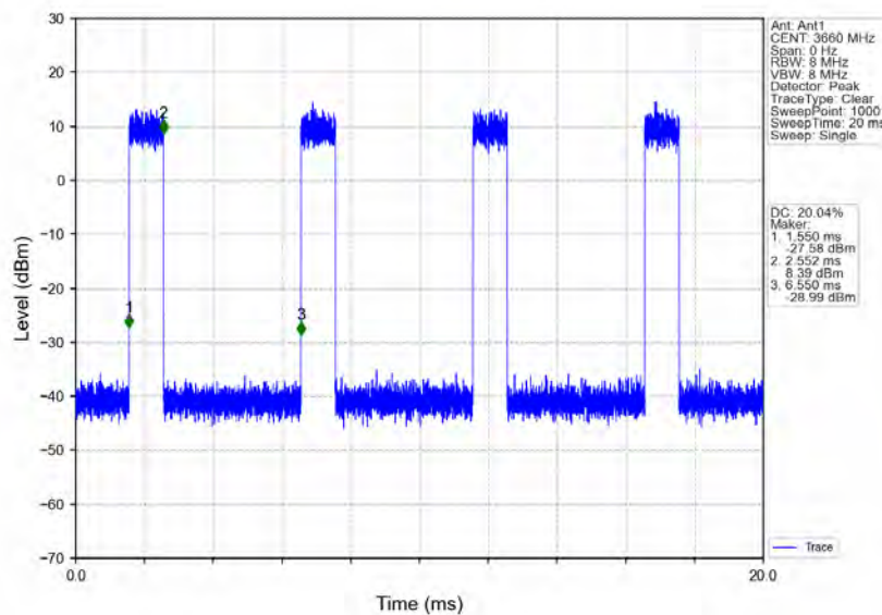
n78d_30kHz_MIMO_NTNV_80MHz_CP-OFDM_256_QAM_3660MHz_Inner_Full
