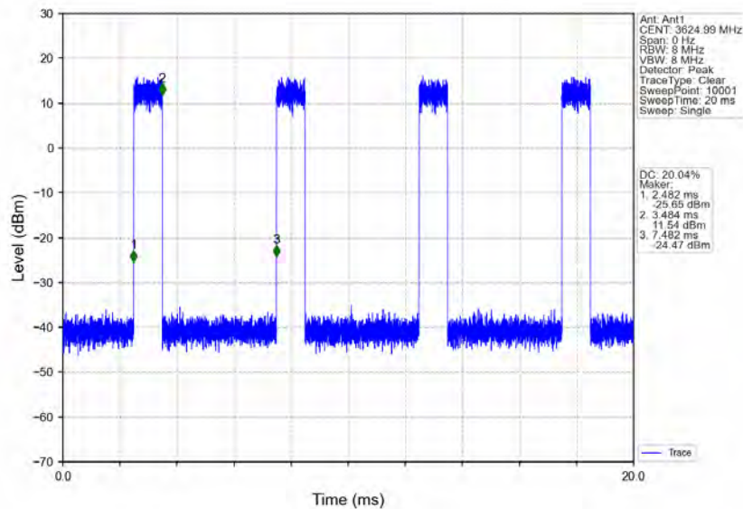
n78d_30kHz_MIMO_NTNV_80MHz_CP-OFDM 64 QAM_3624.99MHz_Inner_Full
