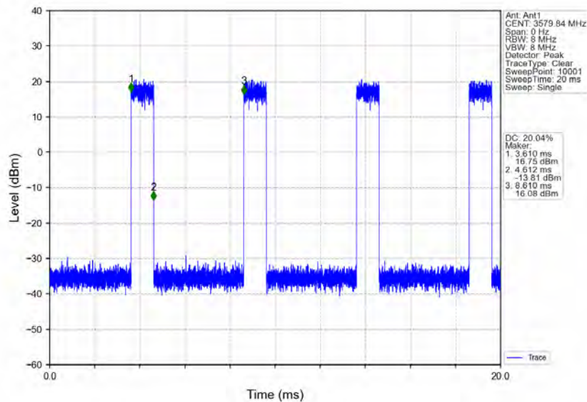
n78d_30kHz_MIMO_NTNV_60MHz_CP-OFDM_QPSK_3580.02MHz_Inner_Full
