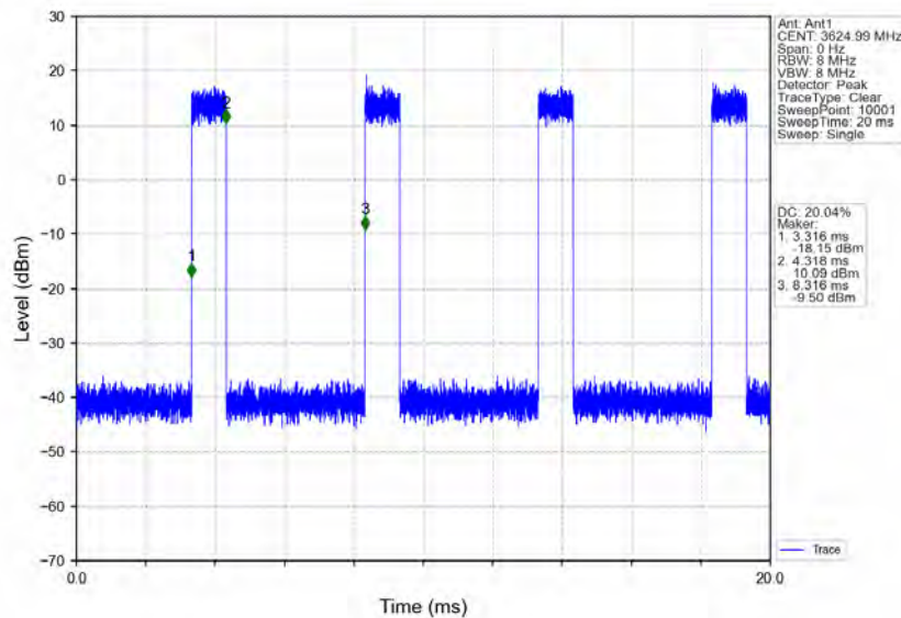
n78d_30kHz_MIMO_NTNV_60MHz_CP-OFDM 64 QAM_3624.99MHz_Inner_Full
