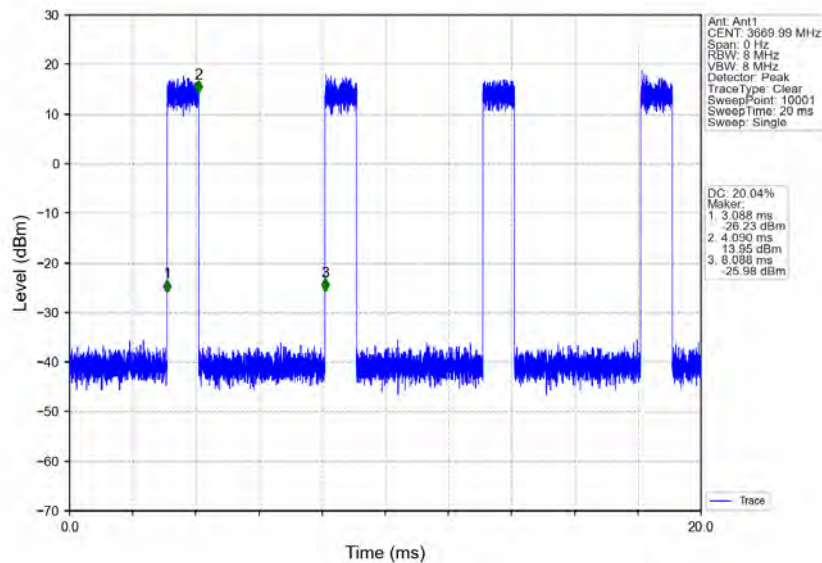
n78d_30kHz_MIMO_NTNV_60MHz_CP-OFDM 64 QAM_3669.99MHz_Inner_Full
