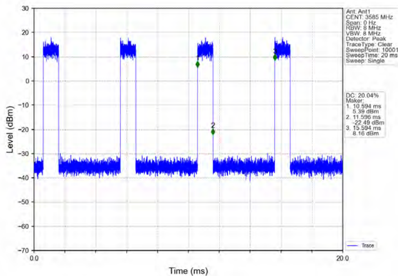
n78d_30kHz_MIMO_NTNV_70MHz_CP-OFDM_64_QAM_3585MHz_Inner_Full
