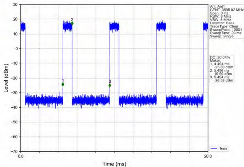
n78d_30kHz_MIMO_NTNV_90MHz_CP-OFDM_QPSK_3595.02MHz_Inner_Full
