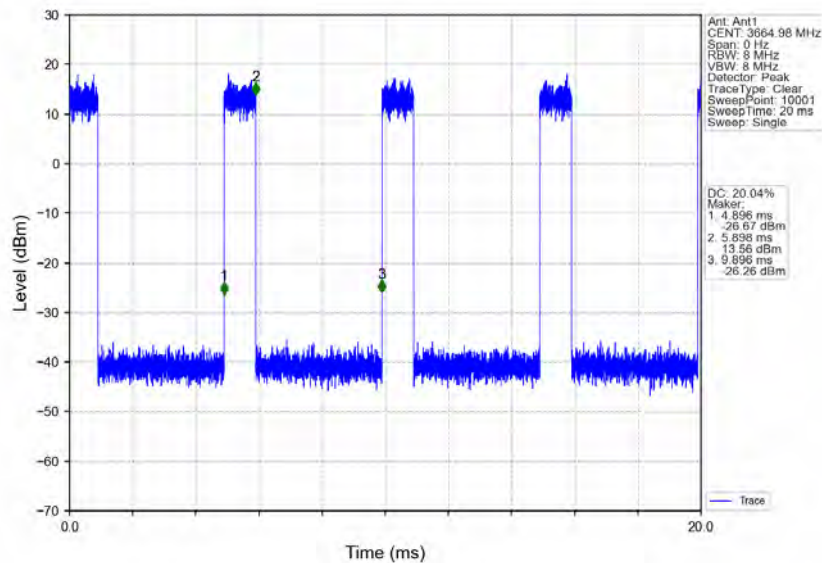
n78d_30kHz_MIMO_NTNV_70MHz_CP-OFDM_256_QAM_3664.98MHz_Inner_Full
