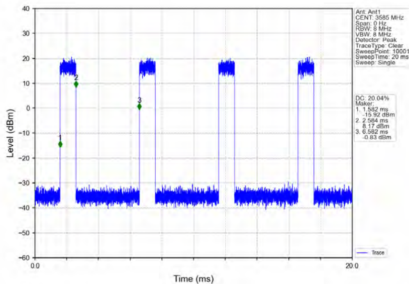
n78d_30kHz_MIMO_NTNV_70MHz_CP-OFDM_QPSK_3585MHz_Inner_Full
