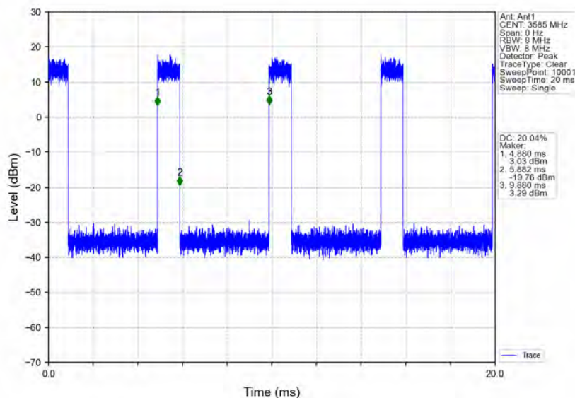
n78d_30kHz_MIMO_NTNV_70MHz_CP-OFDM_16_QAM_3585MHz_Inner_Full
