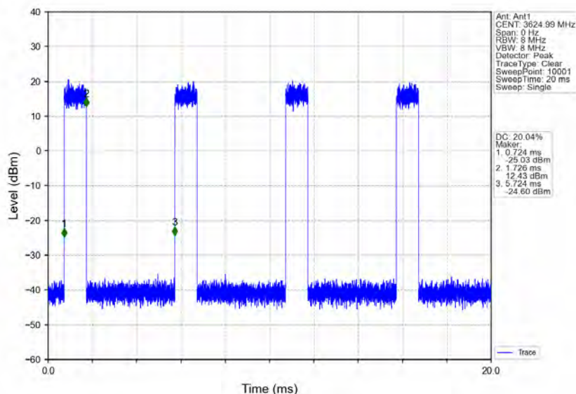
n78d_30kHz_MIMO_NTNV_70MHz_CP-OFDM 64 QAM_3624.99MHz_Inner_Full
