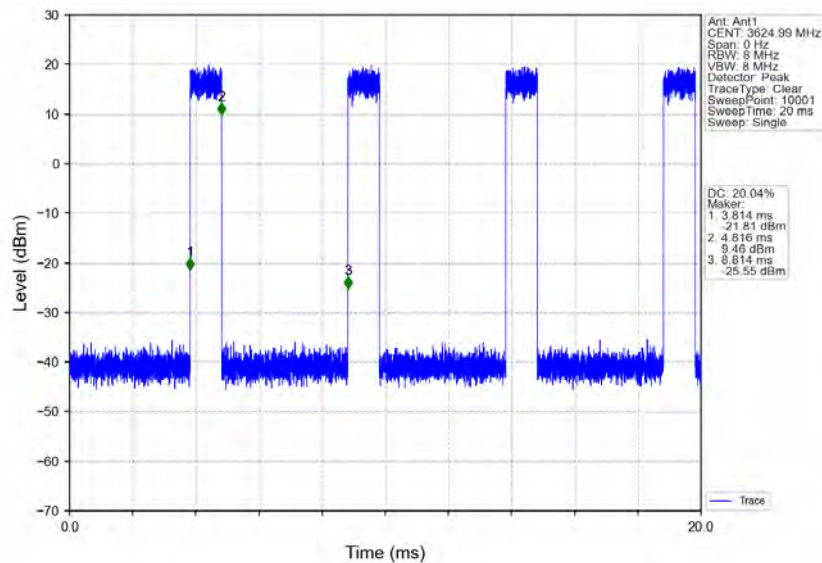
n78d_30kHz_MIMO_NTNV_70MHz_CP-OFDM_16_QAM_3624.99MHz_Inner_Full
