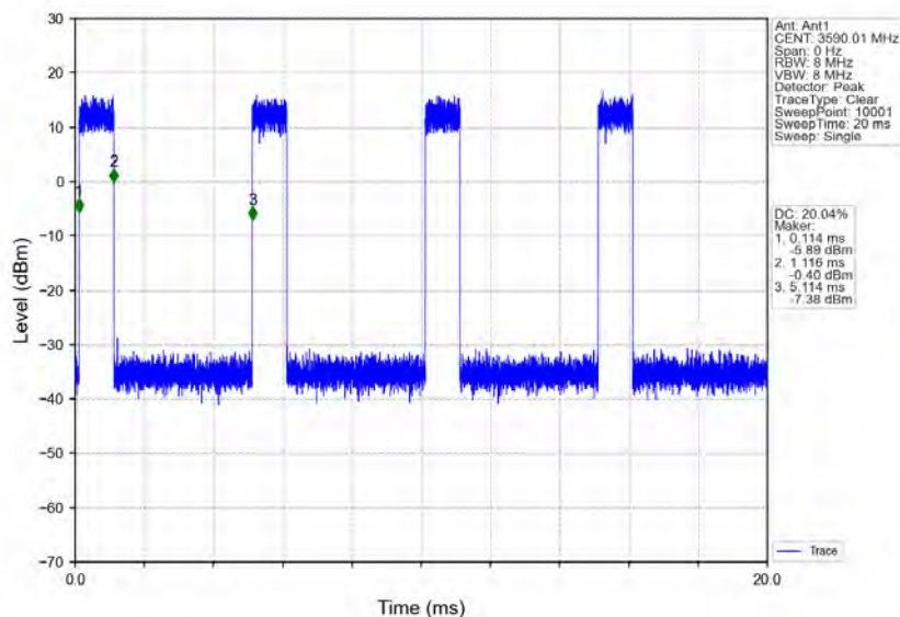
n78d_30kHz_MIMO_NTNV_80MHz_CP-OFDM 64 QAM_3590.01MHz_Inner_Full
