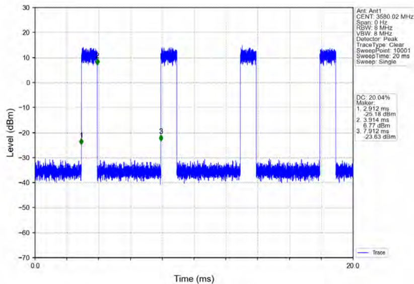
n78d_30kHz_MIMO_NTNV_60MHz_CP-OFDM_256_QAM_3580.02MHz_Inner_Full
