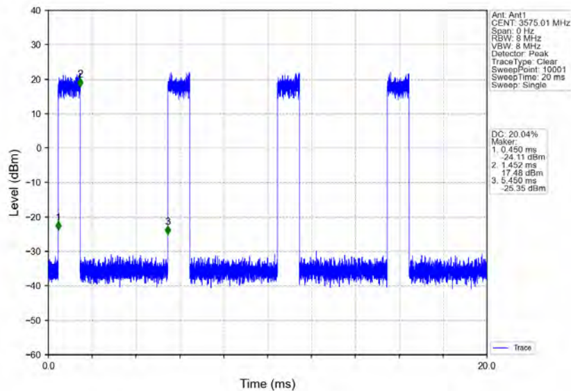
n78d_30kHz_MIMO_NTNV_50MHz_CP-OFDM_QPSK_3575.01MHz_Inner_Full
