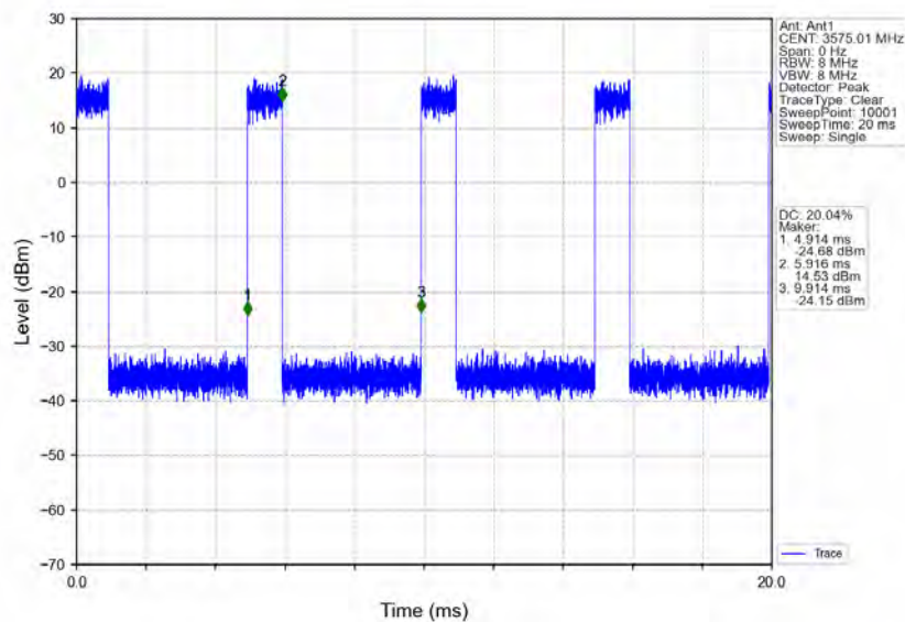
n78d_30kHz_MIMO_NTNV_50MHz_CP-OFDM_16_QAM_3575.01MHz_Inner_Full
