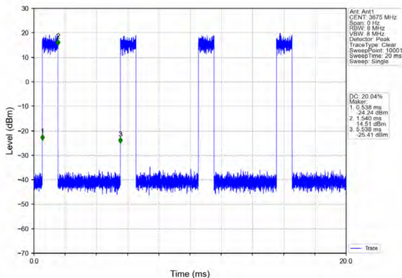
n78d_30kHz_MIMO_NTNV_50MHz_CP-OFDM_16_QAM_3675MHz_Inner_Full
