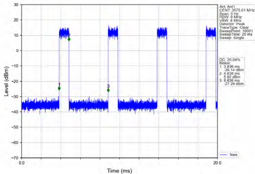
n78d_30kHz_MIMO_NTNV_50MHz_CP-OFDM_256_QAM_3575.01MHz_Inner_Full
