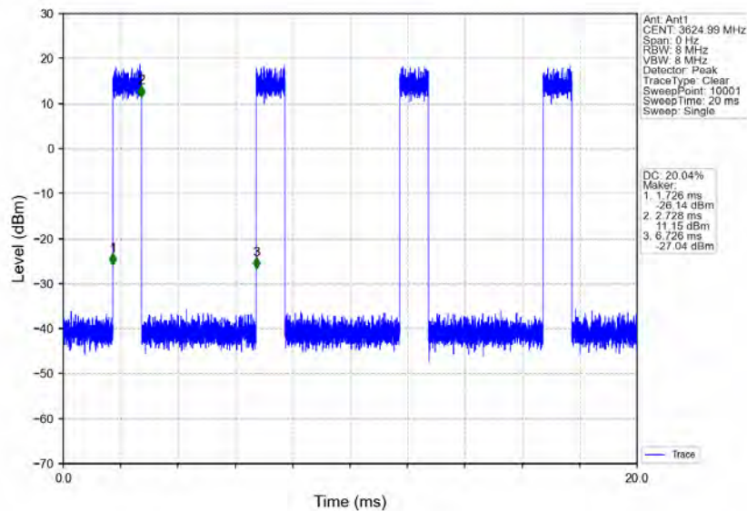
n78d_30kHz_MIMO_NTNV_50MHz_CP-OFDM_256_QAM_3624.99MHz_Inner_Full
