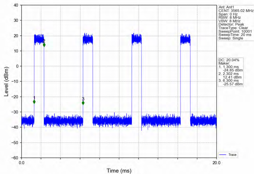
n78d_30kHz_MIMO_NTNV_30MHz_CP-OFDM_QPSK_3565.02MHz_Inner_Full
