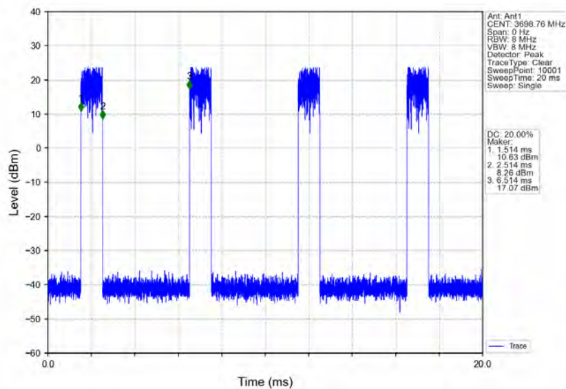
n78d_30kHz_MIMO_NTNV_50MHz_CP-OFDM 64 QAM_3675MHz_Edge_1RB_Right
