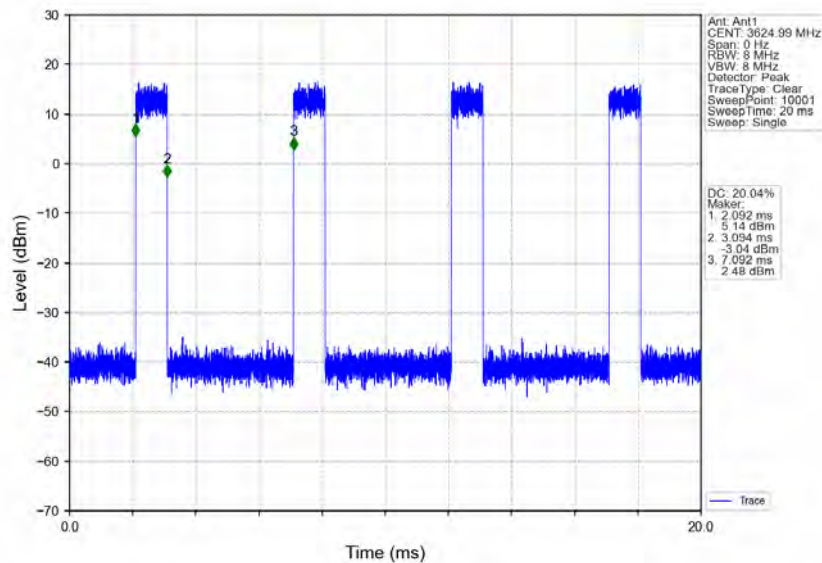
n78d_30kHz_MIMO_NTNV_40MHz_CP-OFDM_256_QAM_3624.99MHz_Inner_Full
