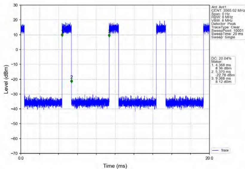
n78d_30kHz_MIMO_NTNV_30MHz_CP-OFDM_256_QAM_3565.02MHz_Inner_Full
