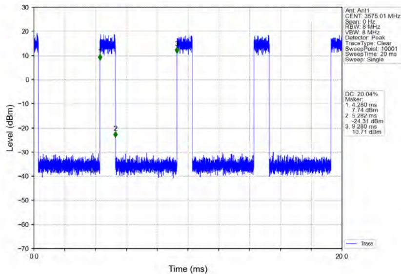
n78d_30kHz_MIMO_NTNV_50MHz_CP-OFDM 64 QAM_3575.01MHz_Inner_Full
