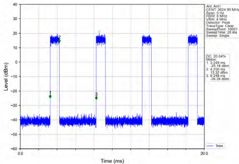
n78d_30kHz_MIMO_NTNV_40MHz_CP-OFDM_64_QAM_3624.99MHz_Inner_Full
