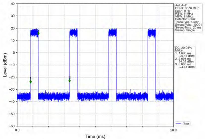
n78d_30kHz_MIMO_NTNV_40MHz_CP-OFDM_QPSK_3570MHz_Inner_Full
