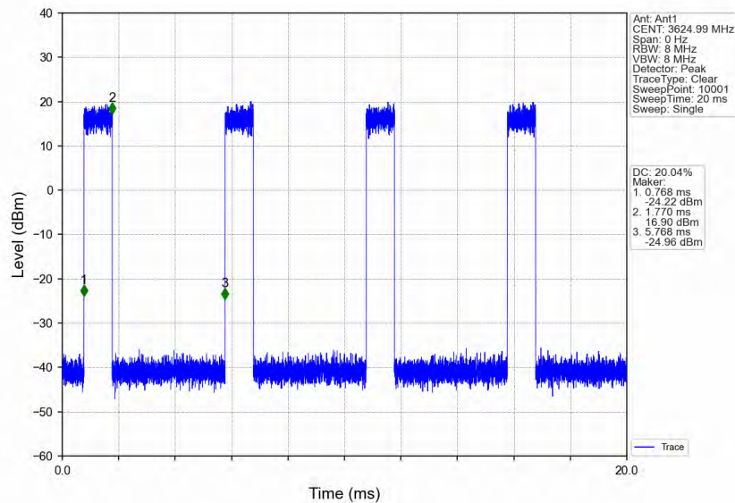
n78d_30kHz_MIMO_NTNV_40MHz_CP-OFDM_16_QAM_3624.99MHz_Inner_Full
