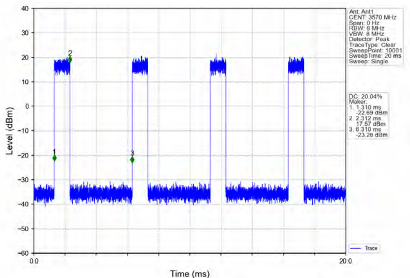
n78d_30kHz_MIMO_NTNV_40MHz_CP-OFDM_16_QAM_3570MHz_Inner_Full
