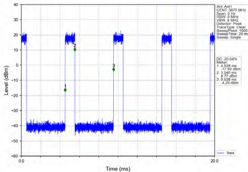
n78d_30kHz_MIMO_NTNV_50MHz_CP-OFDM_64_QAM_3675MHz_Inner_Full
