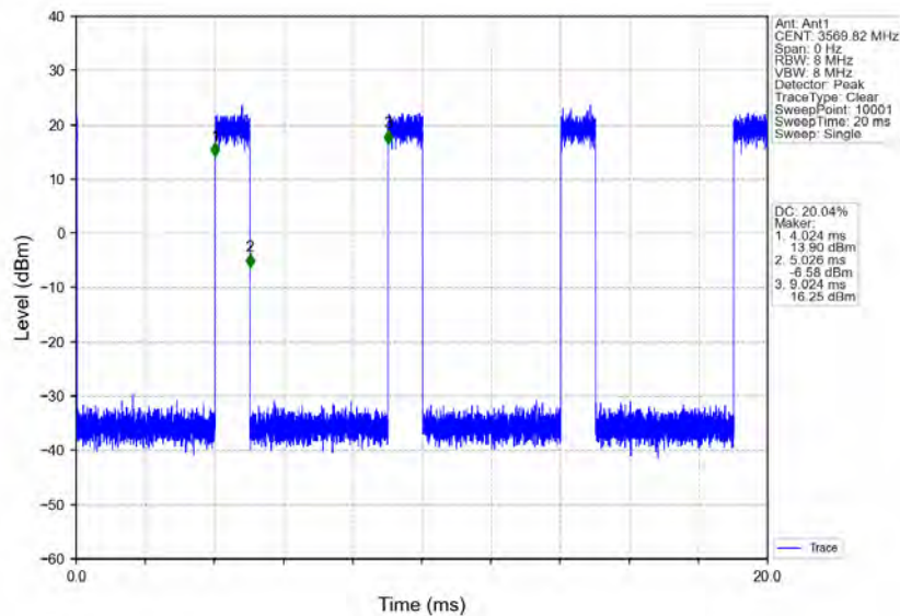
n78d_30kHz_MIMO_NTNV_40MHz_CP-OFDM_QPSK_3570MHz_Inner_Full
