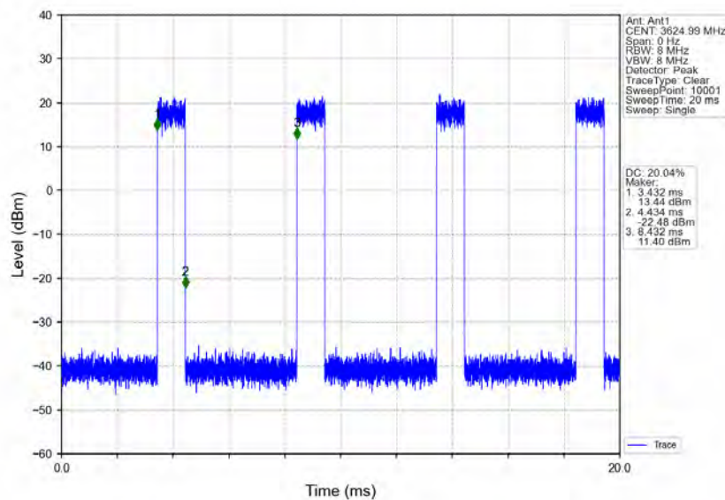
n78d_30kHz_MIMO_NTNV_50MHz_CP-OFDM_16_QAM_3624.99MHz_Inner_Full
