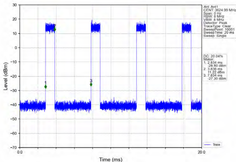
n78d_30kHz_MIMO_NTNV_30MHz_CP-OFDM_256_QAM_3624.99MHz_Inner_Full
