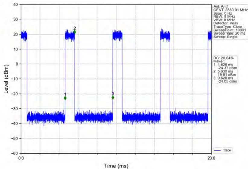
n78d_30kHz_MIMO_NTNV_20MHz_CP-OFDM_16_QAM_3560.01MHz_Inner_Full
