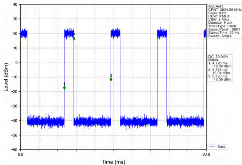
n78d_30kHz_MIMO_NTNV_15MHz_CP-OFDM_64_QAM_3624.99MHz_Inner_Full
