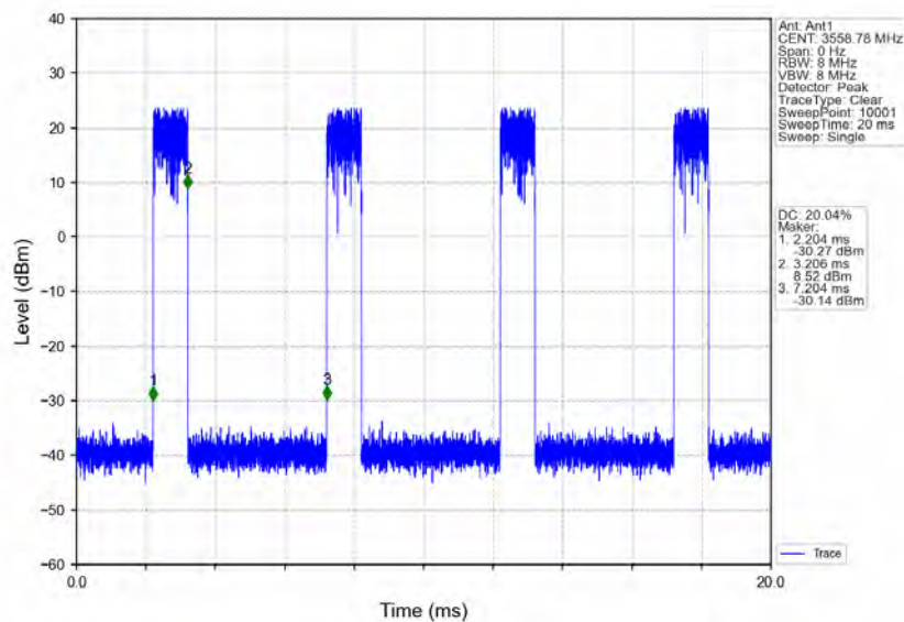
n78d_30kHz_MIMO_NTNV_10MHz_CP-OFDM_64_QAM_3555MHz_Inner_1RB_Right
