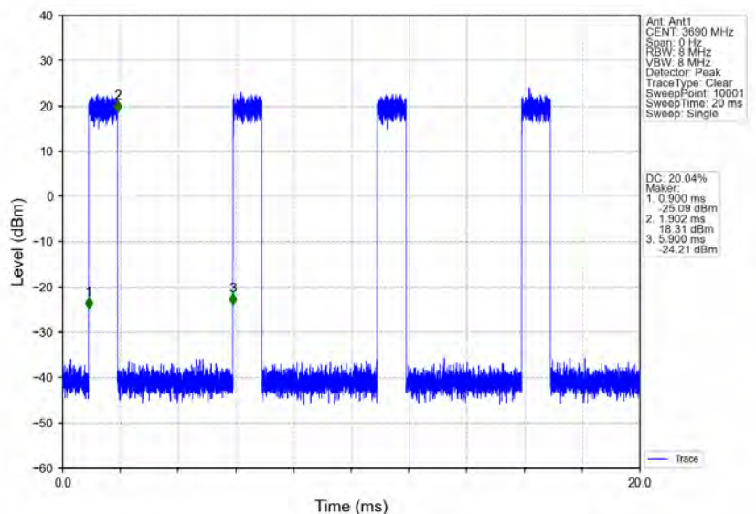
n78d_30kHz_MIMO_NTNV_20MHz_CP-OFDM_QPSK_3690MHz_Inner_Full
