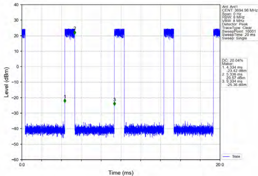
n78d_30kHz_MIMO_NTNV_10MHz_CP-OFDM_64_QAM_3694.98MHz_Inner_Full
