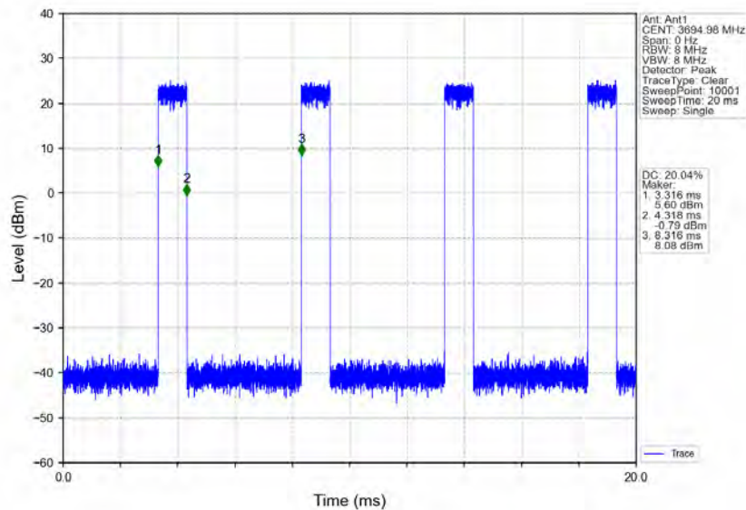
n78d_30kHz_MIMO_NTNV_10MHz_CP-OFDM_QPSK_3694.98MHz_Inner_Full
