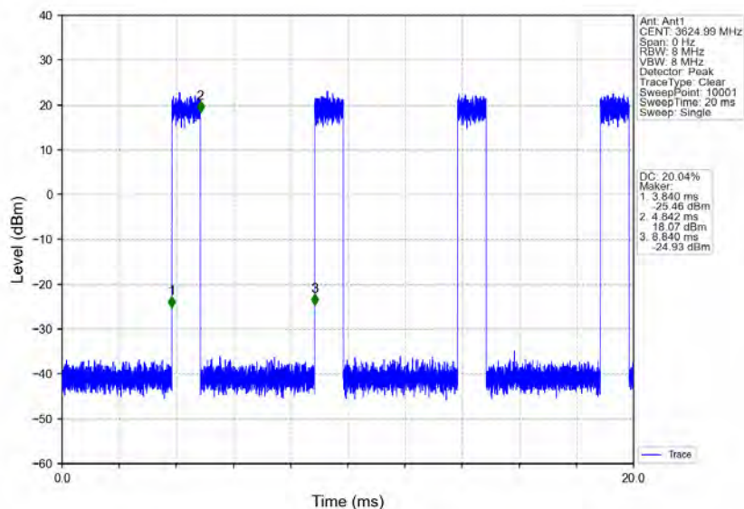
n78d_30kHz_MIMO_NTNV_20MHz_CP-OFDM_QPSK_3624.99MHz_Inner_Full
