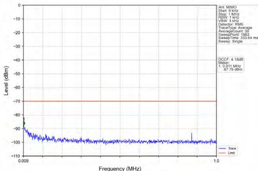
n48_30kHz_MIMO_NTNV_40MHz_CP-OFDM_QPSK_3570MHz_Inner_1RB_Left
