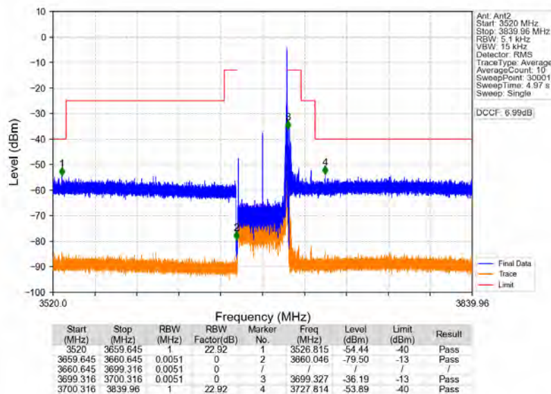
n48_30kHz_MIMO_NTNV_40MHz_CP-OFDM_QPSK_3679.98MHz_Inner_1RB_Right
