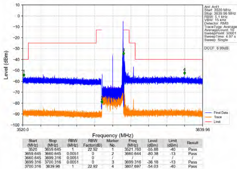
n48_30kHz_MIMO_NTNV_40MHz_CP-OFDM_QPSK_3679.98MHz_Inner_1RB_Right
