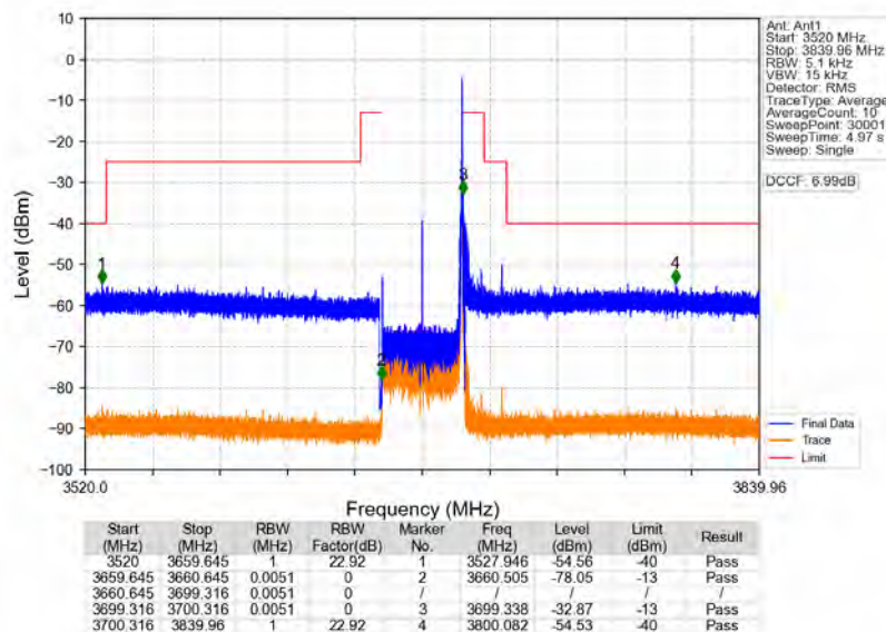
n48_30kHz_MIMO_NTNV_40MHz_CP-OFDM_QPSK_3679.98MHz_Edge_1RB_Right
