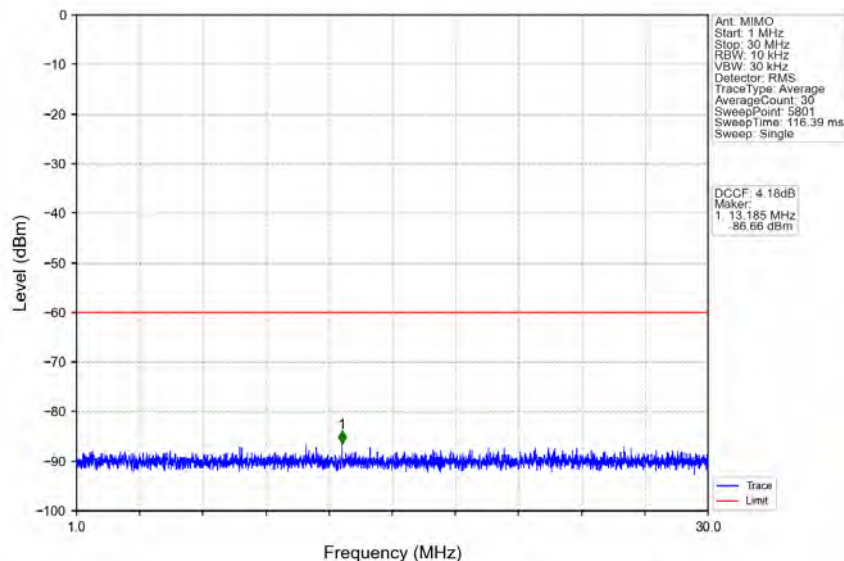
n48_30kHz_MIMO_NTNV_40MHz_CP-OFDM_QPSK_3570MHz_Inner_1RB_Left
