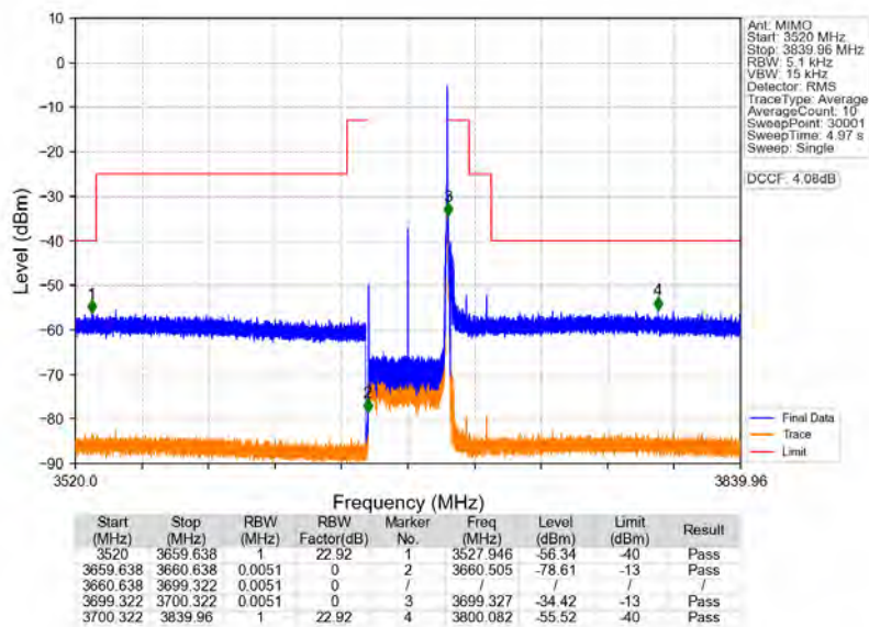
n48_30kHz_MIMO_NTNV_40MHz_CP-OFDM_QPSK_3679.98MHz_Edge_1RB_Right
