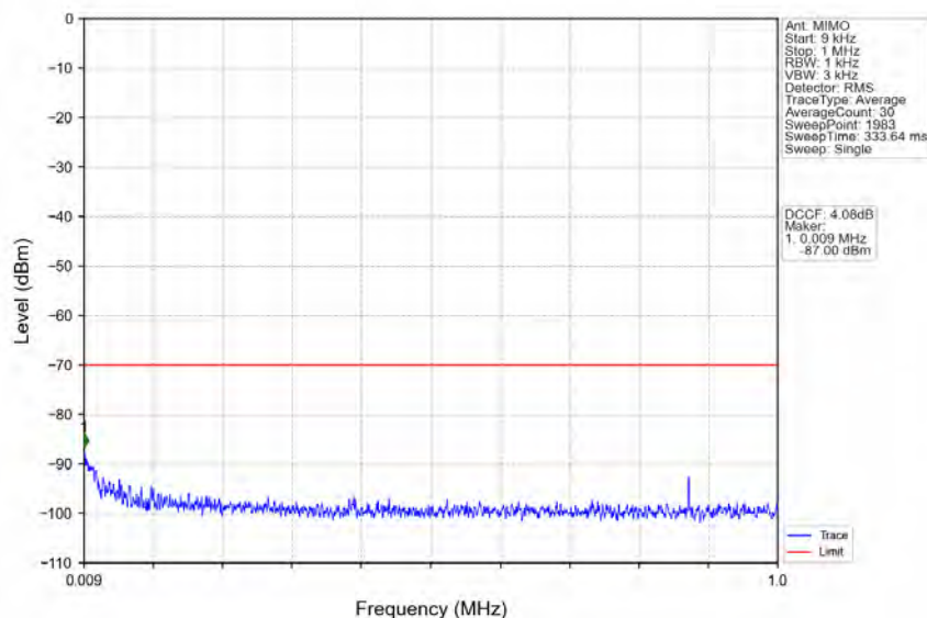
n48_30kHz_MIMO_NTNV_40MHz_CP-OFDM_QPSK_3679.98MHz_Edge_1RB_Right
