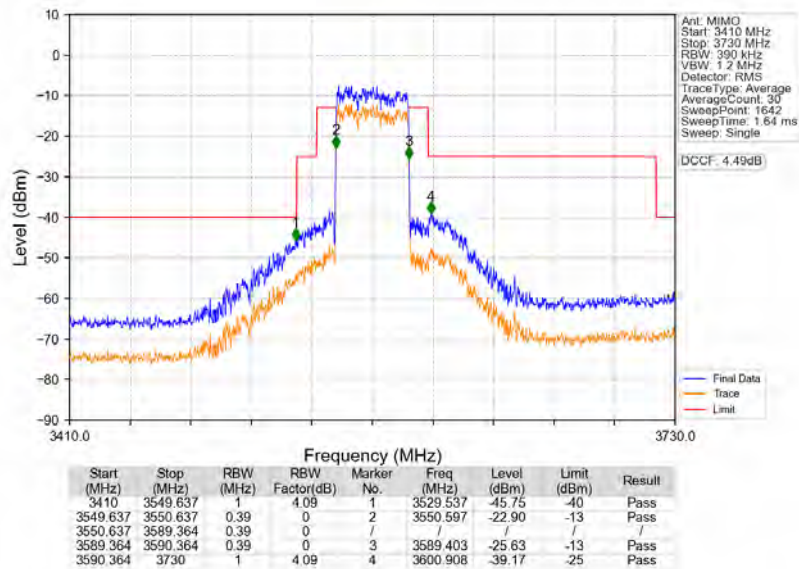
n48_30kHz_MIMO_NTNV_40MHz_CP-OFDM_QPSK_3570MHz_Outer_Full
