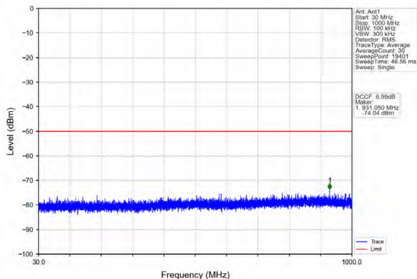
n48_30kHz_MIMO_NTNV_20MHz_CP-OFDM_QPSK_3560.01MHz_Outer_Full
