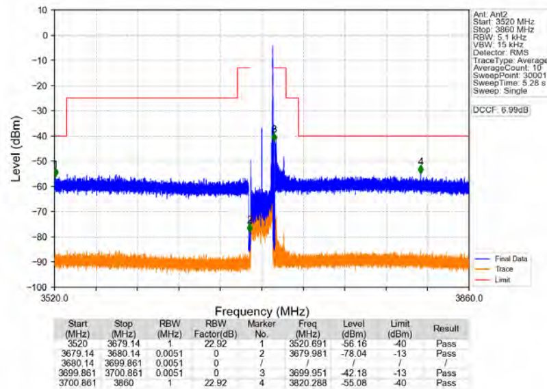
n48_30kHz_MIMO_NTNV_20MHz_CP-OFDM_QPSK_3690MHz_Edge_1RB_Right
