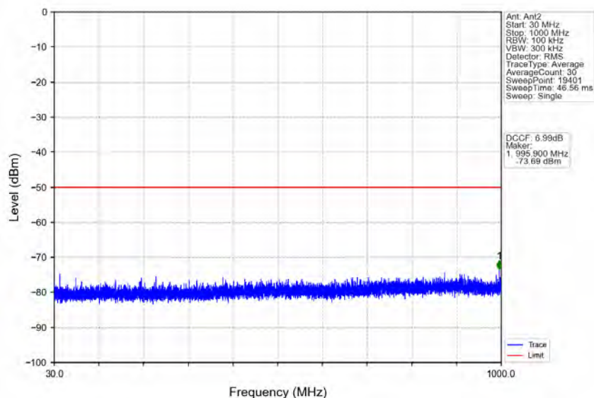
n48_30kHz_MIMO_NTNV_40MHz_CP-OFDM QPSK_3570MHz_Edge_1RB_Left
