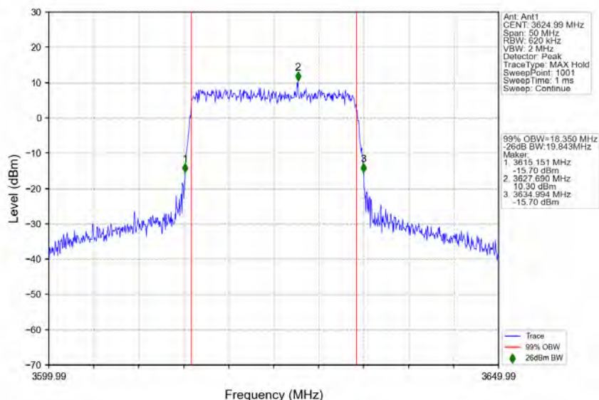
n48_30kHz_MIMO_NTNV_20MHz_CP-OFDM_16_QAM_3624.99MHz_Outer_Full
