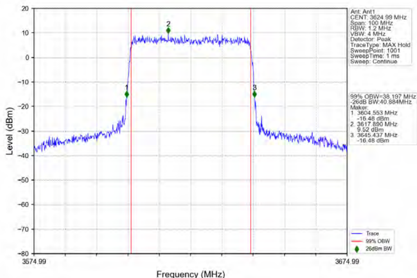
n48_30kHz_MIMO_NTNV_40MHz_CP-OFDM_16 QAM_3624.99MHz_Outer_Full
