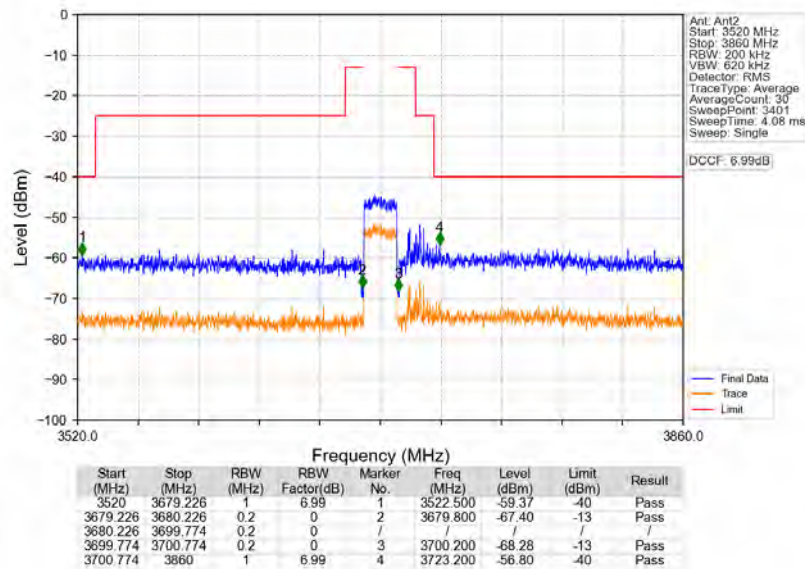
n48_30kHz_MIMO_NTNV_20MHz_CP-OFDM_QPSK_3690MHz_Outer_Full
