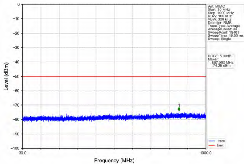
n48_30kHz_MIMO_NTNV_20MHz_CP-OFDM_QPSK_3690MHz_Inner_1RB_Right
