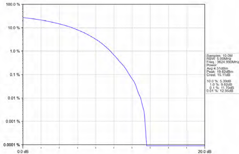
n48_30kHz_MIMO_NTNV_10MHz_CP-OFDM_256_QAM_3624.99MHz_Outer_Full
