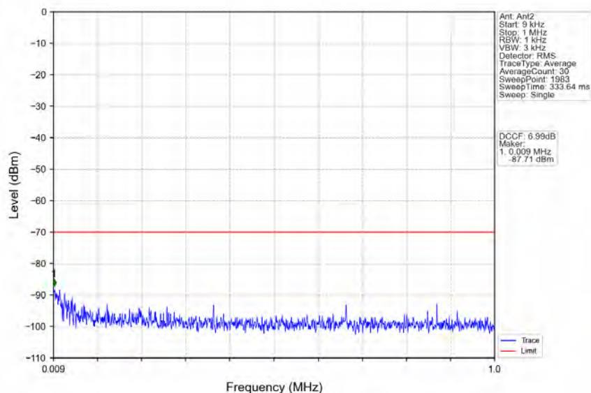
n48_30kHz_MIMO_NTNV_10MHz_CP-OFDM QPSK_3555MHz_Edge_1RB_Left
