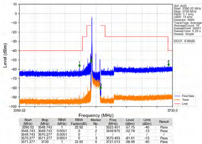
n48_30kHz_MIMO_NTNV_20MHz_CP-OFDM_QPSK_3560.01MHz_Edge_1RB_Left
