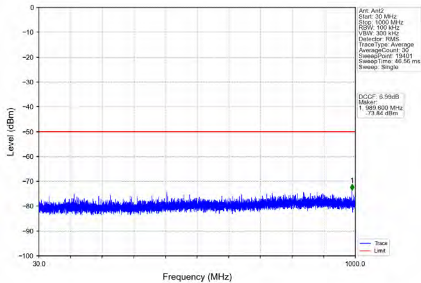
n48_30kHz_MIMO_NTNV_10MHz_CP-OFDM QPSK_3555MHz_Inner_1RB_Left
