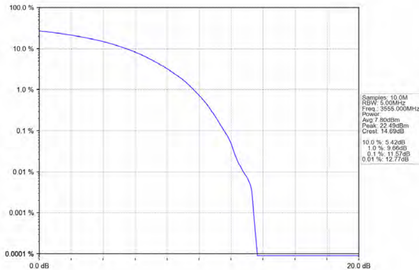
n48_30kHz_MIMO_NTNV_10MHz_CP-OFDM_16_QAM_3555MHz_Outer_Full
