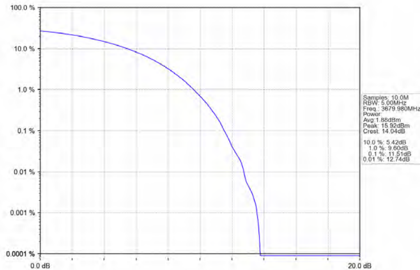
n48_30kHz_MIMO_NTNV_40MHz_CP-OFDM_QPSK_3679.98MHz_Outer_Full
