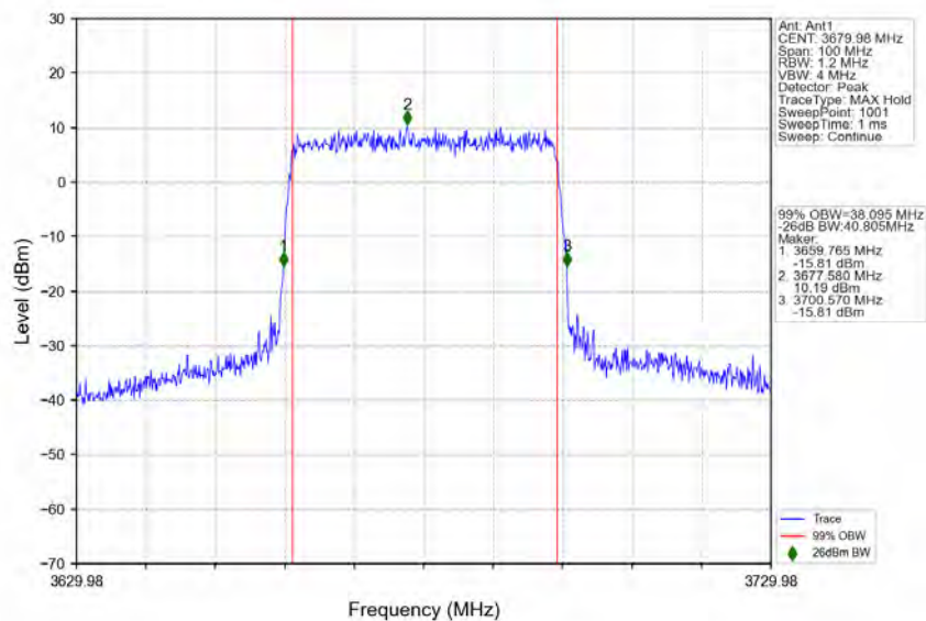
n48_30kHz_MIMO_NTNV_40MHz_CP-OFDM QPSK_3679.98MHz_Outer_Full
