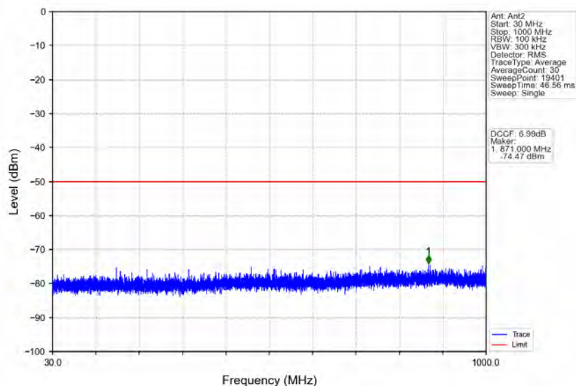
n48_30kHz_MIMO_NTNV_10MHz_CP-OFDM_QPSK_3694.98MHz_Outer_Full
