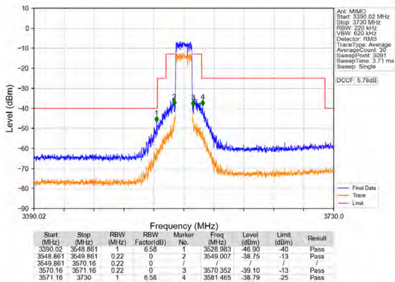
n48_30kHz_MIMO_NTNV_20MHz_CP-OFDM_QPSK_3560.01MHz_Outer_Full
