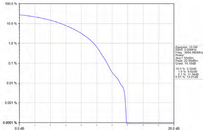
n48_30kHz_MIMO_NTNV_10MHz_CP-OFDM_64_QAM_3694.98MHz_Outer_Full
