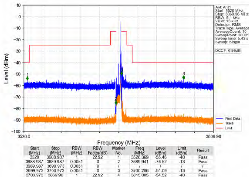
n48_30kHz_MIMO_NTNV_10MHz_CP-OFDM_QPSK_3694.98MHz_Edge_1RB_Right
