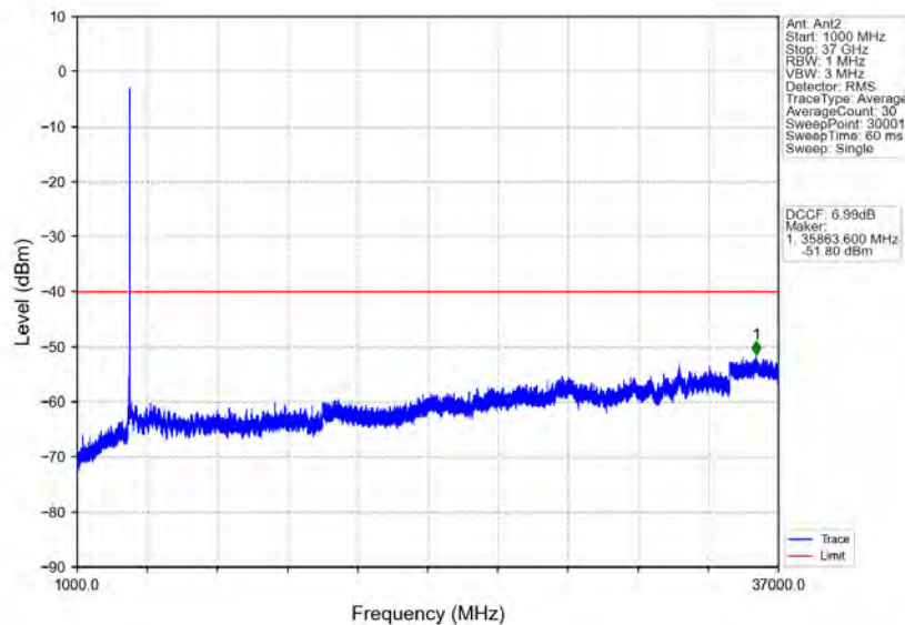
n48_30kHz_MIMO_NTNV_20MHz_CP-OFDM_QPSK_3690MHz_Outer_Full
