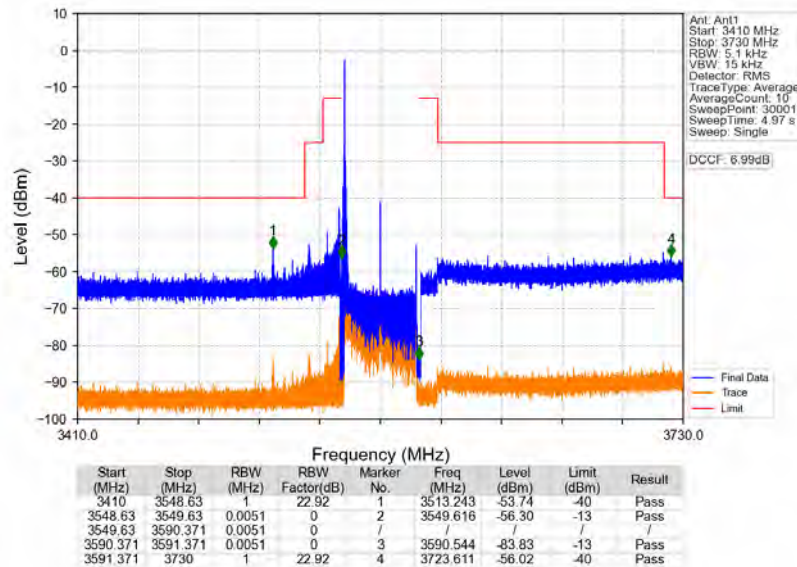
n48_30kHz_MIMO_NTNV_40MHz_CP-OFDM_QPSK_3570MHz_Edge_1RB_Left
