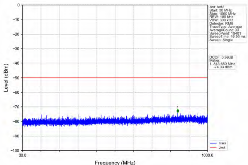
n48_30kHz_MIMO_NTNV_10MHz_CP-OFDM_QPSK_3694.98MHz_Edge_1RB_Right
