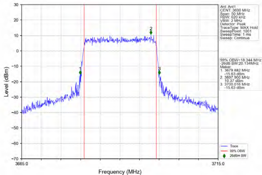
n48_30kHz_MIMO_NTNV_20MHz_CP-OFDM_QPSK_3690MHz_Outer_Full
