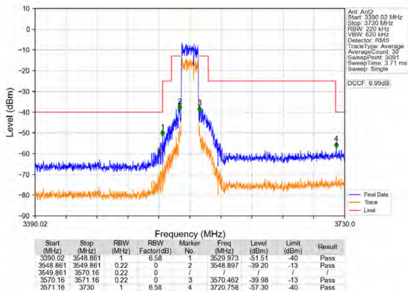
n48_30kHz_MIMO_NTNV_20MHz_CP-OFDM_QPSK_3560.01MHz_Outer_Full
