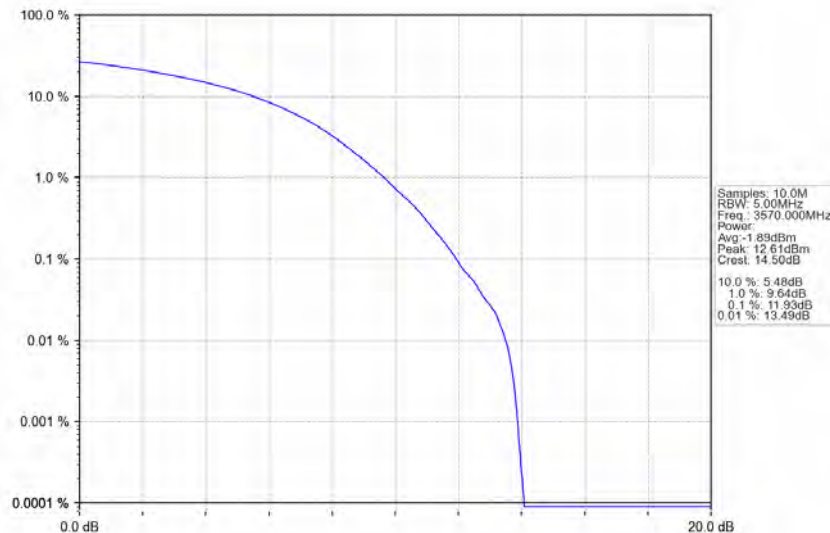
n48_30kHz_MIMO_NTNV_40MHz_CP-OFDM_256_QAM_3570MHz_Outer_Full
