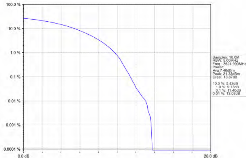
n48_30kHz_MIMO_NTNV_10MHz_CP-OFDM_64_QAM_3624.99MHz_Outer_Full
