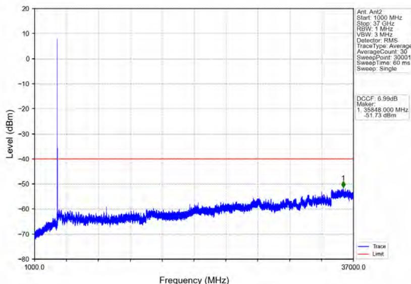
n48_30kHz_MIMO_NTNV_40MHz_CP-OFDM QPSK_3570MHz_Edge_1RB_Left
