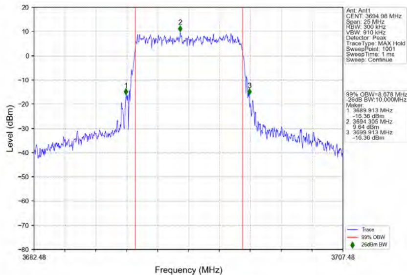
n48_30kHz_MIMO_NTNV_10MHz_CP-OFDM_QPSK_3694.98MHz_Outer_Full
