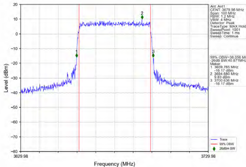
n48_30kHz_MIMO_NTNV_40MHz_CP-OFDM_64_QAM_3679.98MHz_Outer_Full
