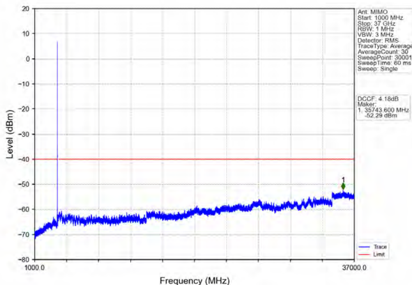
n48_30kHz_MIMO_NTNV_10MHz_CP-OFDM_QPSK_3555MHz_Outer_Full
