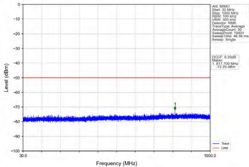
n48_30kHz_MIMO_NTNV_20MHz_CP-OFDM_QPSK_3690MHz_Edge_1RB_Right
