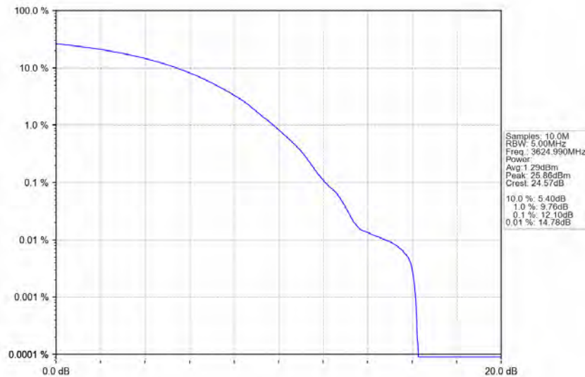
n48_30kHz_MIMO_NTNV_20MHz_CP-OFDM_256_QAM_3624.99MHz_Outer_Full
