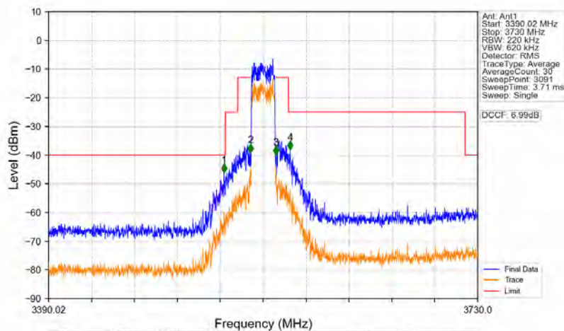
n48_30kHz_MIMO_NTNV_20MHz_CP-OFDM_QPSK_3560.01MHz_Outer_Full
