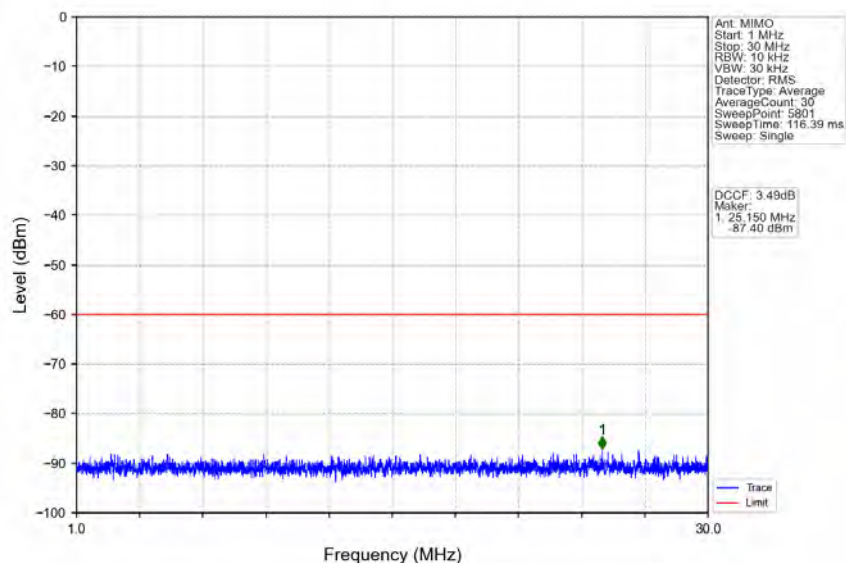
n48_30kHz_MIMO_NTNV_20MHz_CP-OFDM_QPSK_3560.01MHz_Edge_1RB_Left
