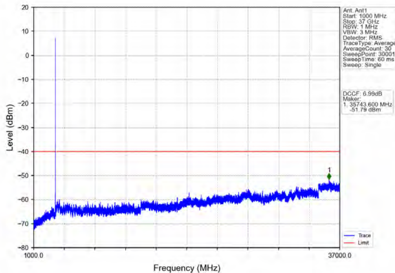
n48_30kHz_MIMO_NTNV_10MHz_CP-OFDM_QPSK_3555MHz_Edge_1RB_Left
