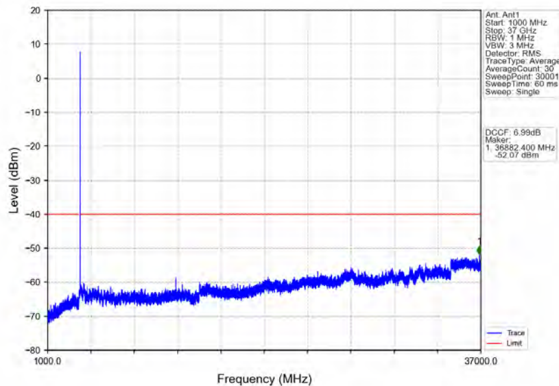
n48_30kHz_MIMO_NTNV_10MHz_CP-OFDM_QPSK_3694.98MHz_Edge_1RB_Right
