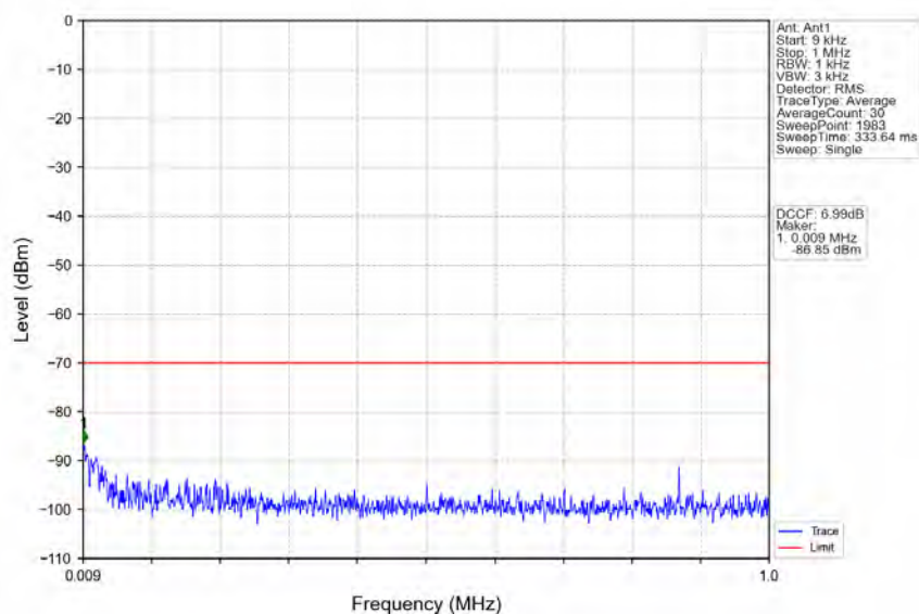
n48_30kHz_MIMO_NTNV_10MHz_CP-OFDM_QPSK_3555MHz_Edge_1RB_Left
