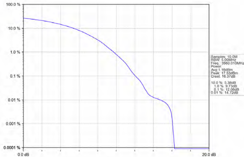
n48_30kHz_MIMO_NTNV_20MHz_CP-OFDM_256_QAM_3560.01MHz_Outer_Full
