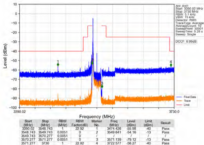
n48_30kHz_MIMO_NTNV_20MHz_CP-OFDM_QPSK_3560.01MHz_Inner_1RB_Left
