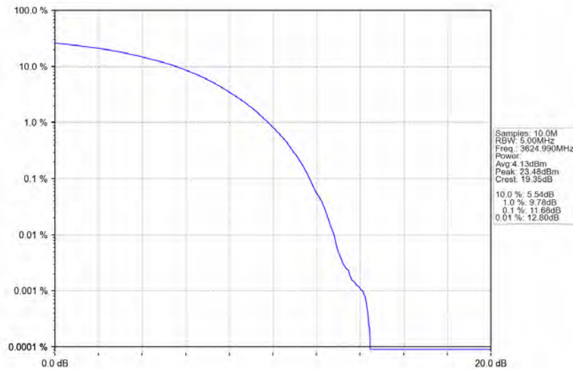
n48_30kHz_MIMO_NTNV_20MHz_CP-OFDM_64_QAM_3624.99MHz_Outer_Full
