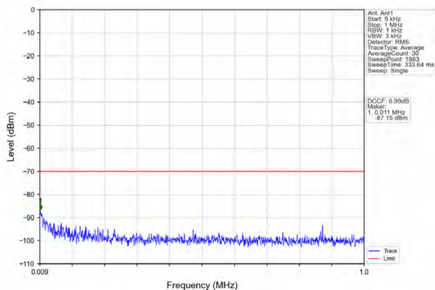
n48_30kHz_MIMO_NTNV_40MHz_CP-OFDM_QPSK_3570MHz_Edge_1RB_Left
