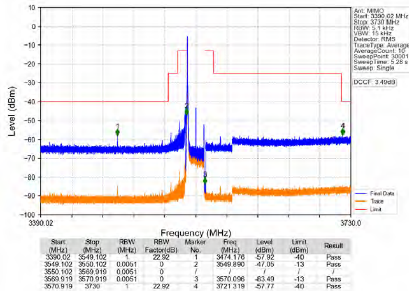
n48_30kHz_MIMO_NTNV_20MHz_CP-OFDM_QPSK_3560.01MHz_Edge_1RB_Left
