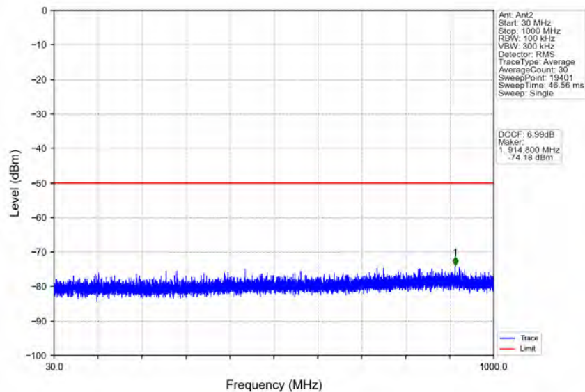
n48_30kHz_MIMO_NTNV_10MHz_CP-OFDM QPSK_3555MHz_Edge_1RB_Left
