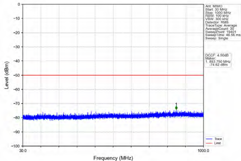
n48_30kHz_MIMO_NTNV_10MHz_CP-OFDM QPSK_3555MHz_Inner_1RB_Left
