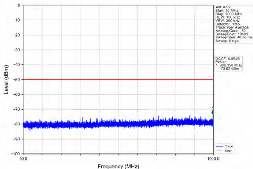
n48_30kHz_MIMO_NTNV_20MHz_CP-OFDM_QPSK_3560.01MHz_Inner_1RB_Left
