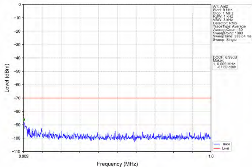
n48_30kHz_MIMO_NTNV_20MHz_CP-OFDM_QPSK_3690MHz_Edge_1RB_Right
