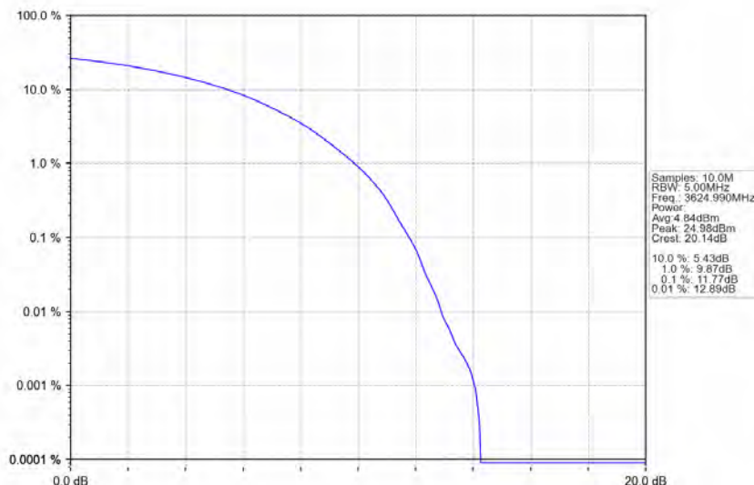
n48_30kHz_MIMO_NTNV_20MHz_CP-OFDM_QPSK_3624.99MHz_Outer_Full
