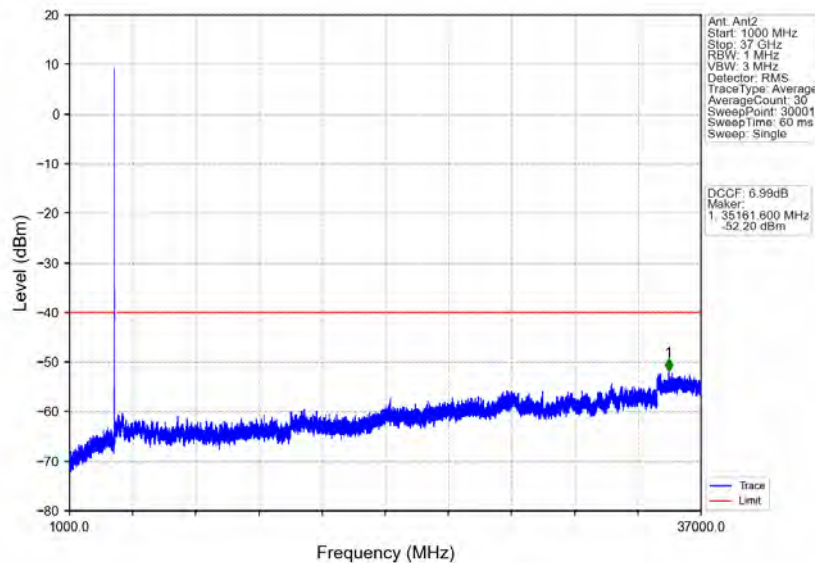
n48_30kHz_MIMO_NTNV_10MHz_CP-OFDM QPSK_3555MHz_Inner_1RB_Left
