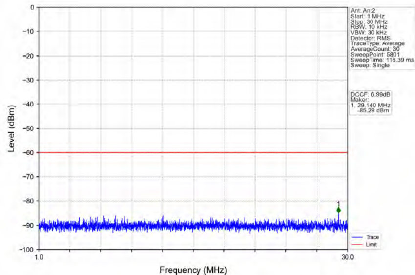
n48_30kHz_MIMO_NTNV_20MHz_CP-OFDM_QPSK_3560.01MHz_Outer_Full
