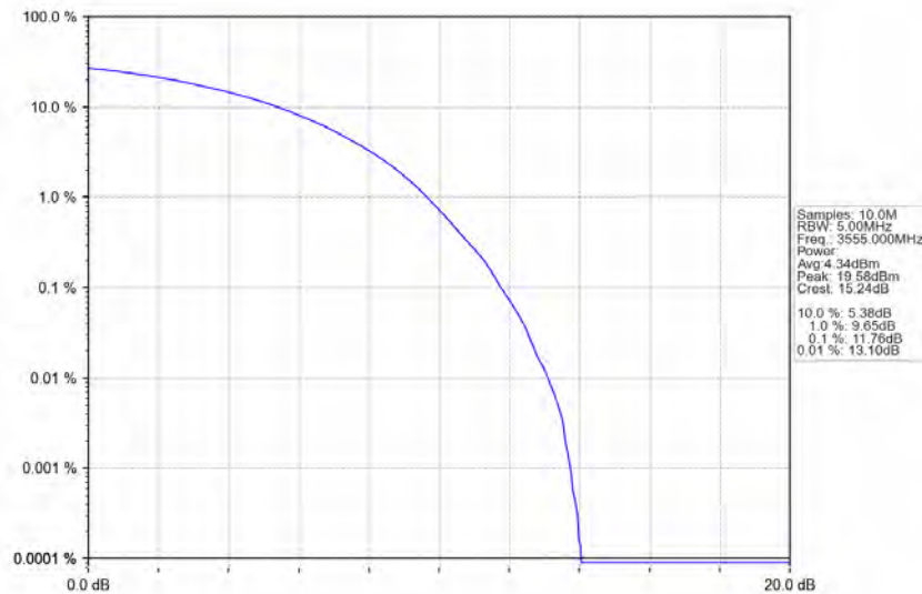
n48_30kHz_MIMO_NTNV_10MHz_CP-OFDM_256_QAM_3555MHz_Outer_Full
