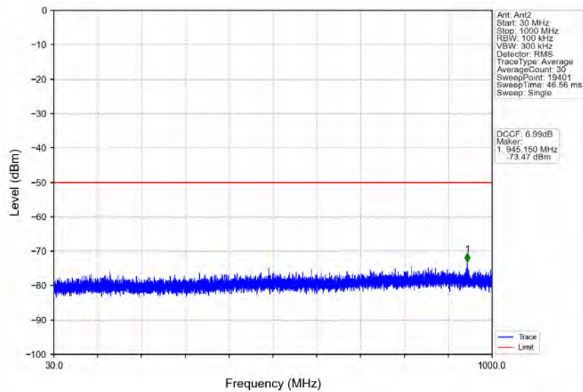
n48_30kHz_MIMO_NTNV_20MHz_CP-OFDM_QPSK_3690MHz_Outer_Full
