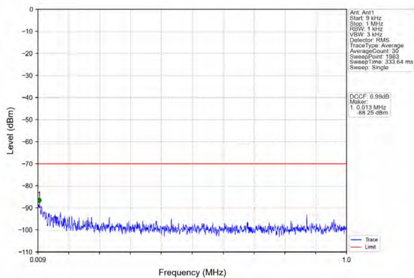
n48_30kHz_MIMO_NTNV_20MHz_CP-OFDM_QPSK_3560.01MHz_Edge_1RB_Left
