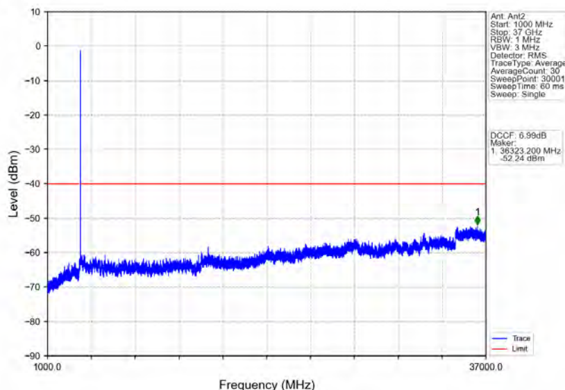
n48_30kHz_MIMO_NTNV_10MHz_CP-OFDM_QPSK_3694.98MHz_Outer_Full
