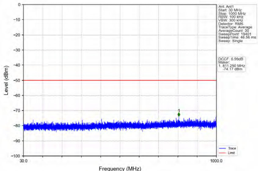
n48_30kHz_MIMO_NTNV_20MHz_CP-OFDM_QPSK_3560.01MHz_Edge_1RB_Left
