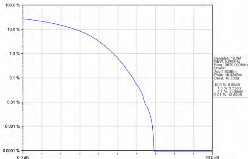
n48_30kHz_MIMO_NTNV_40MHz_CP-OFDM_16_QAM_3570MHz_Outer_Full
