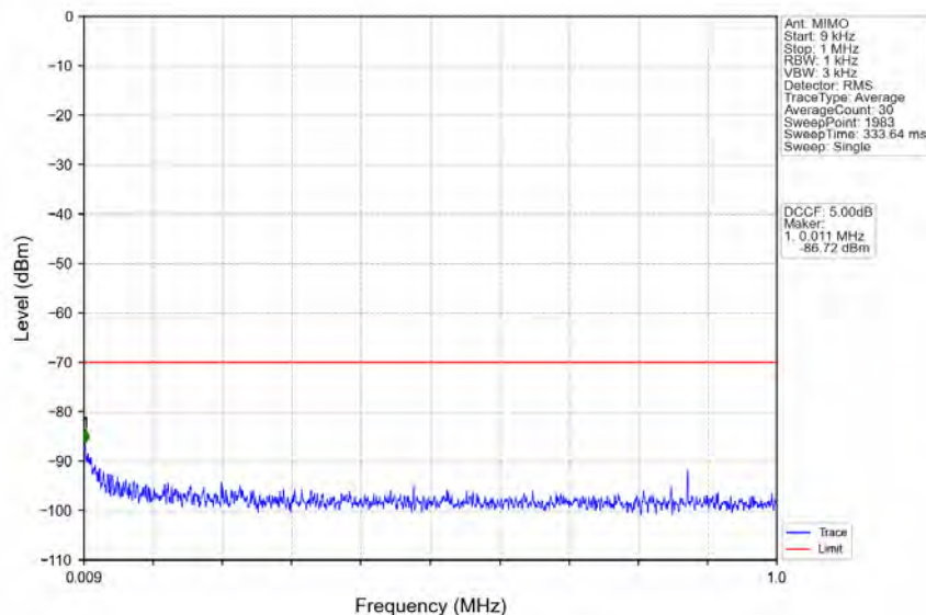
n48_30kHz_MIMO_NTNV_20MHz_CP-OFDM_QPSK_3690MHz_Inner_1RB_Right
