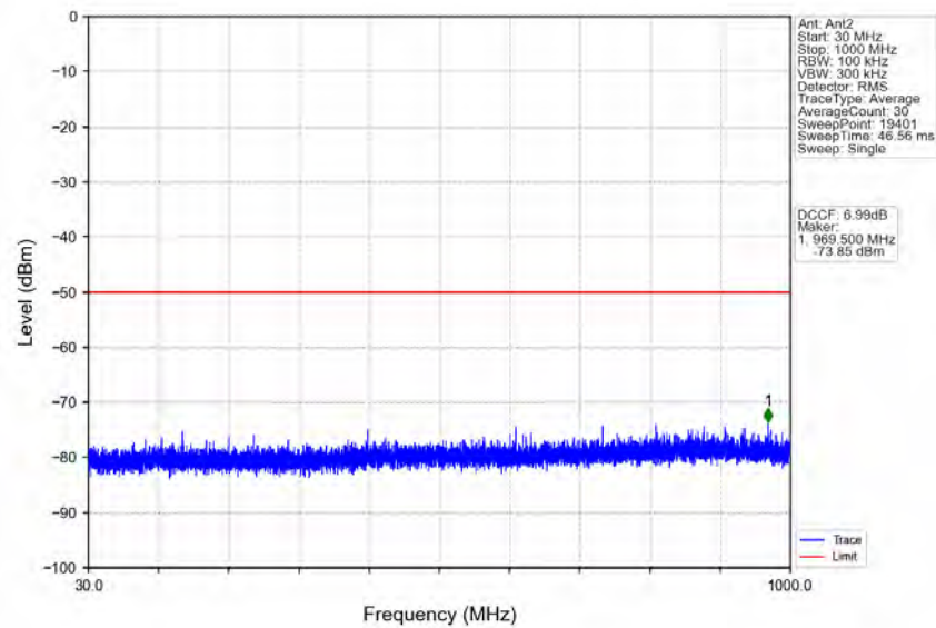
n48_30kHz_MIMO_NTNV_20MHz_CP-OFDM_QPSK_3560.01MHz_Edge_1RB_Left
