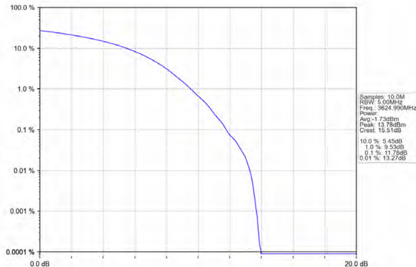
n48_30kHz_MIMO_NTNV_40MHz_CP-OFDM_256_QAM_3624.99MHz_Outer_Full
