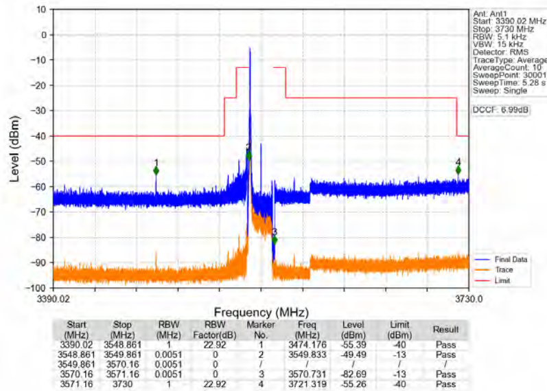
n48_30kHz_MIMO_NTNV_20MHz_CP-OFDM_QPSK_3560.01MHz_Edge_1RB_Left
