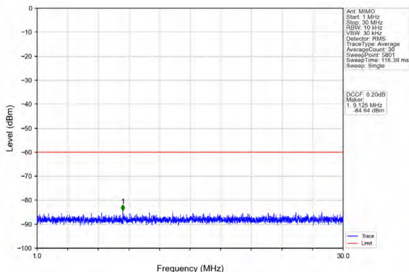
n48_30kHz_MIMO_NTNV_20MHz_CP-OFDM_QPSK_3690MHz_Edge_1RB_Right
