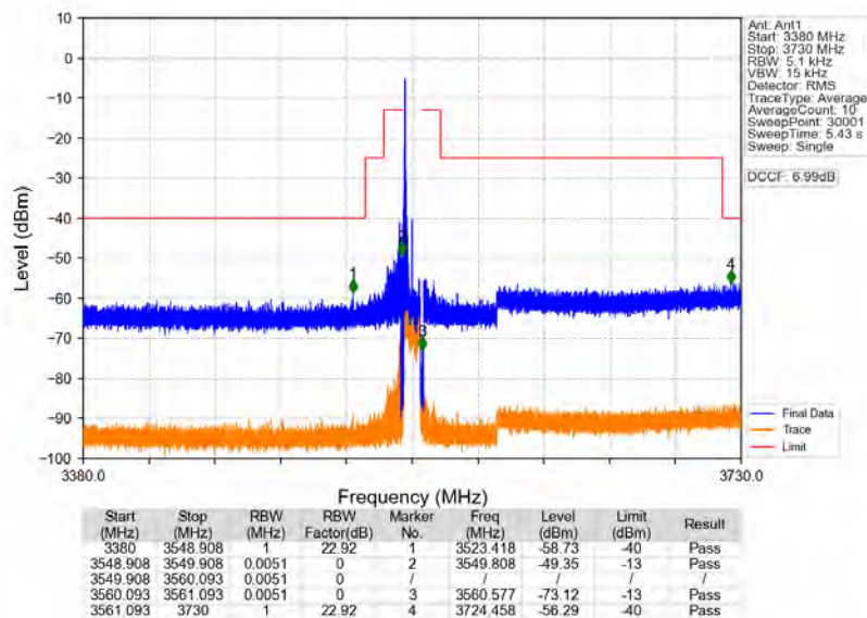
n48_30kHz_MIMO_NTNV_10MHz_CP-OFDM_QPSK_3555MHz_Inner_1RB_Left
