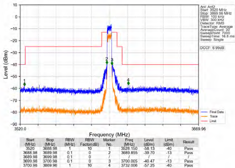
n48_30kHz_MIMO_NTNV_10MHz_CP-OFDM_QPSK_3694.98MHz_Outer_Full
