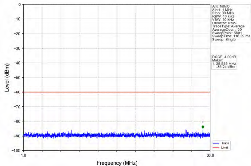
n48_30kHz_MIMO_NTNV_10MHz_CP-OFDM QPSK_3555MHz_Inner_1RB_Left
