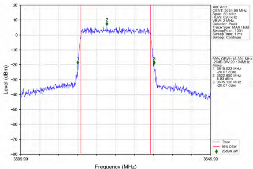
n48_30kHz_MIMO_NTNV_20MHz_CP-OFDM_256_QAM_3624.99MHz_Outer_Full
