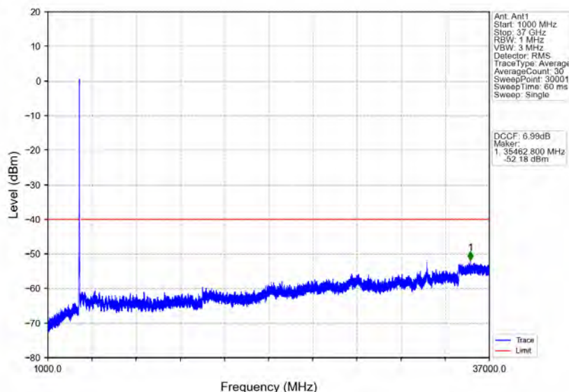
n48_30kHz_MIMO_NTNV_20MHz_CP-OFDM_QPSK_3560.01MHz_Outer_Full
