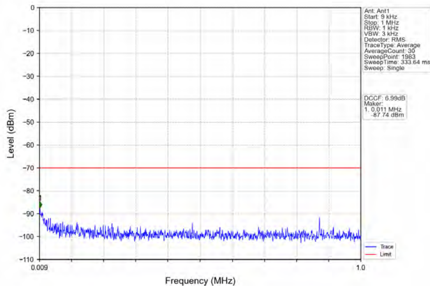
n48_30kHz_MIMO_NTNV_20MHz_CP-OFDM_QPSK_3690MHz_Inner_1RB_Right
