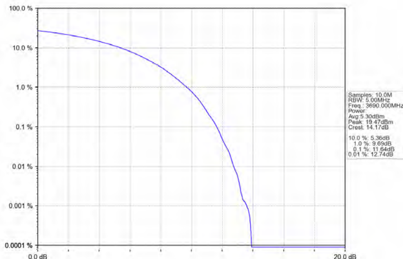
n48_30kHz_MIMO_NTNV_20MHz_CP-OFDM_QPSK_3690MHz_Outer_Full
