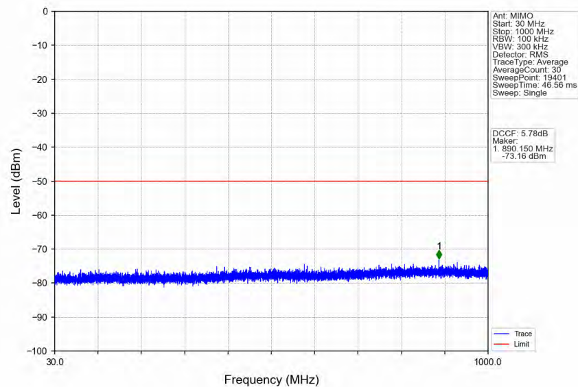
n48_30kHz_MIMO_NTNV_20MHz_CP-OFDM_QPSK_3560.01MHz_Outer_Full
