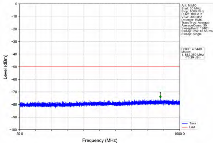
n48_30kHz_MIMO_NTNV_10MHz_CP-OFDM_QPSK_3694.98MHz_Inner_1RB_Right
