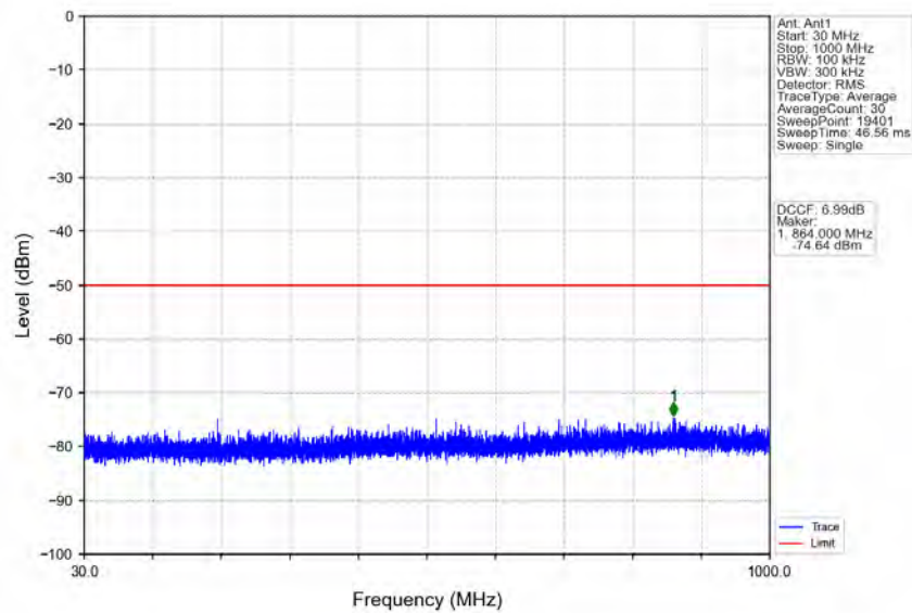
n48_30kHz_MIMO_NTNV_10MHz_CP-OFDM_QPSK_3694.98MHz_Edge_1RB_Right
