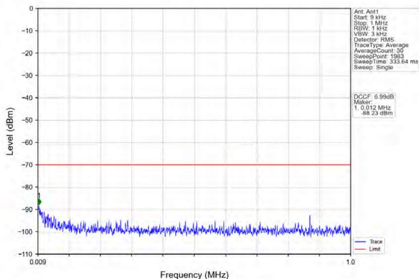
n48_30kHz_MIMO_NTNV_10MHz_CP-OFDM_QPSK_3555MHz_Outer_Full
