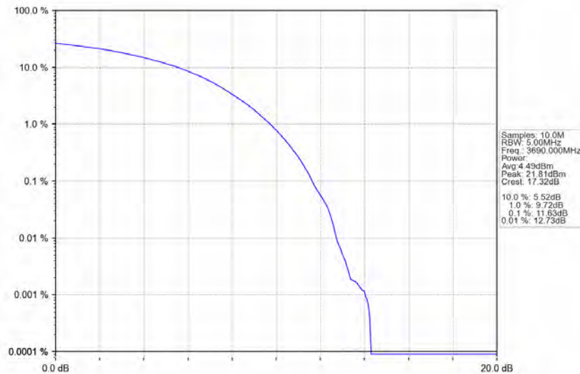
n48_30kHz_MIMO_NTNV_20MHz_CP-OFDM_64_QAM_3690MHz_Outer_Full
