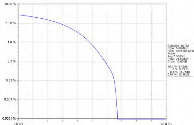
n48_30kHz_MIMO_NTNV_10MHz_CP-OFDM_QPSK_3624.99MHz_Outer_Full
