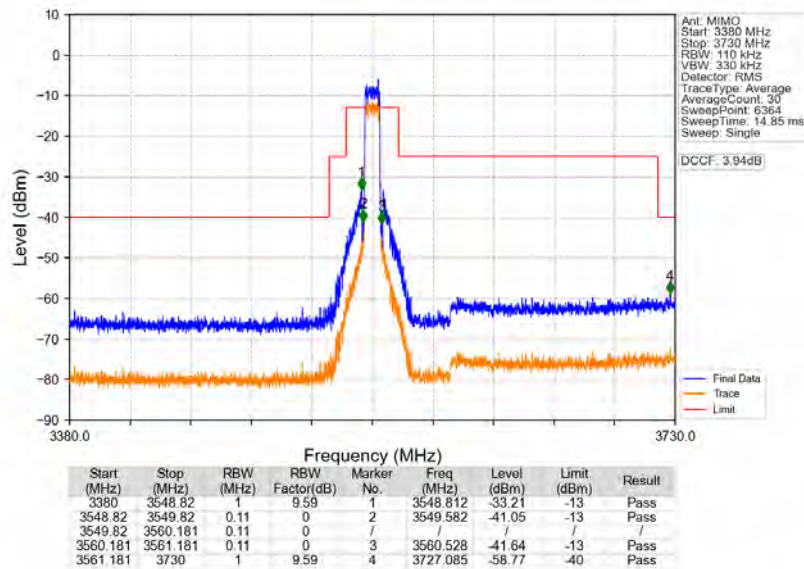
n48_30kHz_MIMO_NTNV_10MHz_CP-OFDM_QPSK_3555MHz_Outer_Full
