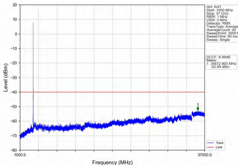
n48_30kHz_MIMO_NTNV_20MHz_CP-OFDM_QPSK_3560.01MHz_Edge_1RB_Left
