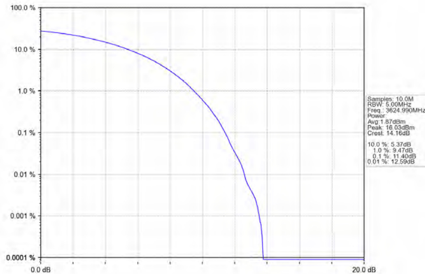
n48_30kHz_MIMO_NTNV_40MHz_CP-OFDM_QPSK_3624.99MHz_Outer_Full
