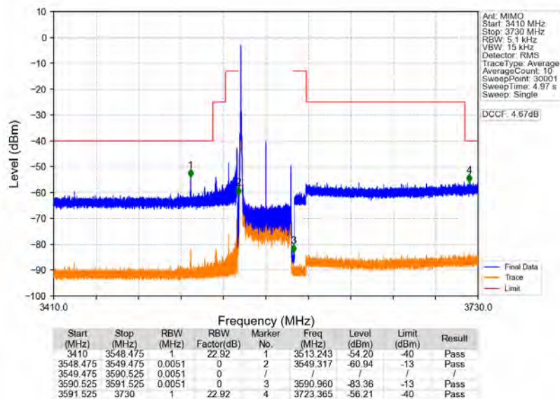
n48_30kHz_MIMO_NTNV_40MHz_CP-OFDM_QPSK_3570MHz_Edge_1RB_Left
