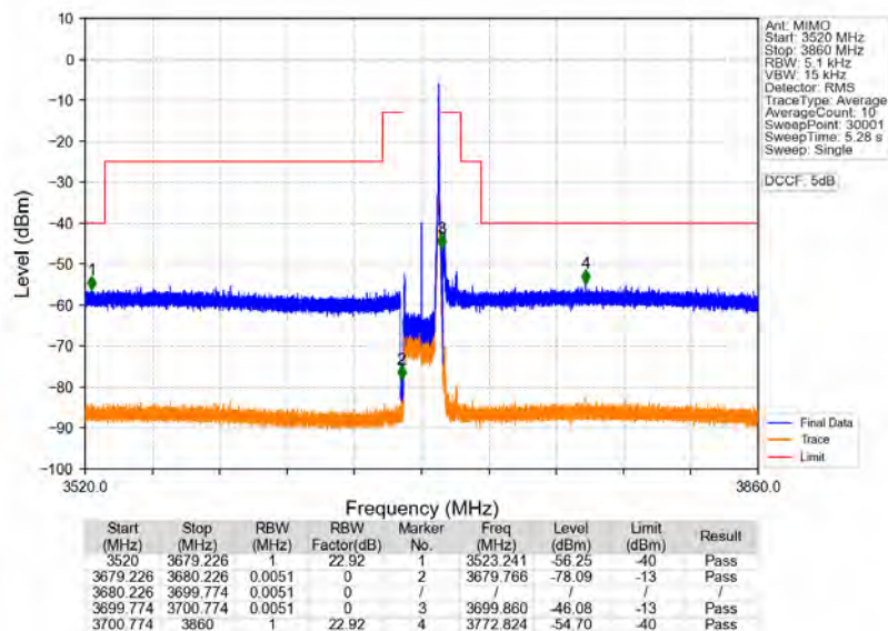
n48_30kHz_MIMO_NTNV_20MHz_CP-OFDM_QPSK_3690MHz_Inner_1RB_Right
