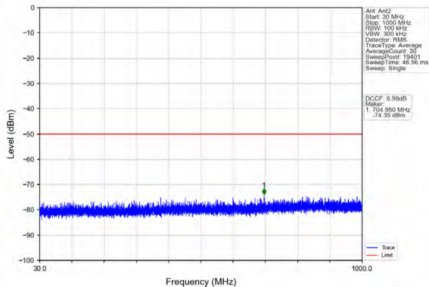
n48_30kHz_MIMO_NTNV_10MHz_CP-OFDM_QPSK_3555MHz_Outer_Full
