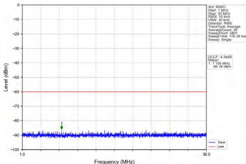
n48_30kHz_MIMO_NTNV_10MHz_CP-OFDM_QPSK_3694.98MHz_Inner_1RB_Right
