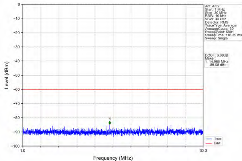
n48_30kHz_MIMO_NTNV_20MHz_CP-OFDM_QPSK_3690MHz_Inner_1RB_Right
