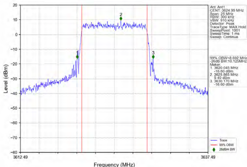
n48_30kHz_MIMO_NTNV_10MHz_CP-OFDM_16_QAM_3624.99MHz_Outer_Full
