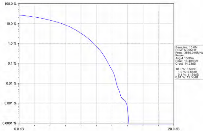
n48_30kHz_MIMO_NTNV_20MHz_CP-OFDM 64 QAM_3560.01MHz_Outer_Full
