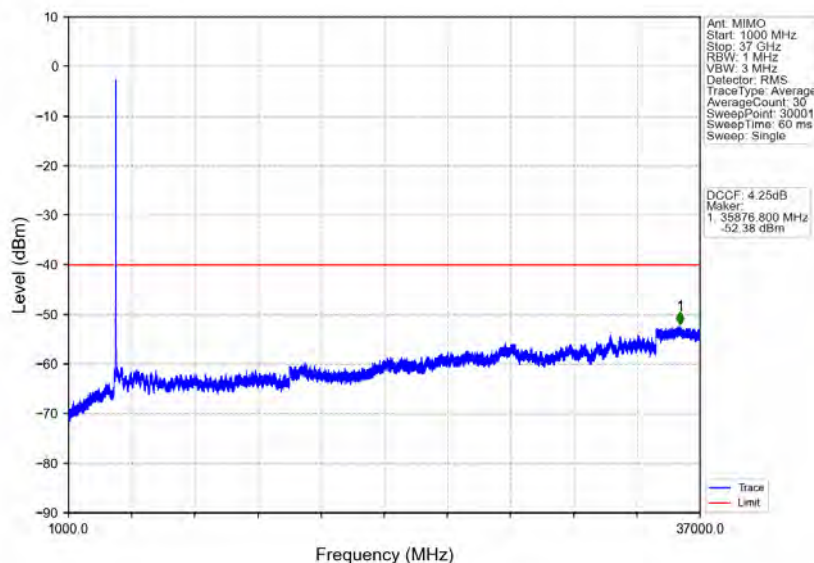
n48_30kHz_MIMO_NTNV_20MHz_CP-OFDM_QPSK_3690MHz_Inner_1RB_Right
