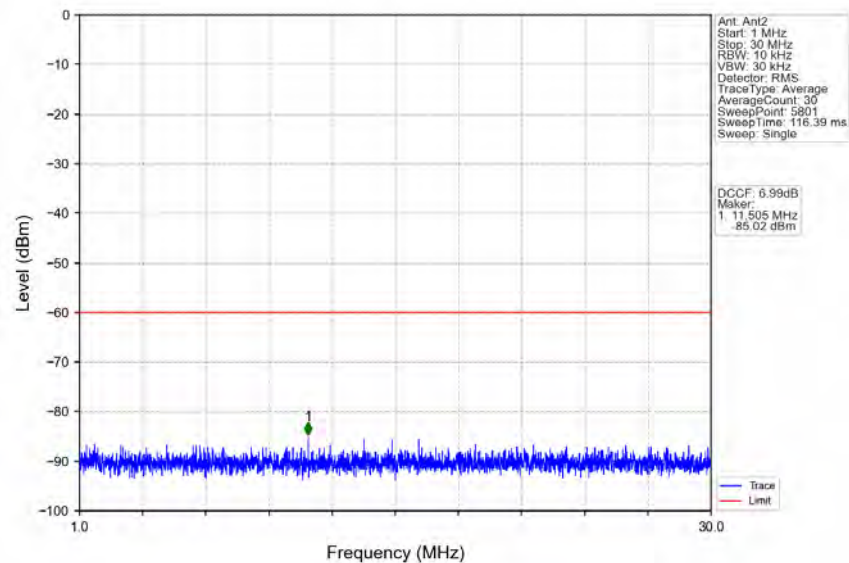
n48_30kHz_MIMO_NTNV_10MHz_CP-OFDM_QPSK_3694.98MHz_Outer_Full
