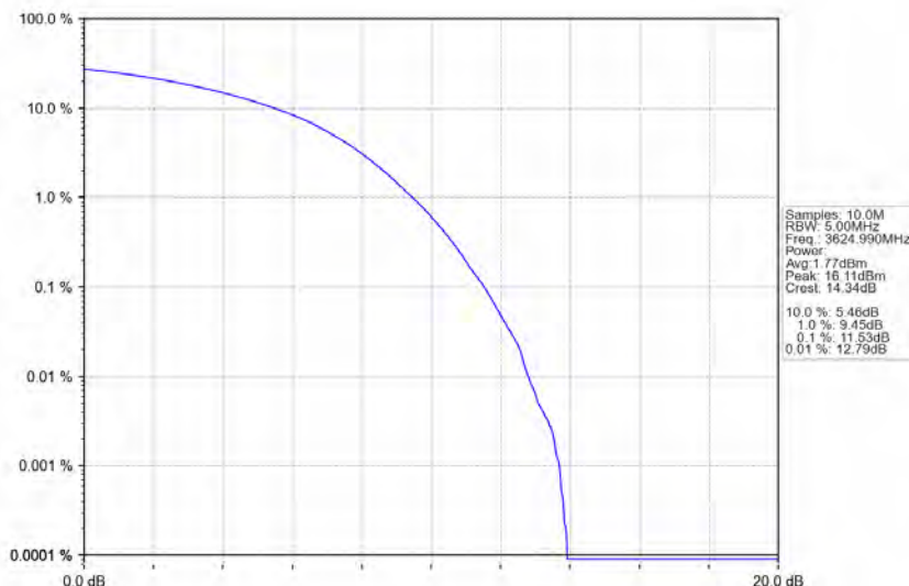
n48_30kHz_MIMO_NTNV_40MHz_CP-OFDM_16_QAM_3624.99MHz_Outer_Full
