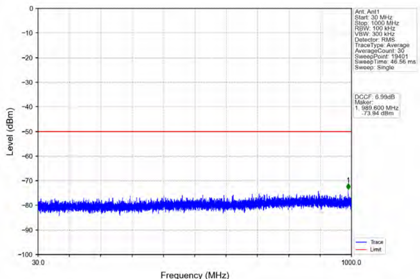
n48_30kHz_MIMO_NTNV_40MHz_CP-OFDM_QPSK_3570MHz_Edge_1RB_Left
