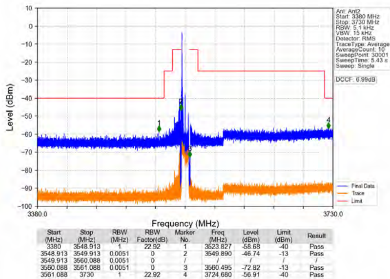
n48_30kHz_MIMO_NTNV_10MHz_CP-OFDM_QPSK_3555MHz_Inner_1RB_Left
