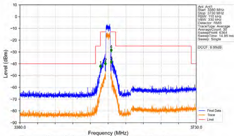
n48_30kHz_MIMO_NTNV_10MHz_CP-OFDM_QPSK_3555MHz_Outer_Full
