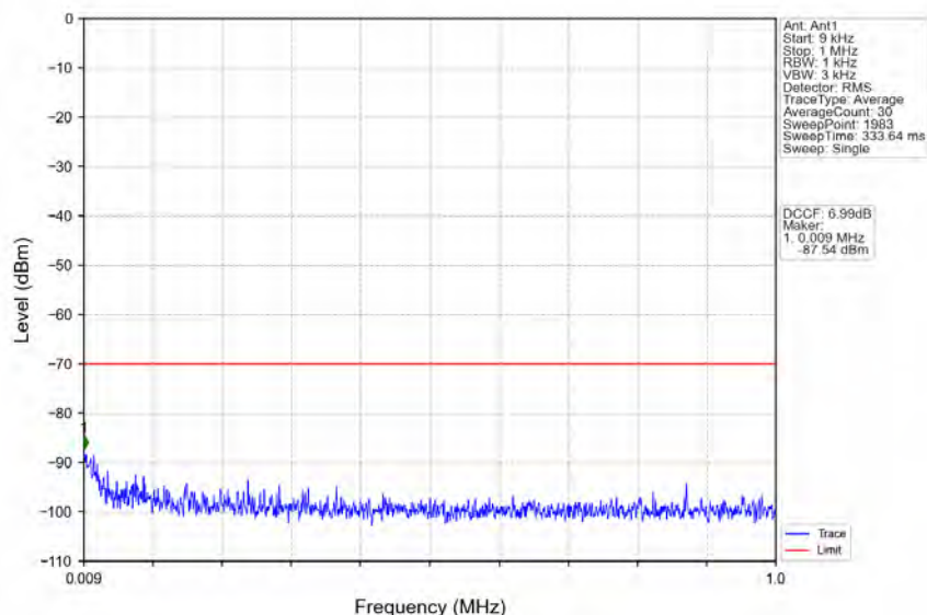
n48_30kHz_MIMO_NTNV_20MHz_CP-OFDM_QPSK_3560.01MHz_Inner_1RB_Left
