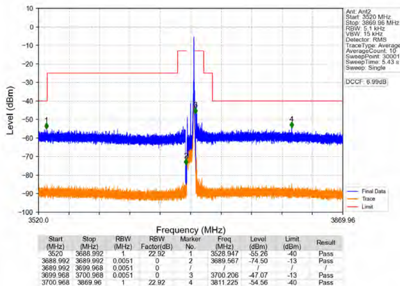
n48_30kHz_MIMO_NTNV_10MHz_CP-OFDM_QPSK_3694.98MHz_Inner_1RB_Right
