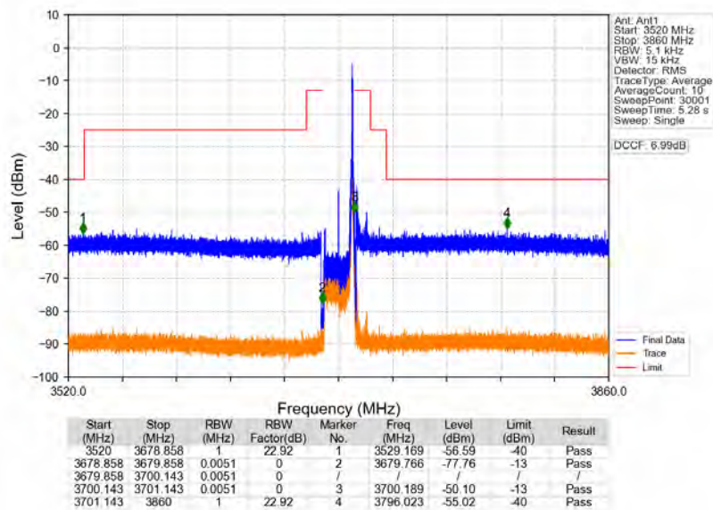
n48_30kHz_MIMO_NTNV_20MHz_CP-OFDM_QPSK_3690MHz_Inner_1RB_Right
