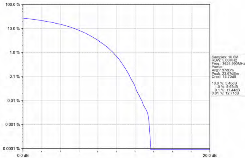
n48_30kHz_MIMO_NTNV_10MHz_CP-OFDM_16_QAM_3624.99MHz_Outer_Full
