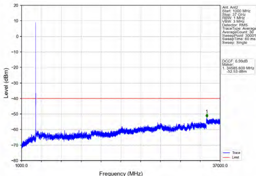
n48_30kHz_MIMO_NTNV_20MHz_CP-OFDM_QPSK_3560.01MHz_Inner_1RB_Left
