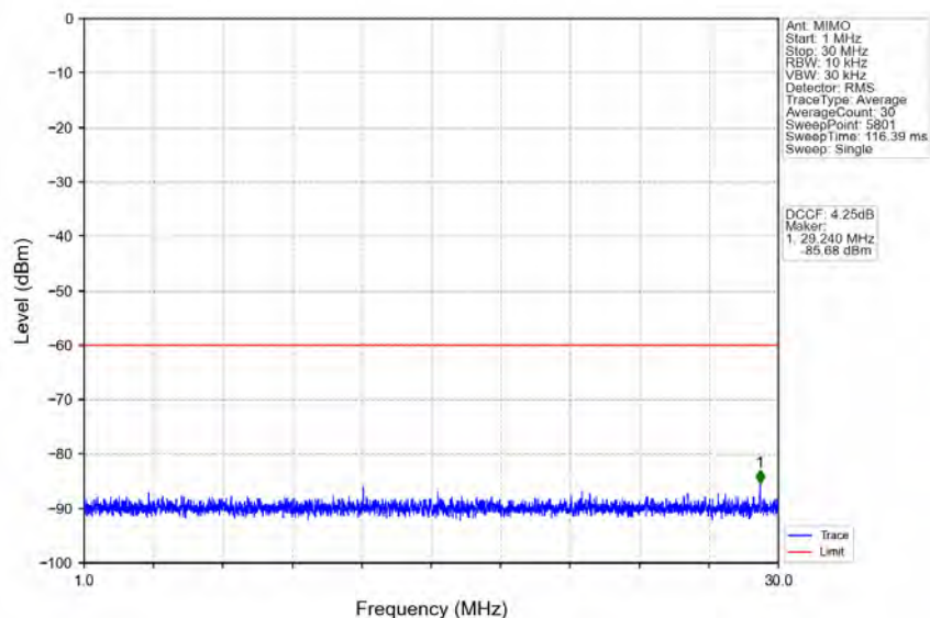
n48_30kHz_MIMO_NTNV_20MHz_CP-OFDM_QPSK_3690MHz_Outer_Full
