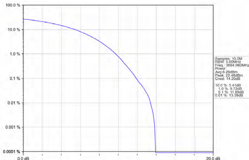
n48_30kHz_MIMO_NTNV_10MHz_CP-OFDM_QPSK_3694.98MHz_Outer_Full
