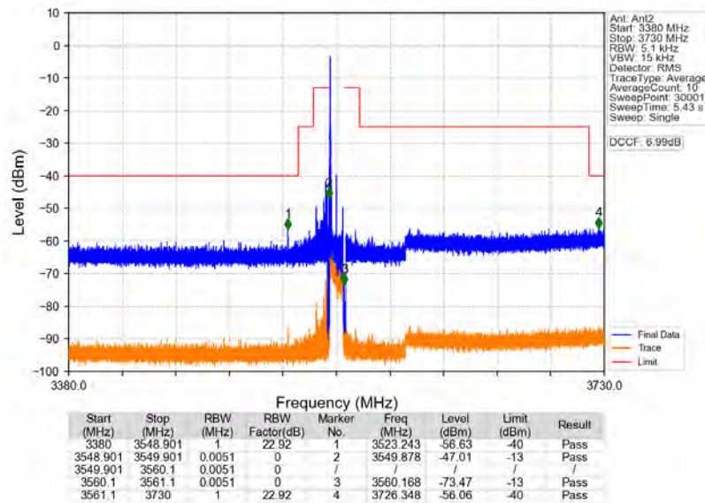
n48_30kHz_MIMO_NTNV_10MHz_CP-OFDM_QPSK_3555MHz_Edge_1RB_Left
