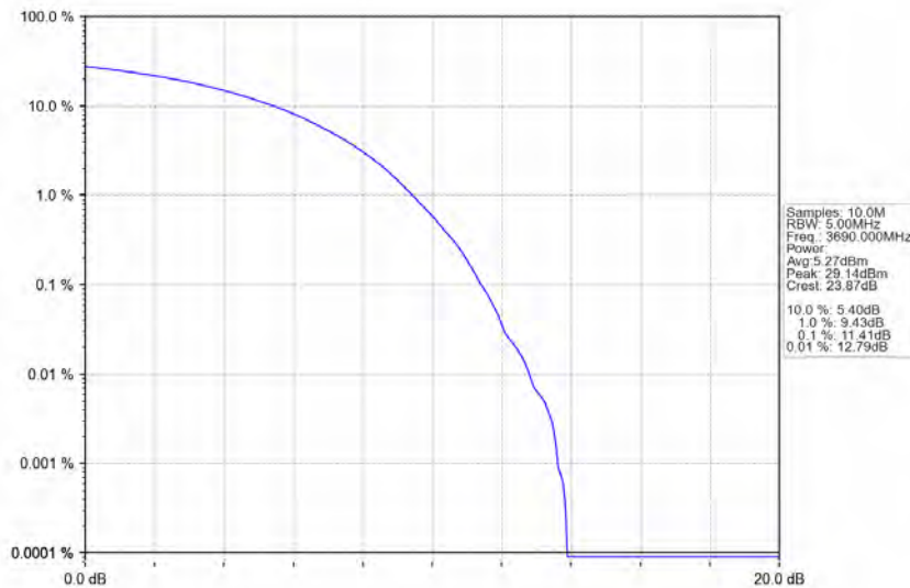
n48_30kHz_MIMO_NTNV_20MHz_CP-OFDM 16 QAM_3690MHz_Outer_Full
