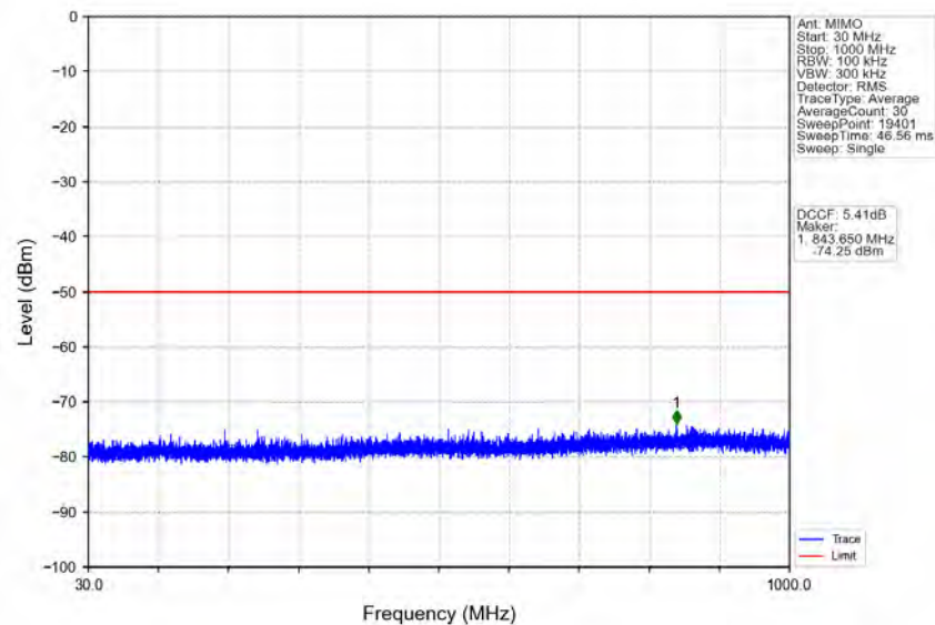
n48_30kHz_MIMO_NTNV_10MHz_CP-OFDM_QPSK_3694.98MHz_Edge_1RB_Right
