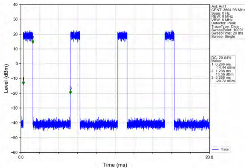
n48_30kHz_MIMO_NTNV_10MHz_CP-OFDM 64 QAM 3694.98MHz_Inner_Full
