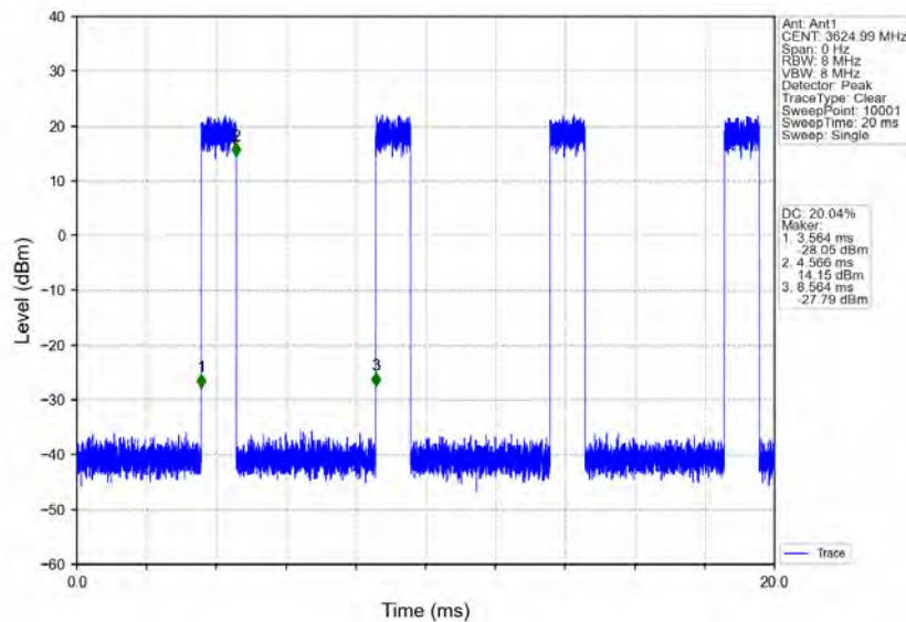
n48_30kHz_MIMO_NTNV_10MHz_CP-OFDM 64 QAM 3624.99MHz_Inner_Full
