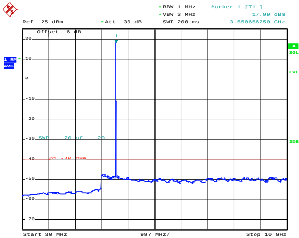
16QAM Low channel 1RB0
