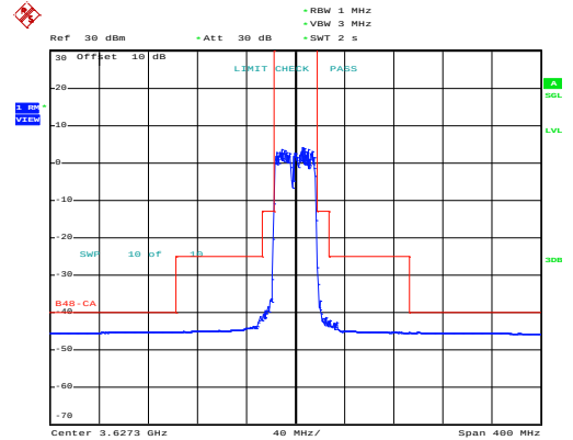
QPSK Middle channel Full RB
