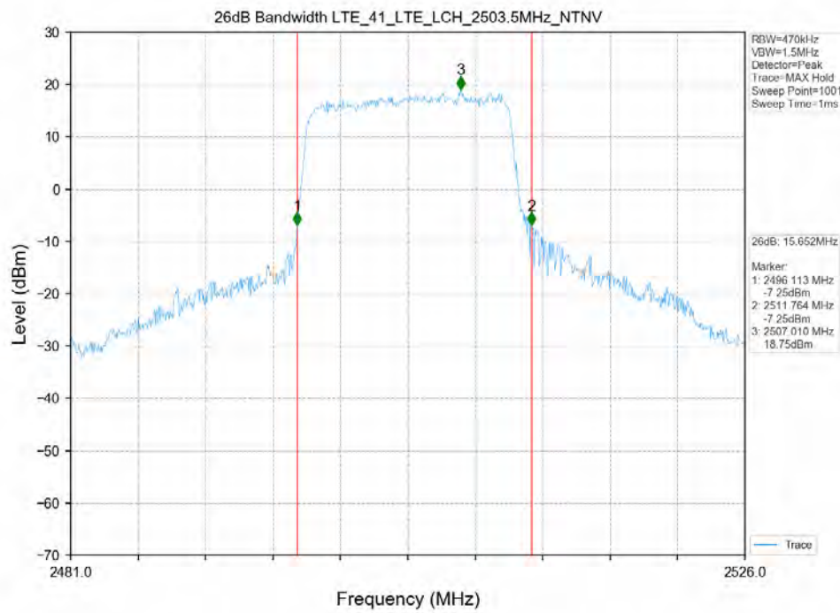
64QAM LCH
