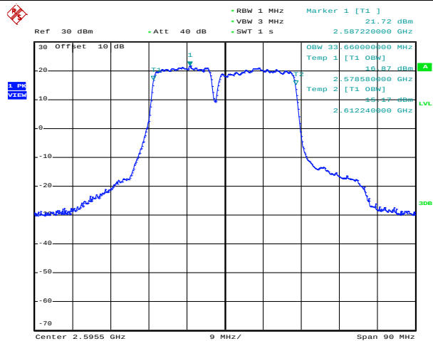
16QAM
