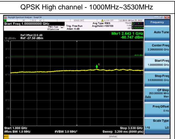
QPSK High channel - 1000MHz~3530MHz
