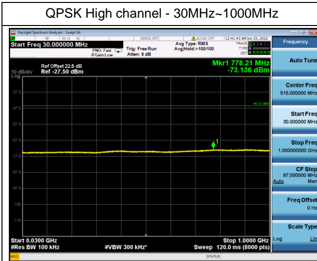
QPSK High channel - 30MHz~1000MHz
