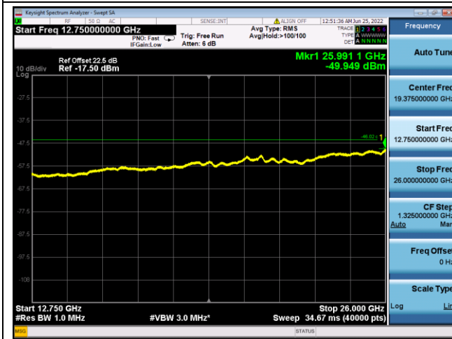
QPSK High channel – 12.75GHz~26GHz
