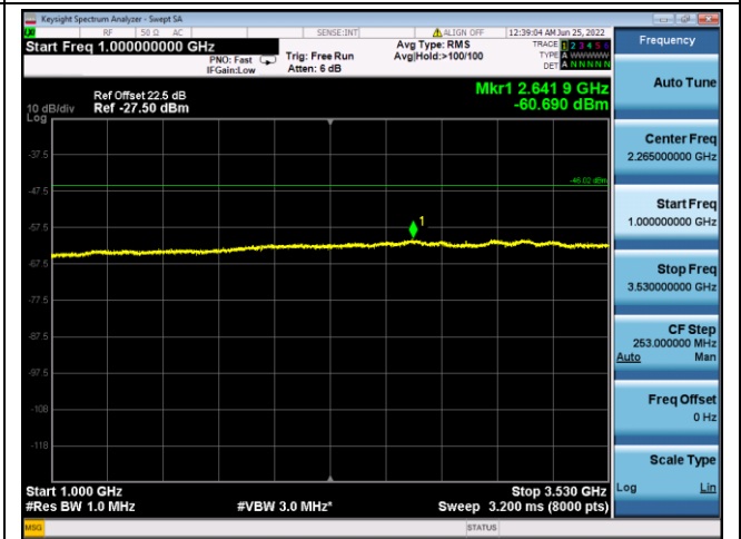
QPSK Middle channel - 1000MHz~3530MHz
