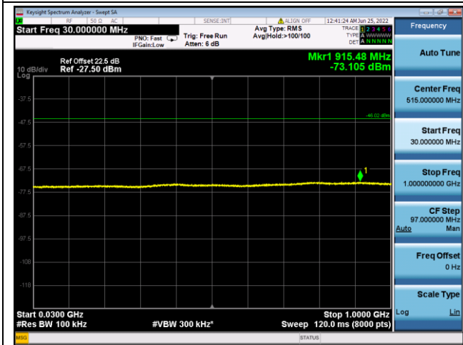
QPSK Middle channel - 30MHz~1000MHz
