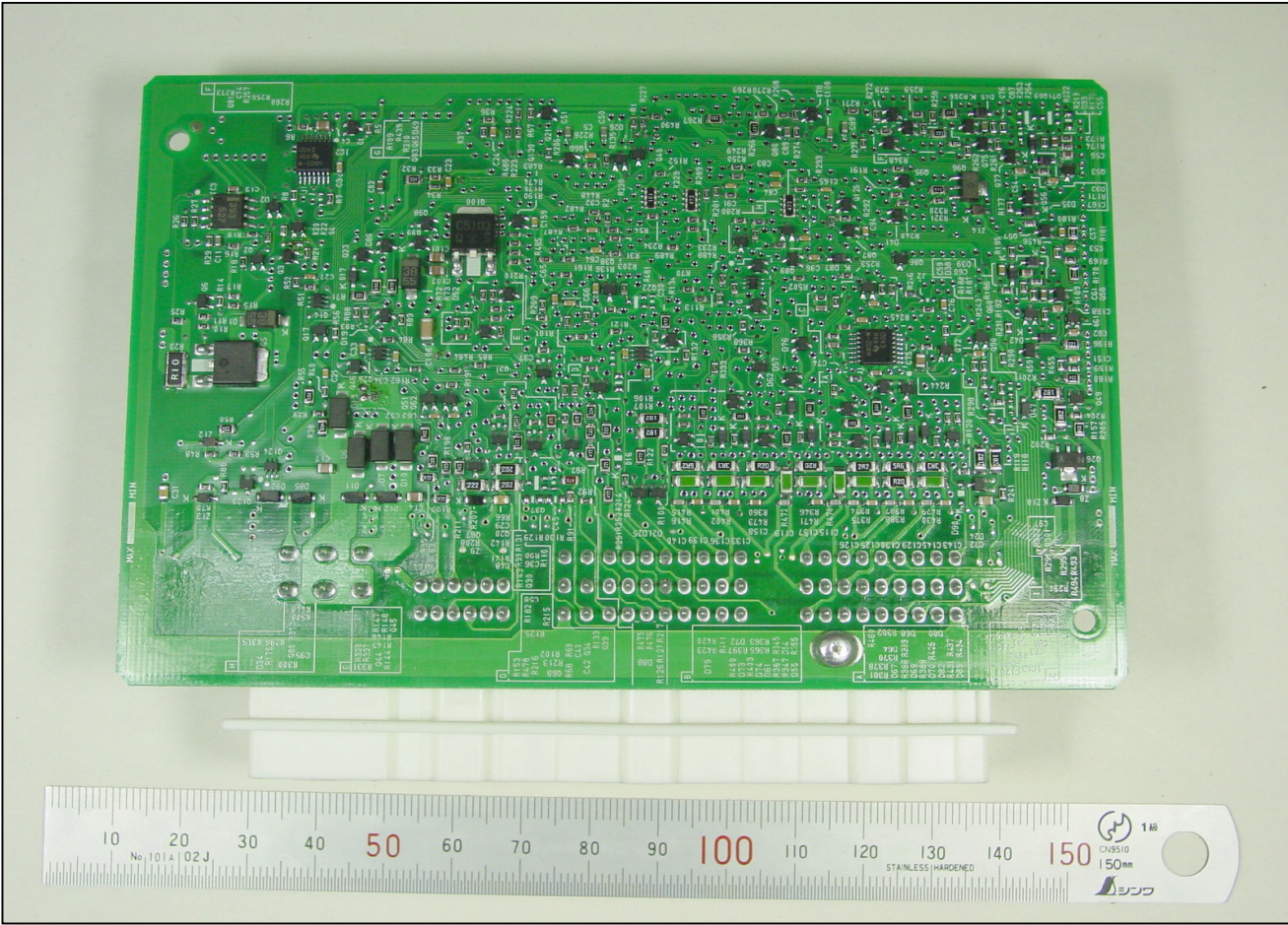
SOLDER SIDE
