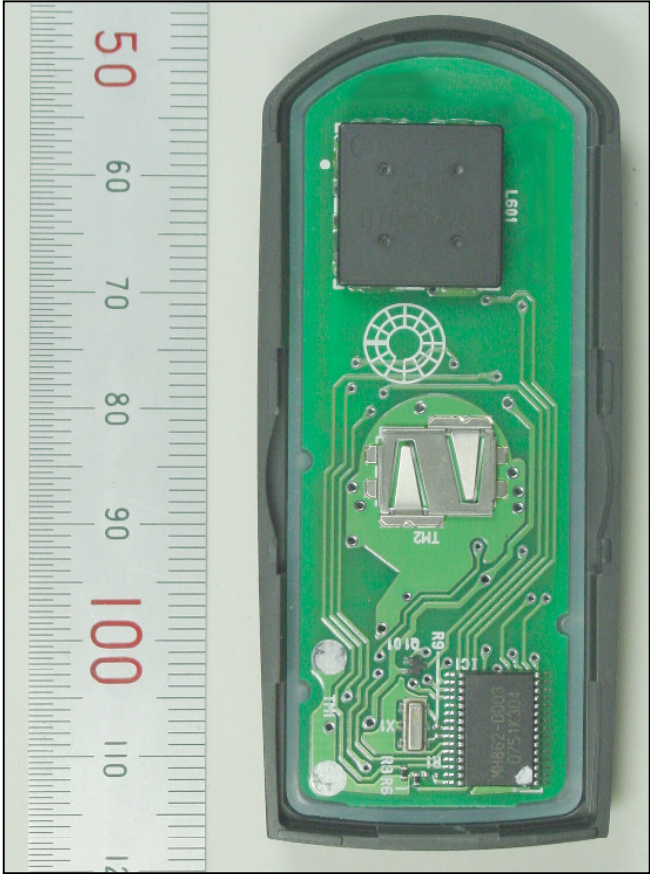
SOLDER SIDE
