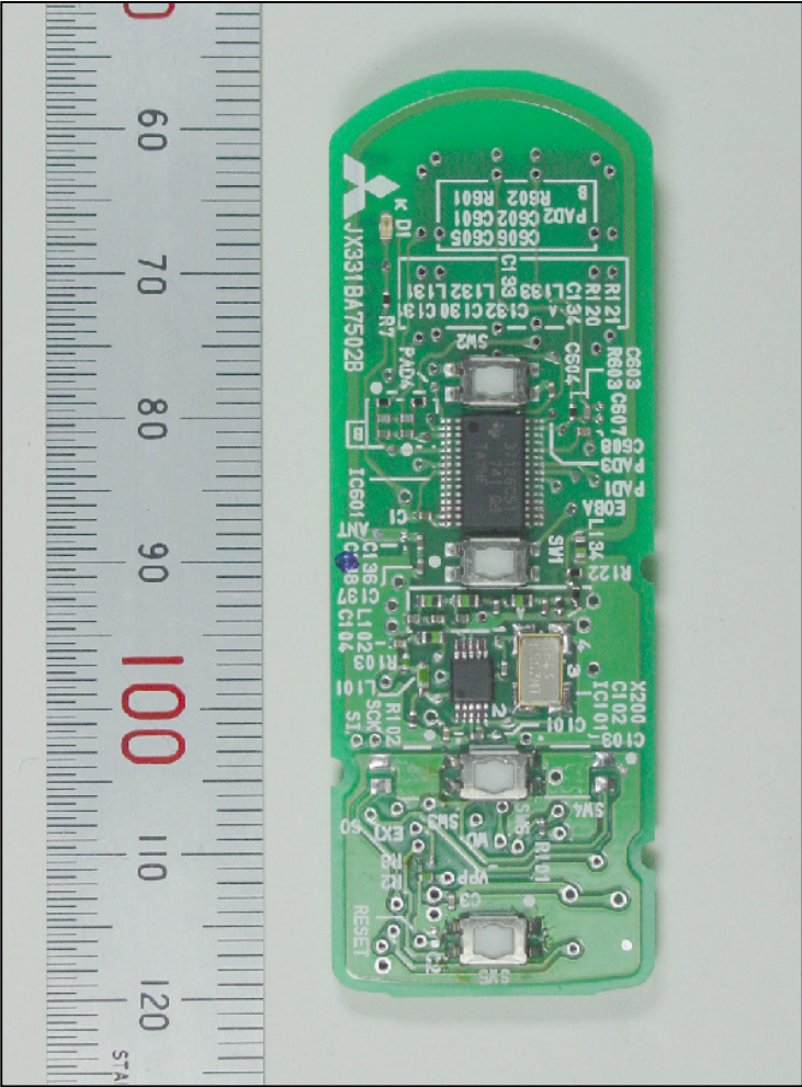
COMPONENT SIDE
