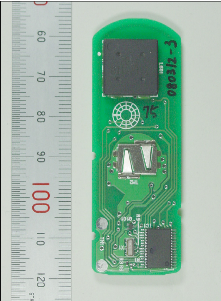
SOLDER SIDE
