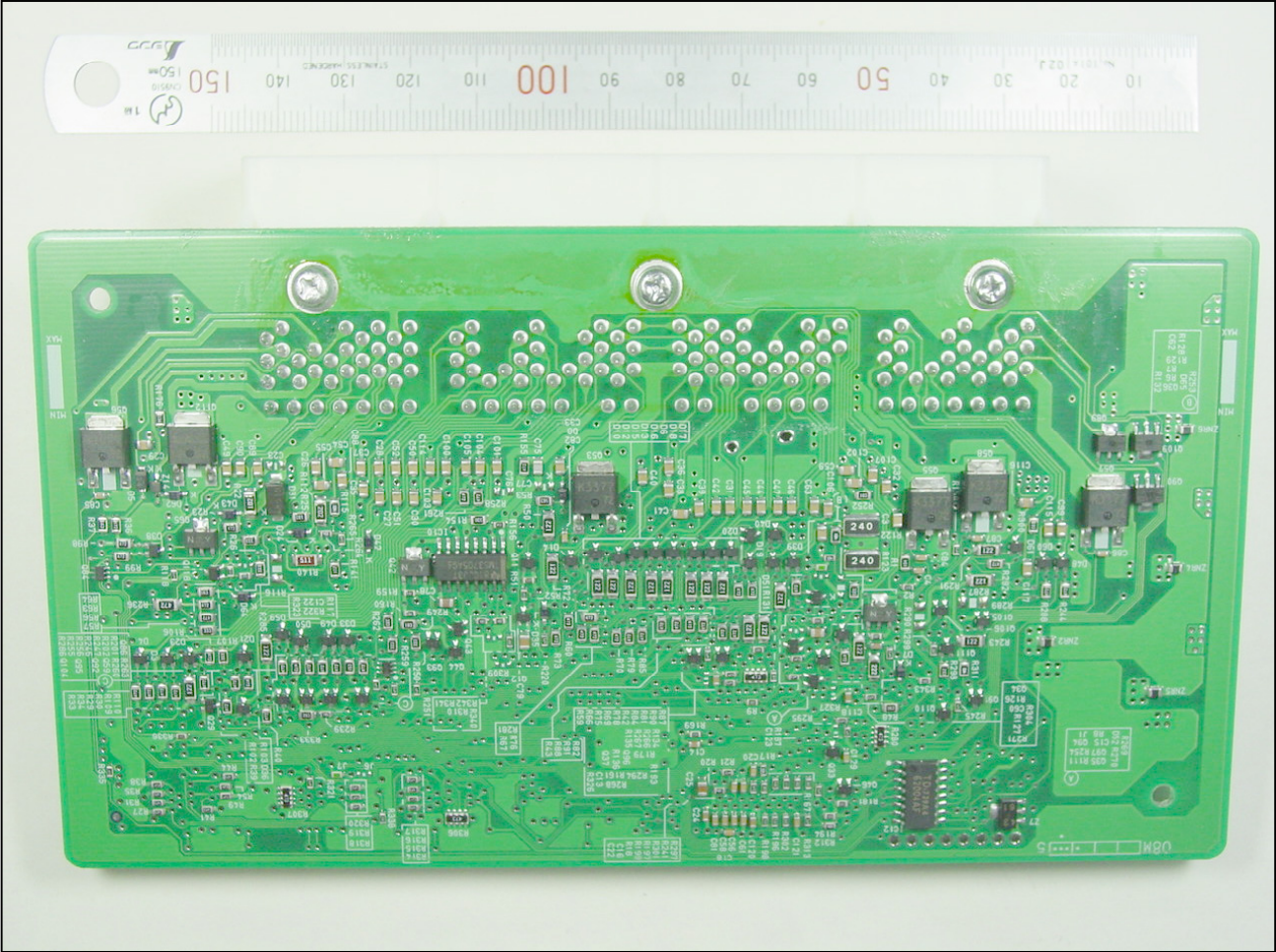
COMPONENT SIDE
