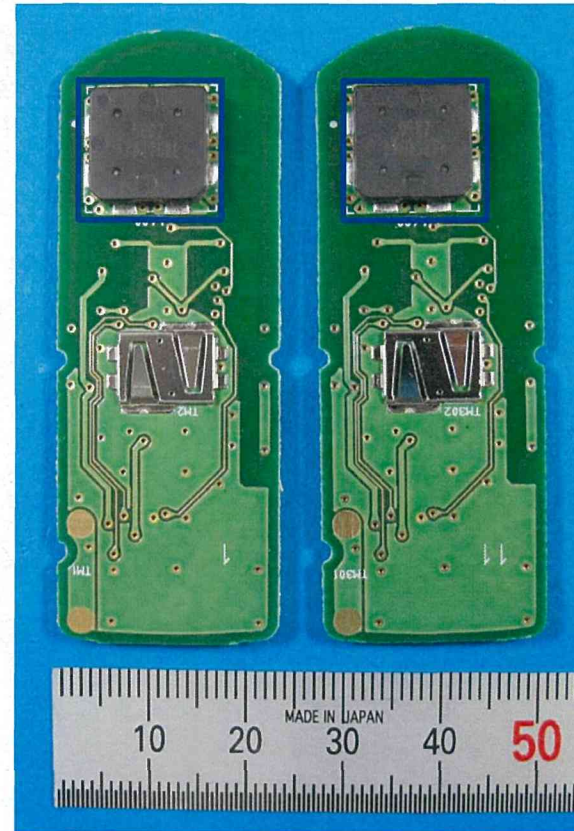
□ Inductive antenna (Receive)
