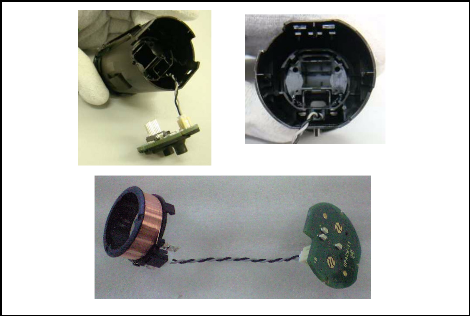
Antenna coil
