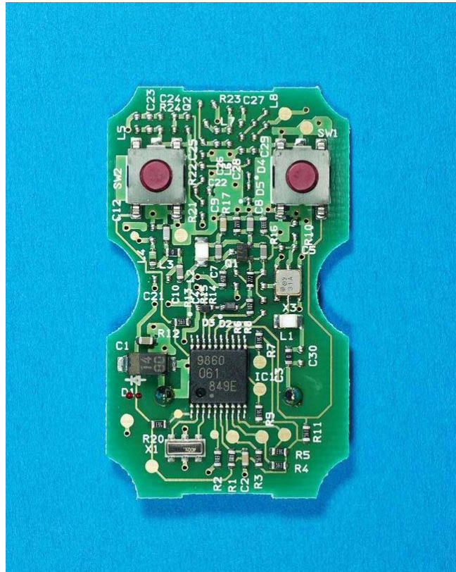
Component Side
