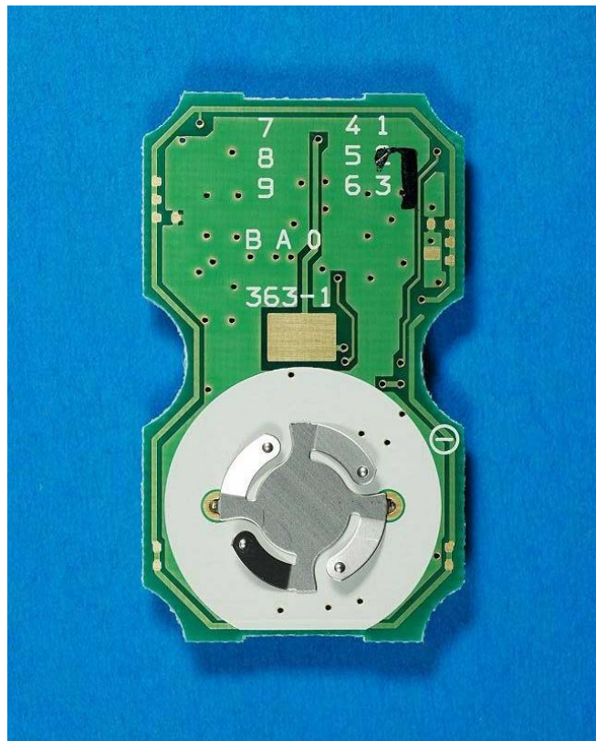
Soldering Side
