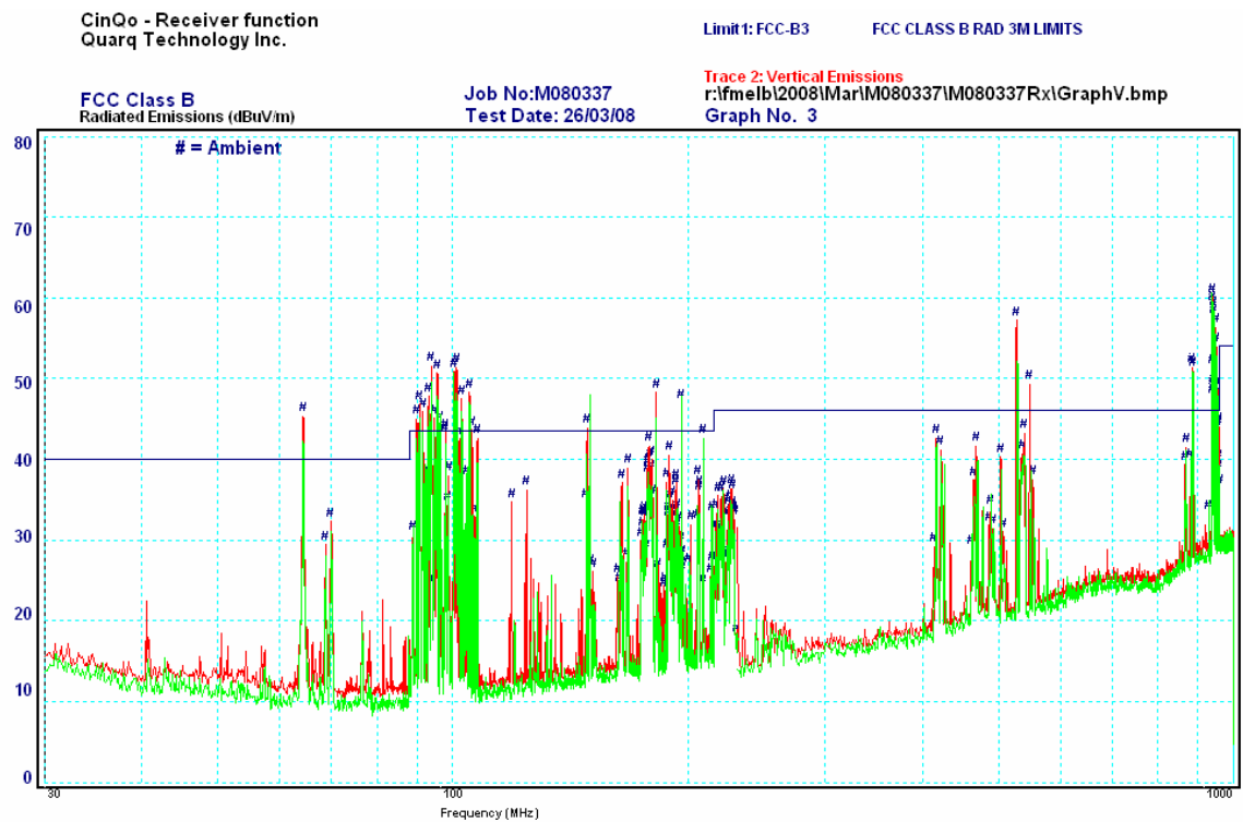
Graph 3 Vertical emissions, 30 MHz to 1000 MHz. EUT in receive mode.
