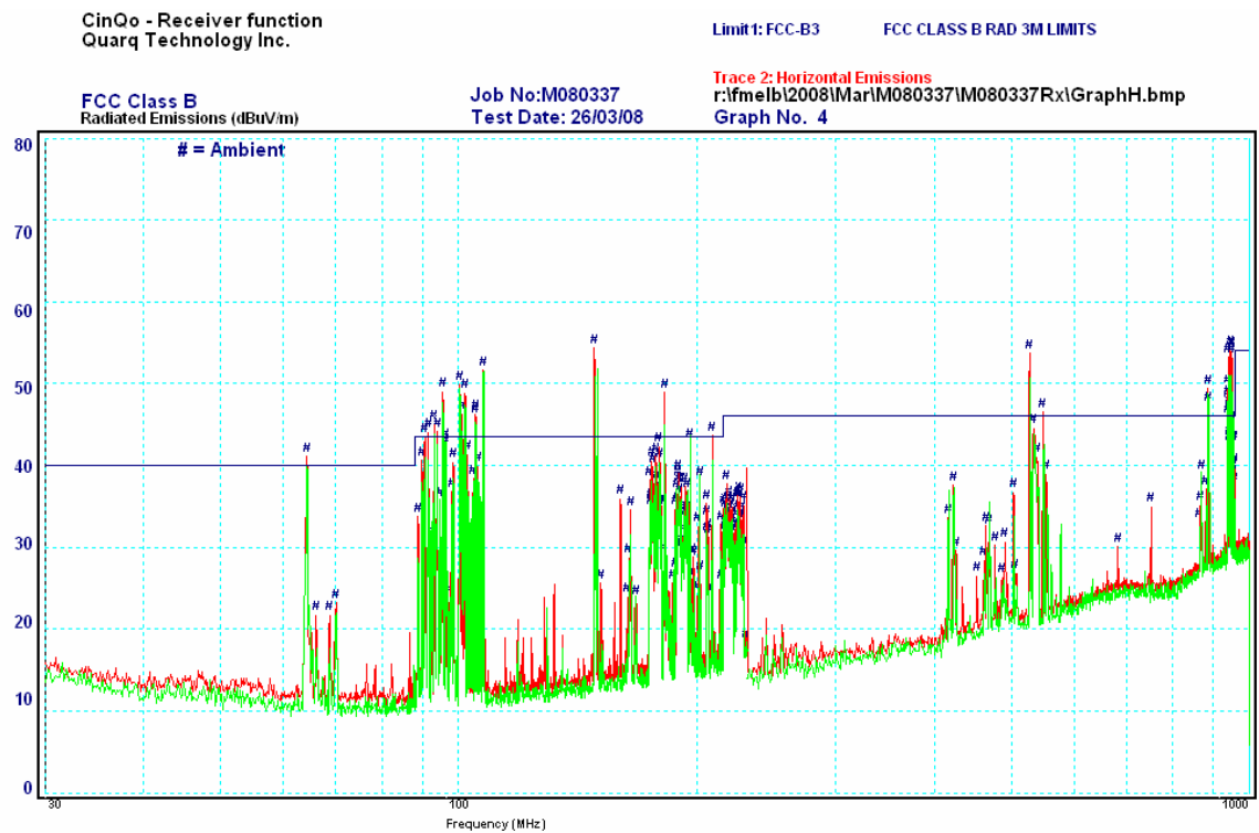
Graph 4 Horizontal emissions, 30 MHz to 1000 MHz. EUT in receive mode.
