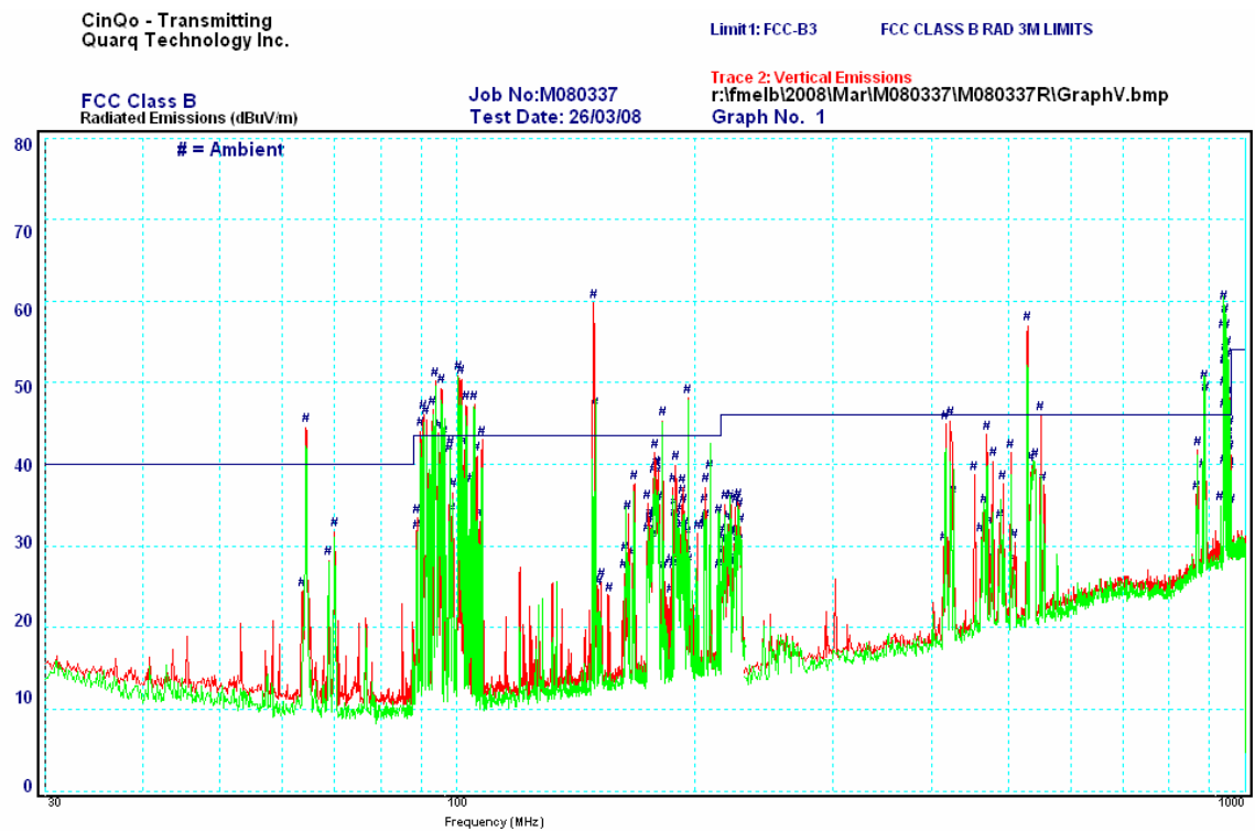
Graph 1 Vertical emissions, 30 MHz to 1000 MHz. EUT transmitting.
