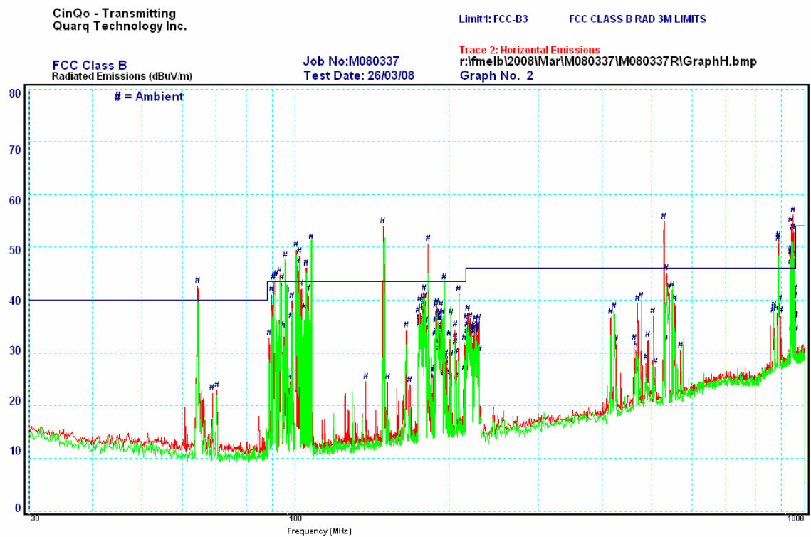
Graph 2 Horizontal emissions, 30 MHz to 1000 MHz. EUT transmitting.
