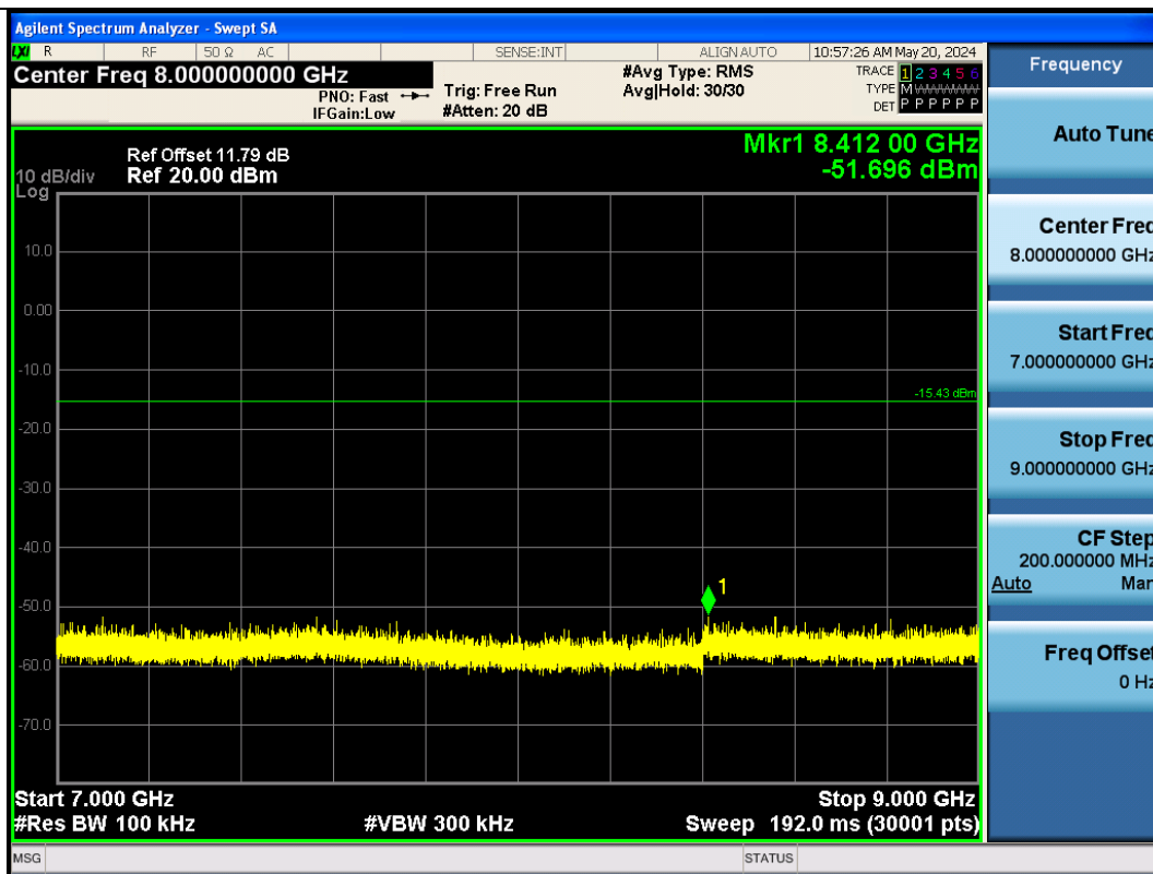
BLE_500K-Ant1-2402-7000~9000-PASS
