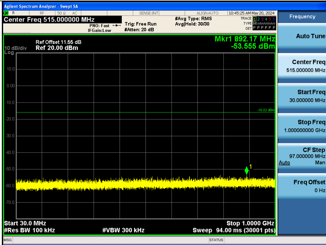
BLE_125K-Ant1-2440-30~1000-PASS
