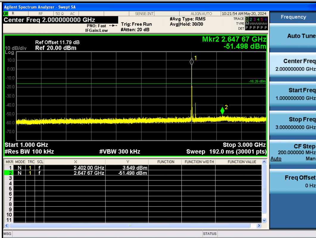
BLE_2M-Ant1-2402-1000~3000-PASS
