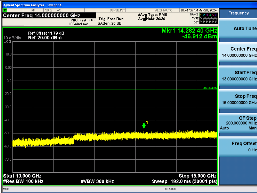
BLE_125K-Ant1-2402-13000~15000-PASS
