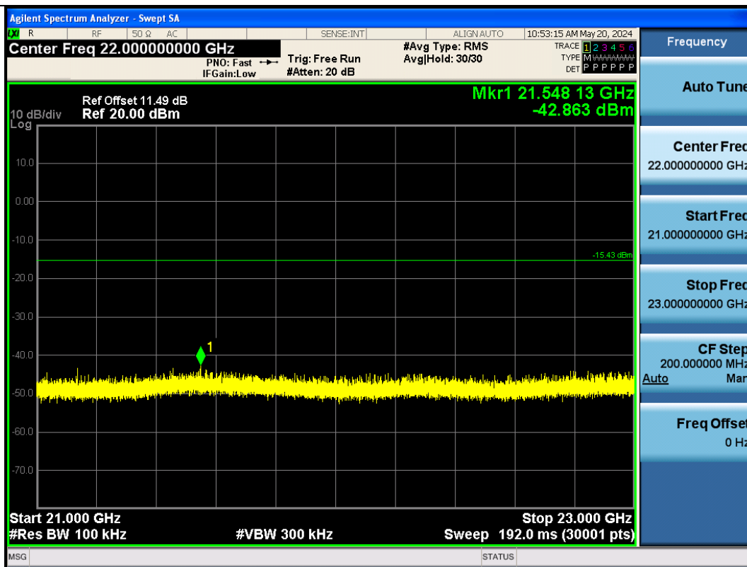
BLE_125K-Ant1-2480-21000~23000-PASS
