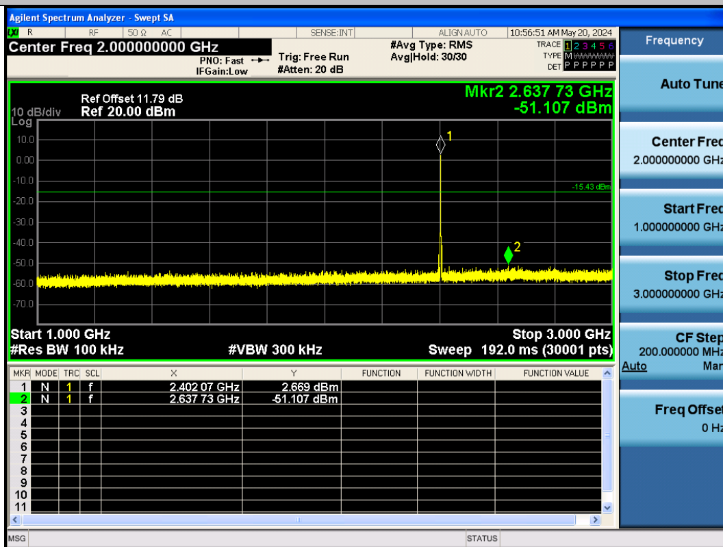
BLE_500K-Ant1-2402-1000~3000-PASS
