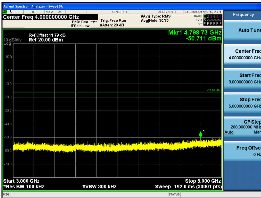
BLE_2M-Ant1-2402-3000~5000-PASS
