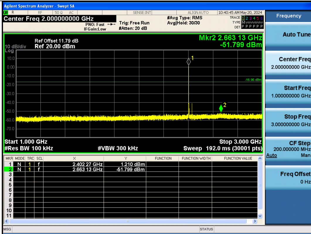
BLE_125K-Ant1-2402-1000~3000-PASS
