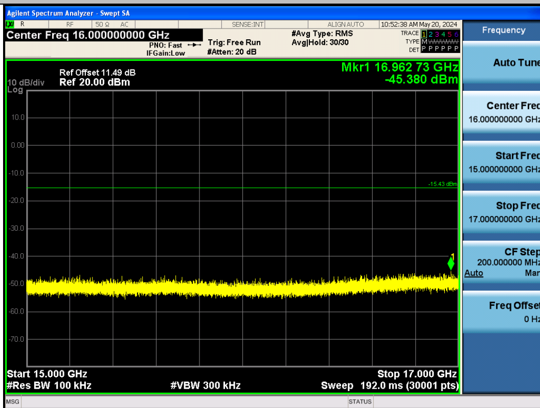
BLE_125K-Ant1-2480-15000~17000-PASS
