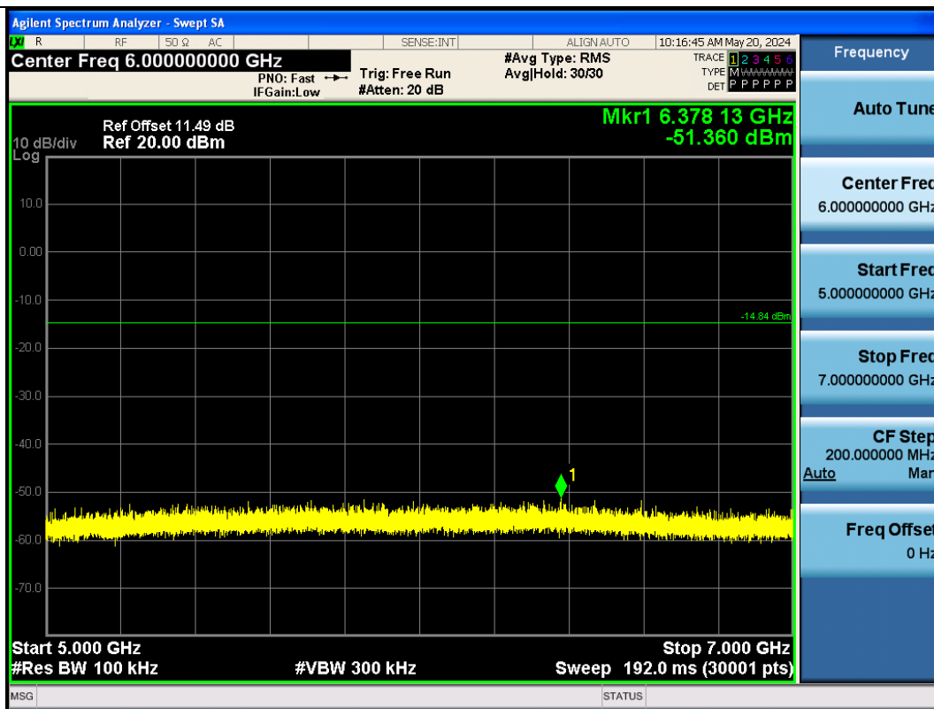
BLE_1M-Ant1-2480-5000~7000-PASS
