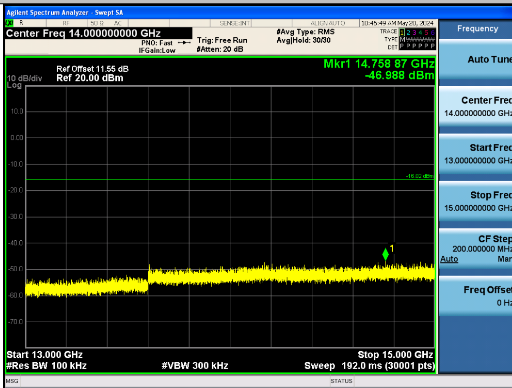
BLE_125K-Ant1-2440-13000~15000-PASS
