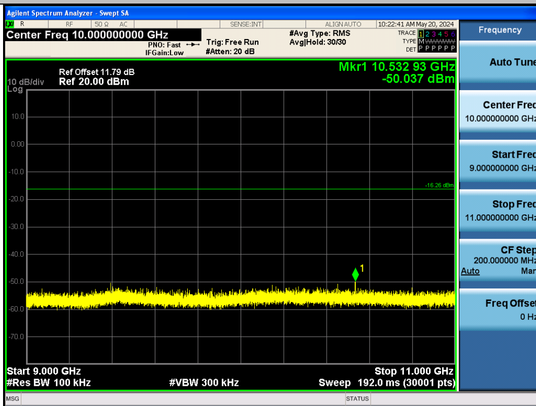
BLE_2M-Ant1-2402-9000~11000-PASS
