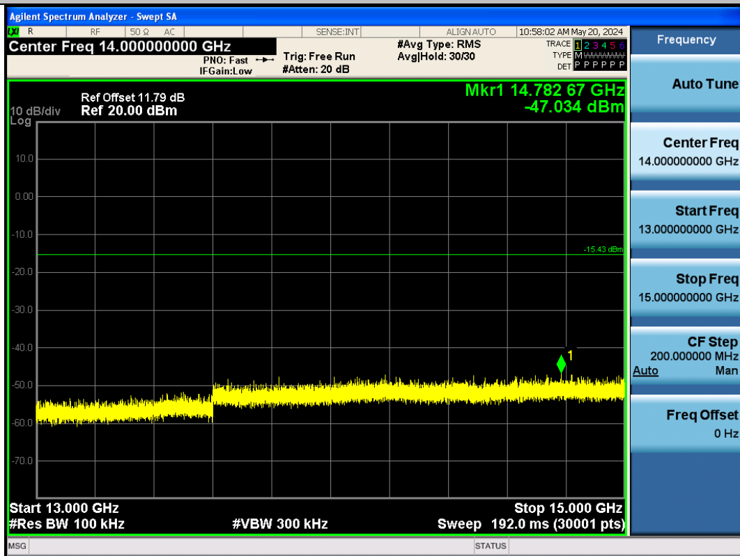
BLE_500K-Ant1-2402-13000~15000-PASS
