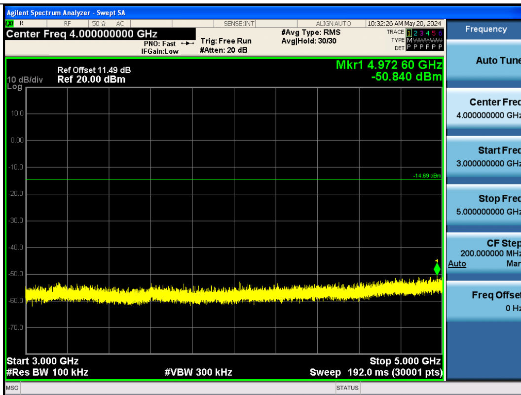
BLE_2M-Ant1-2480-3000~5000-PASS
