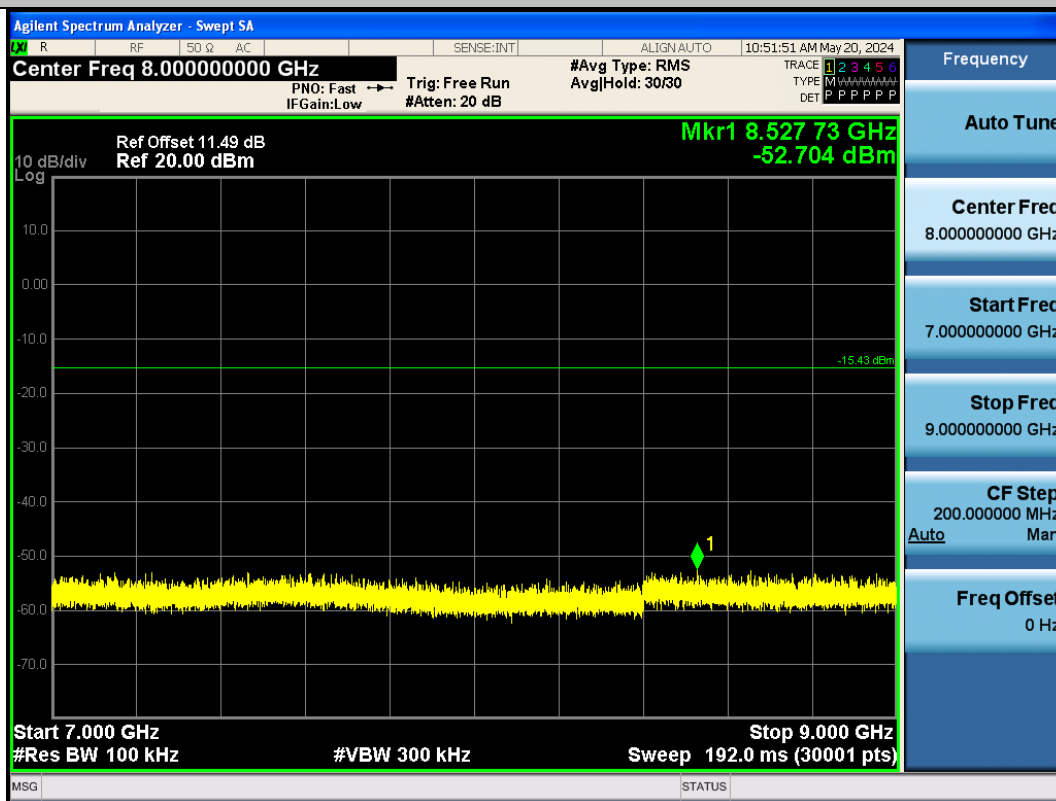
BLE_125K-Ant1-2480-7000~9000-PASS
