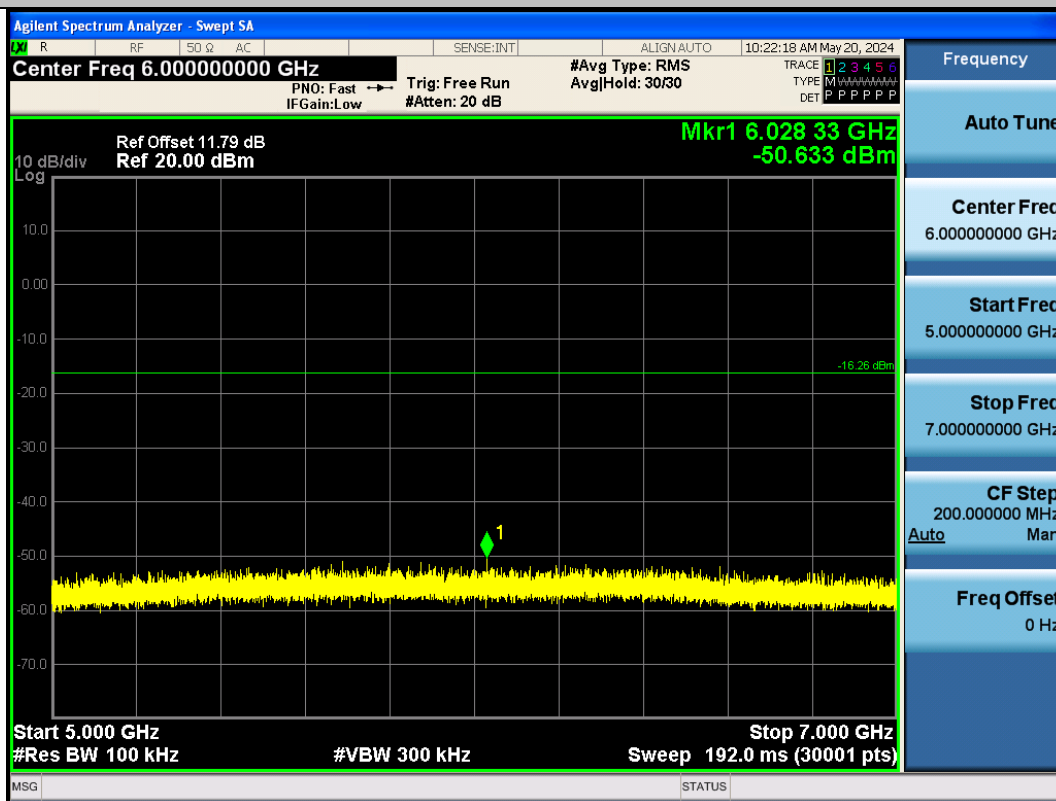
BLE_2M-Ant1-2402-5000~7000-PASS
