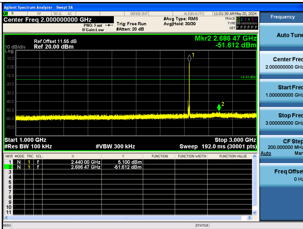
BLE_500K-Ant1-2440-1000~3000-PASS
