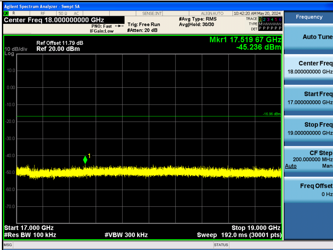
BLE_125K-Ant1-2402-17000~19000-PASS
