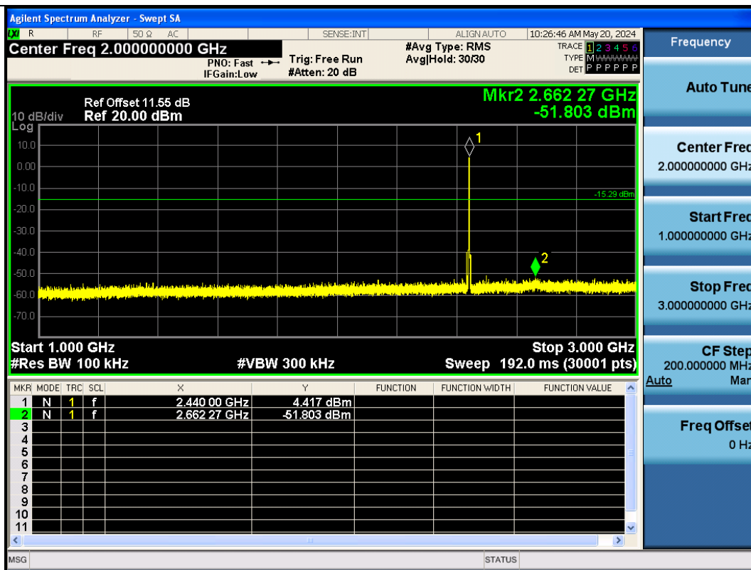
BLE_2M-Ant1-2440-1000~3000-PASS
