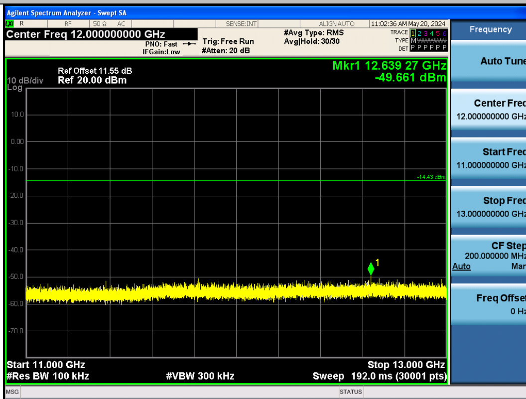
BLE_500K-Ant1-2440-11000~13000-PASS
