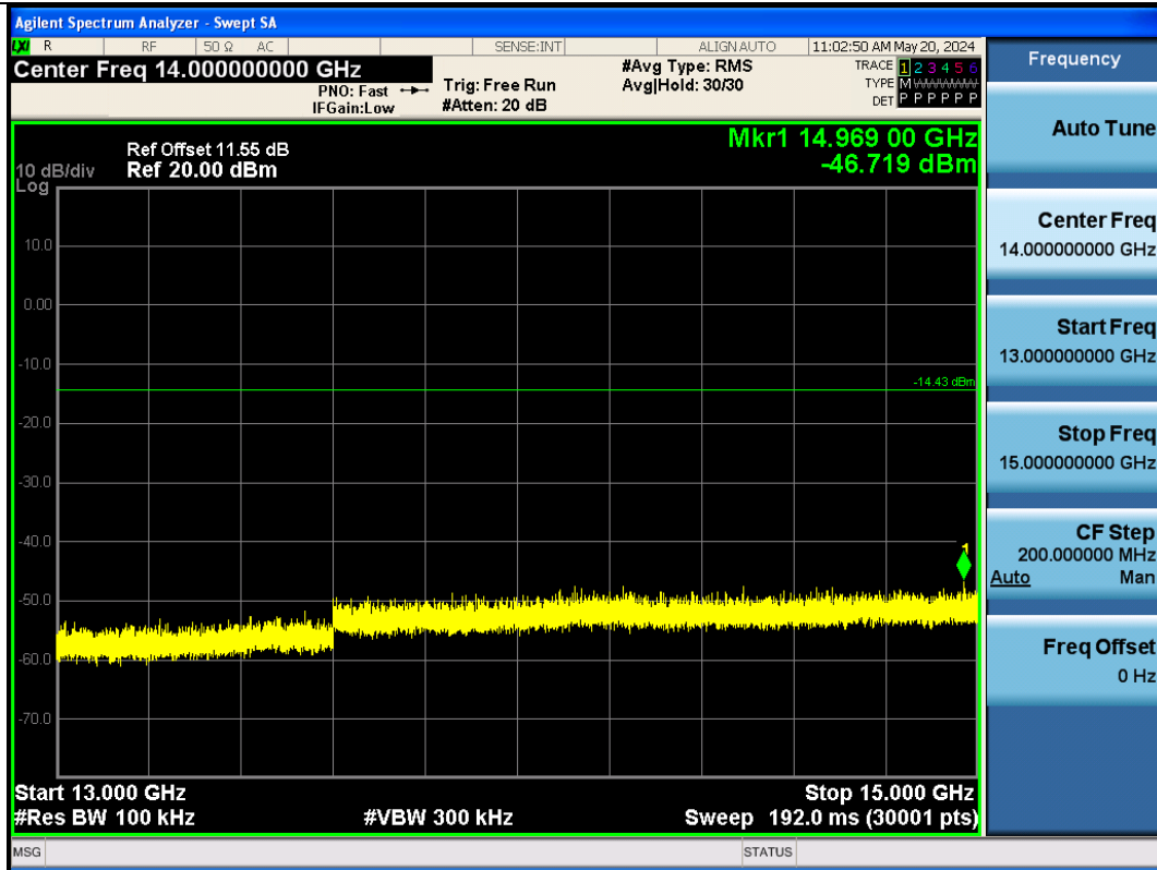
BLE_500K-Ant1-2440-13000~15000-PASS
