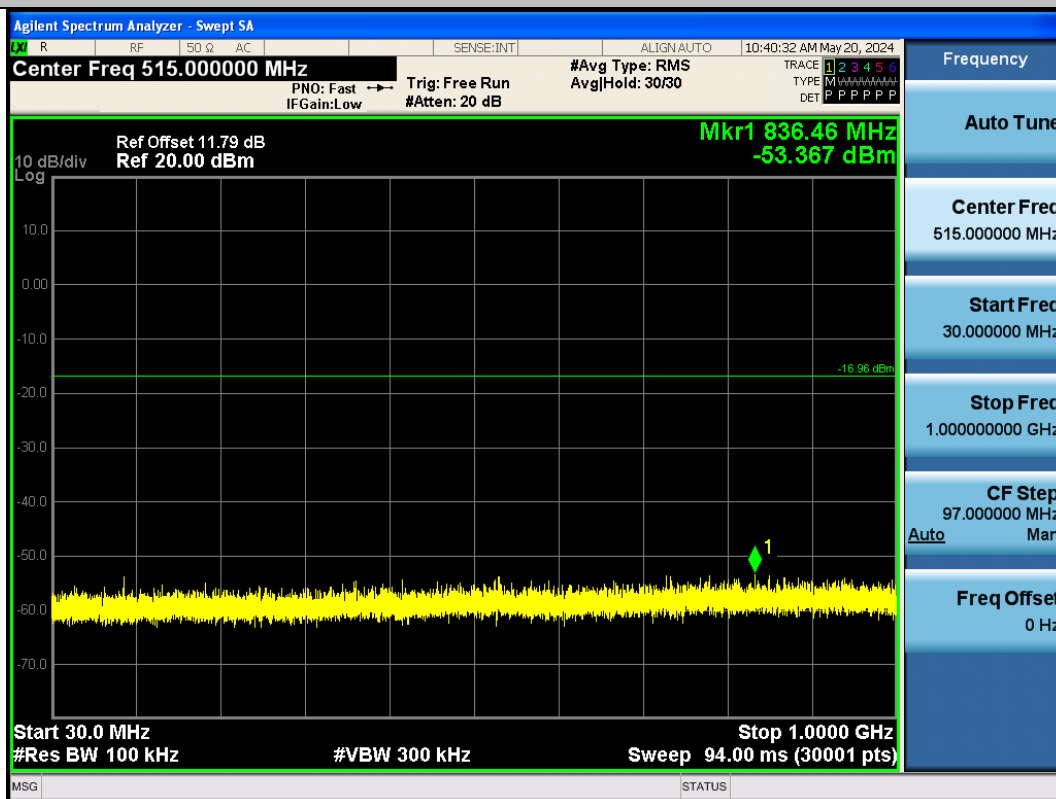
BLE_125K-Ant1-2402-30~1000-PASS
