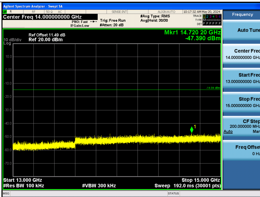
BLE_1M-Ant1-2480-13000~15000-PASS
