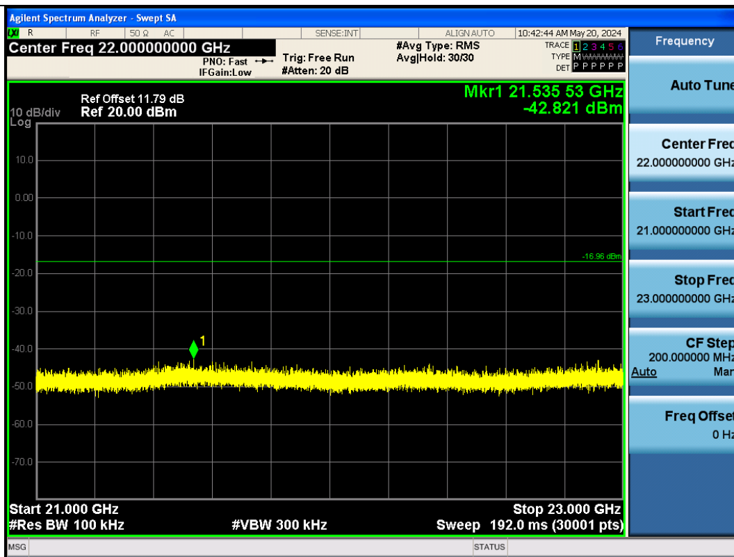
BLE_125K-Ant1-2402-21000~23000-PASS
