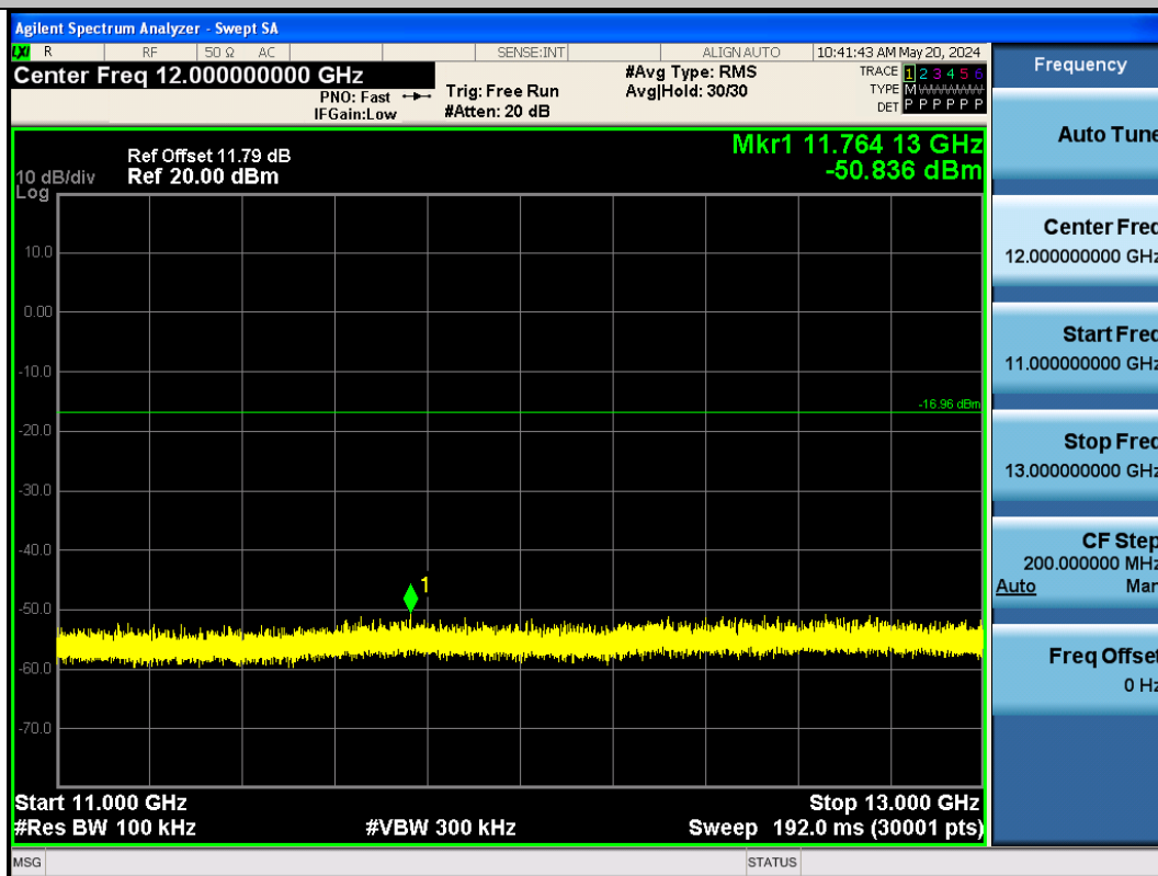
BLE_125K-Ant1-2402-11000~13000-PASS
