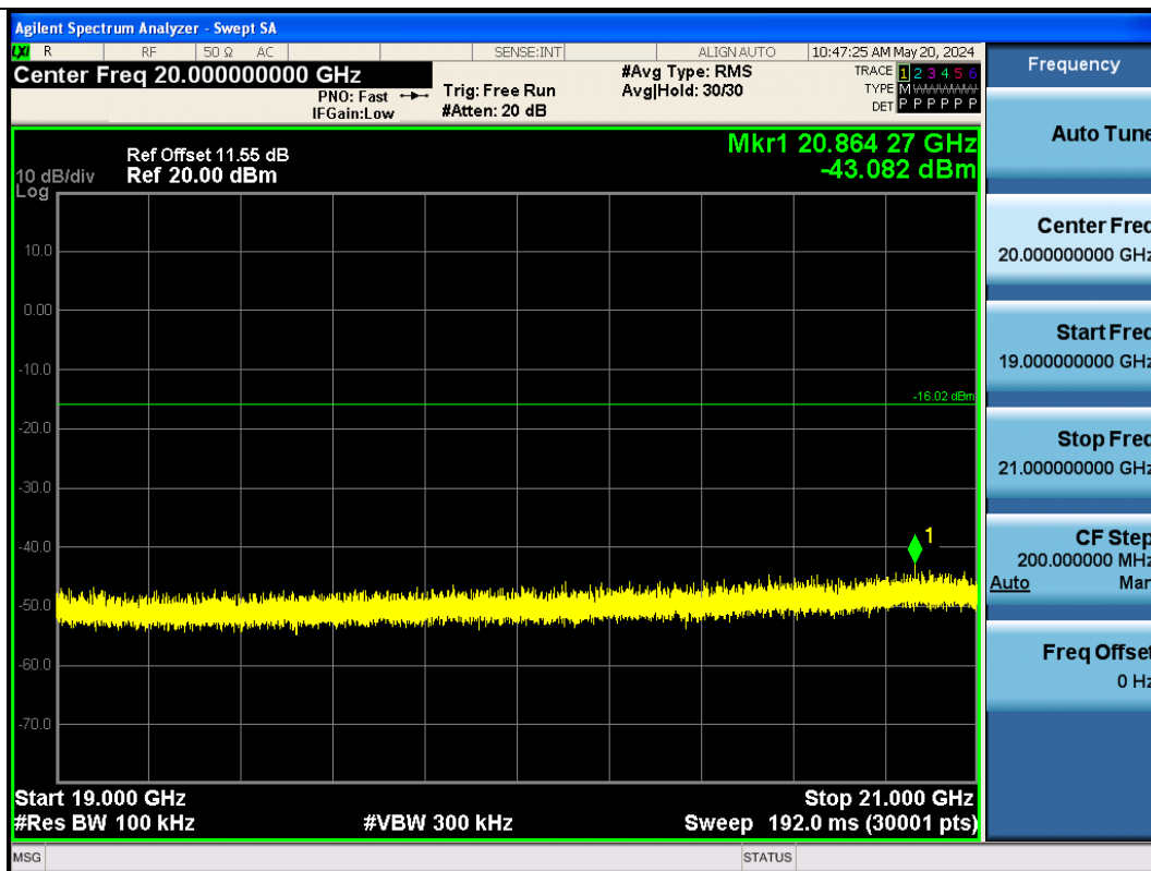
BLE_125K-Ant1-2440-19000~21000-PASS
