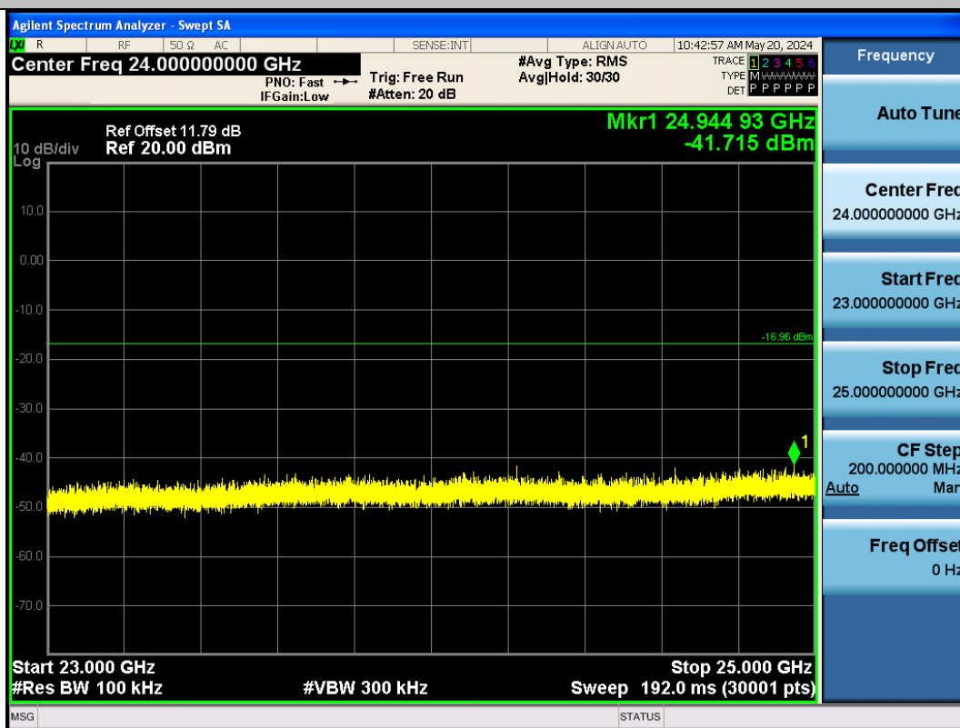
BLE_125K-Ant1-2402-23000~25000-PASS
