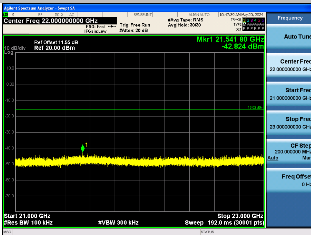
BLE_125K-Ant1-2440-21000~23000-PASS
