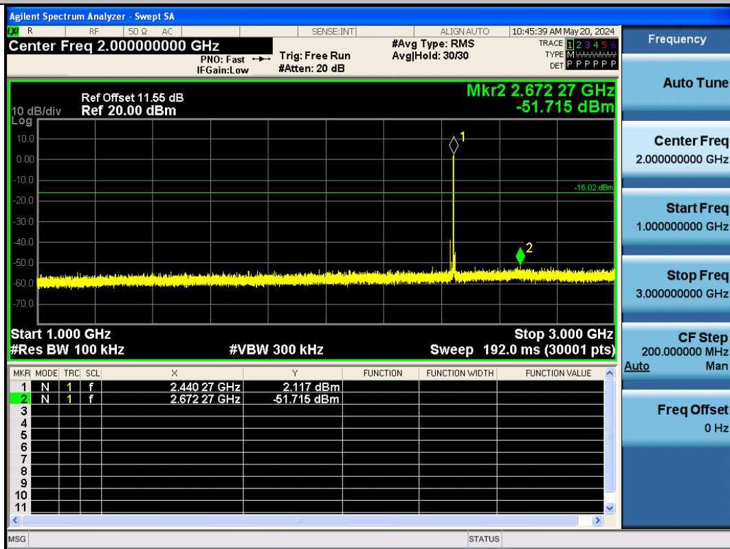
BLE_125K-Ant1-2440-1000~3000-PASS
