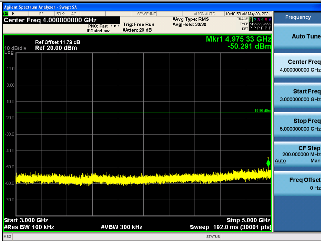
BLE_125K-Ant1-2402-3000~5000-PASS
