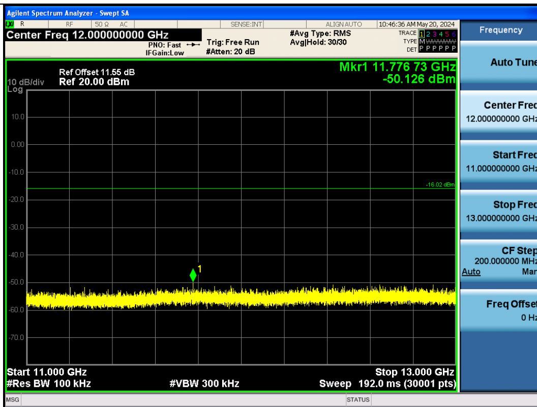
BLE_125K-Ant1-2440-11000~13000-PASS
