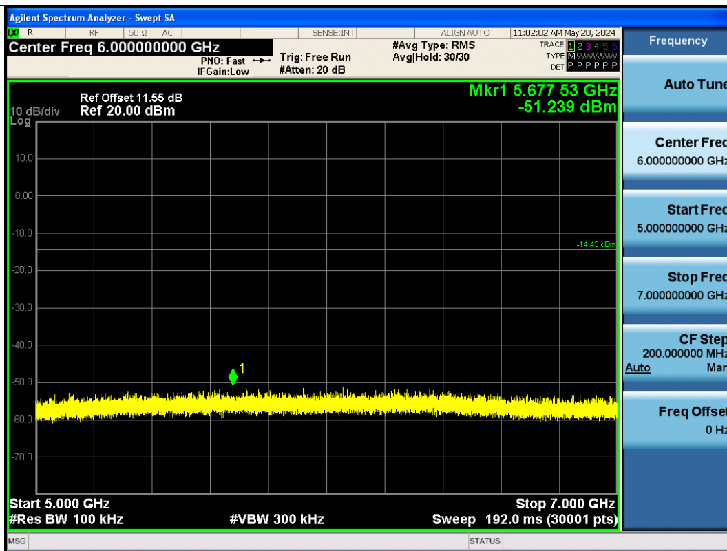
BLE_500K-Ant1-2440-5000~7000-PASS
