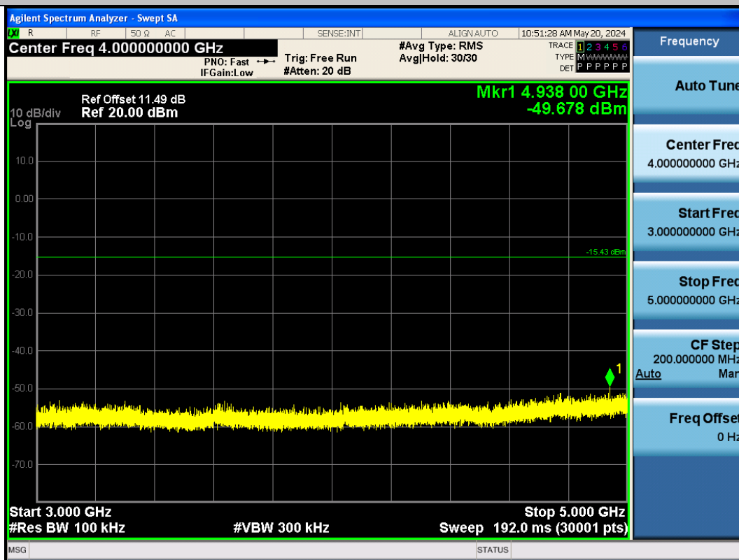
BLE_125K-Ant1-2480-3000~5000-PASS
