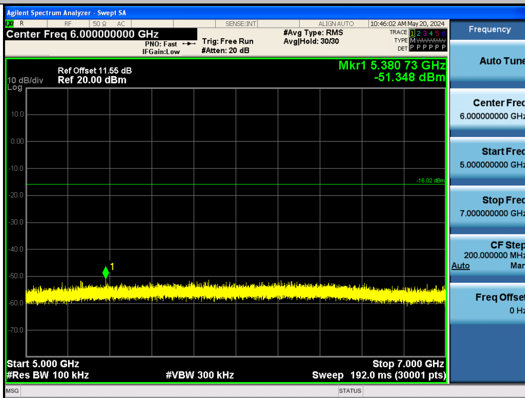
BLE_125K-Ant1-2440-5000~7000-PASS
