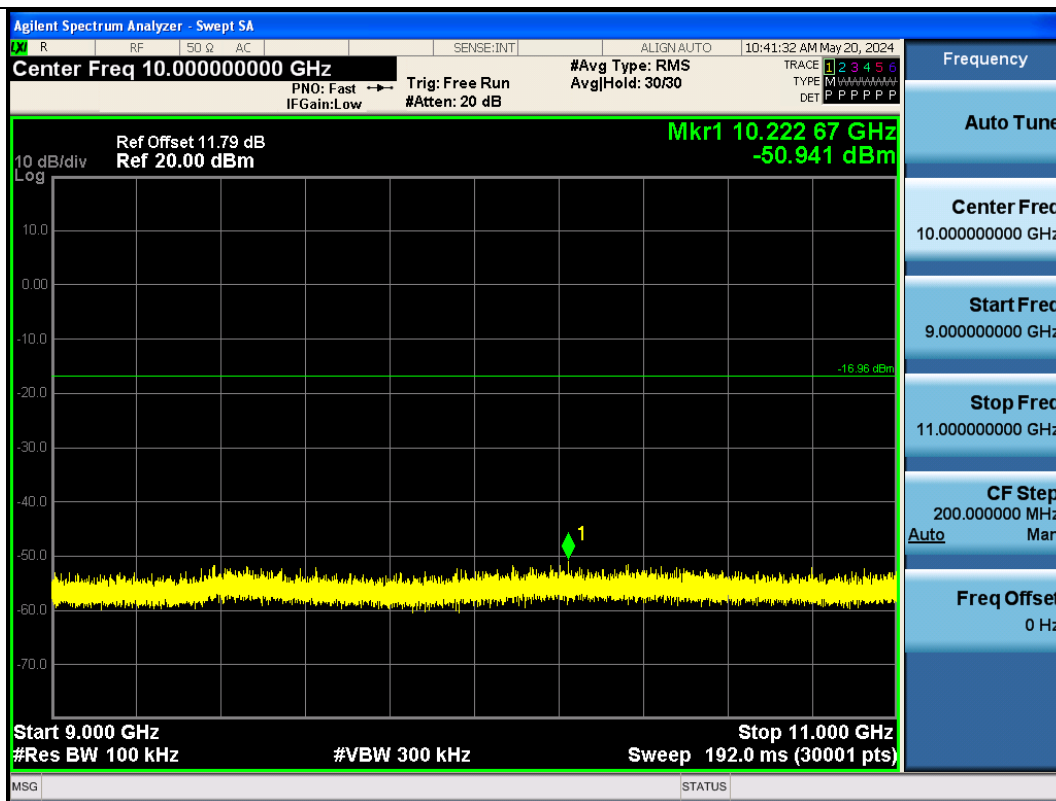
BLE_125K-Ant1-2402-9000~11000-PASS
