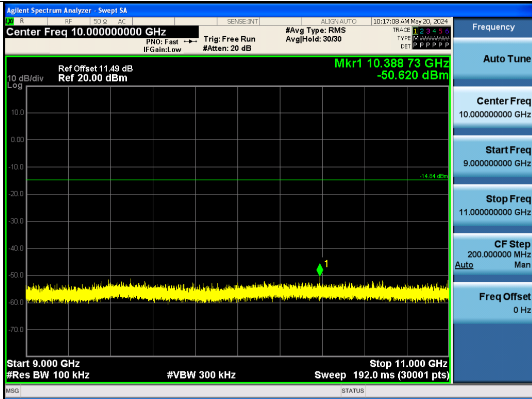
BLE_1M-Ant1-2480-9000~11000-PASS
