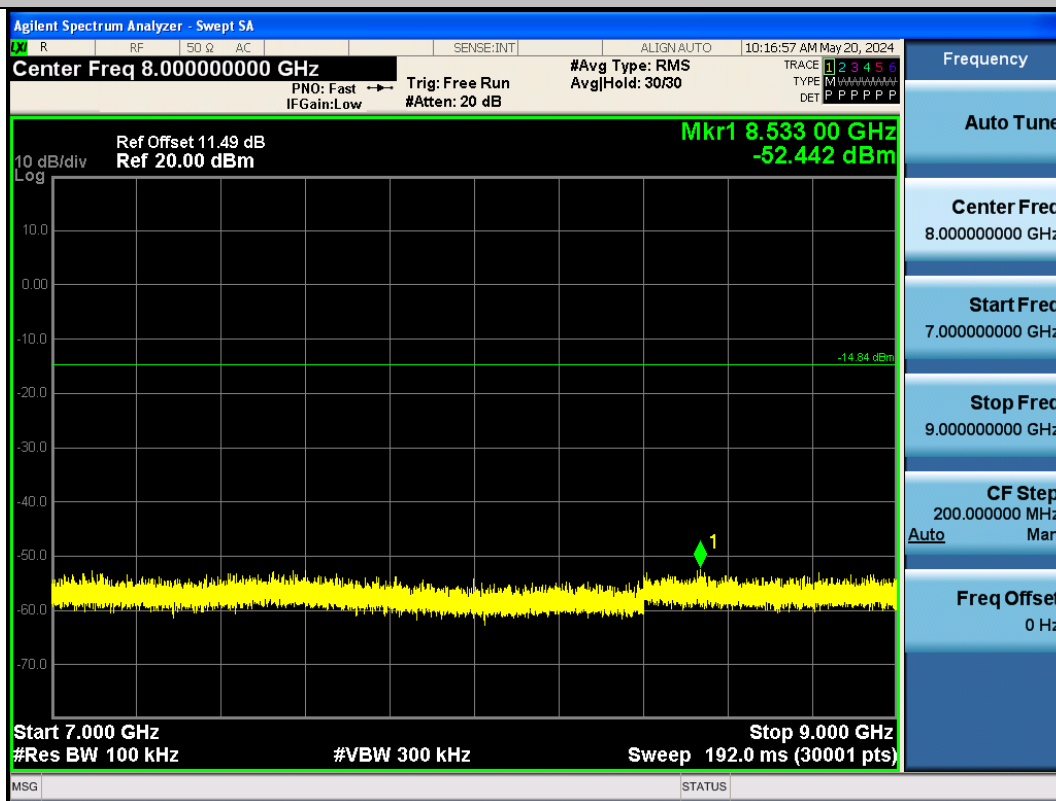
BLE_1M-Ant1-2480-7000~9000-PASS
