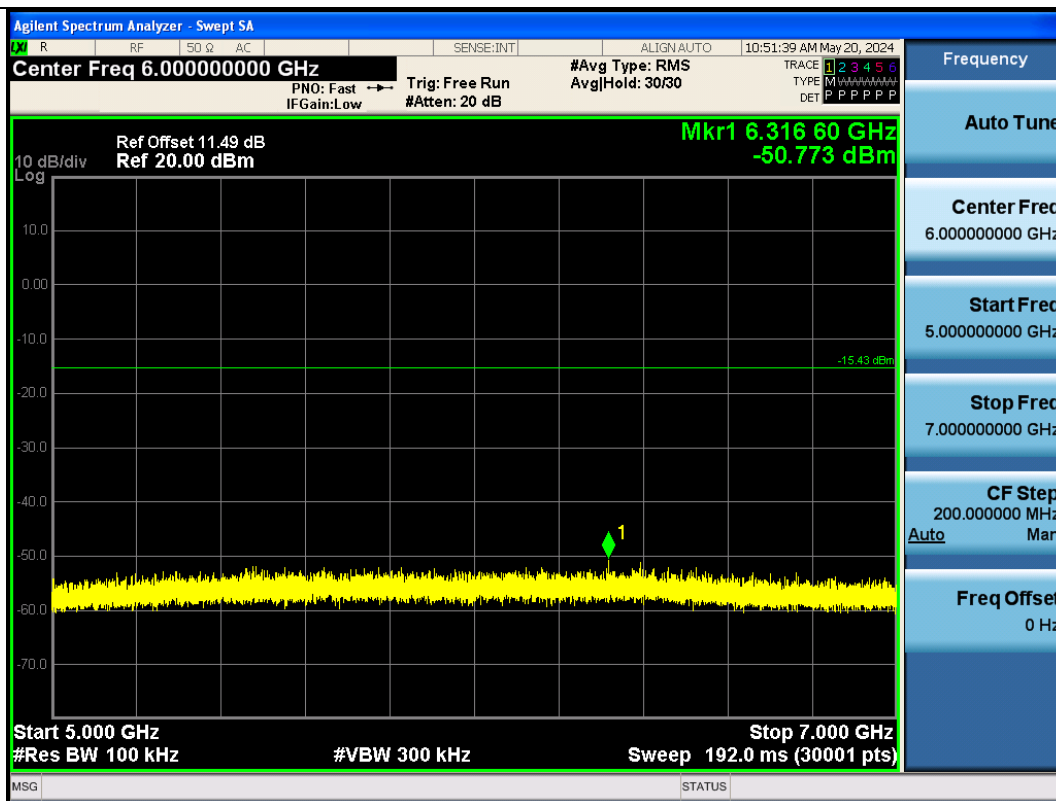
BLE_125K-Ant1-2480-5000~7000-PASS
