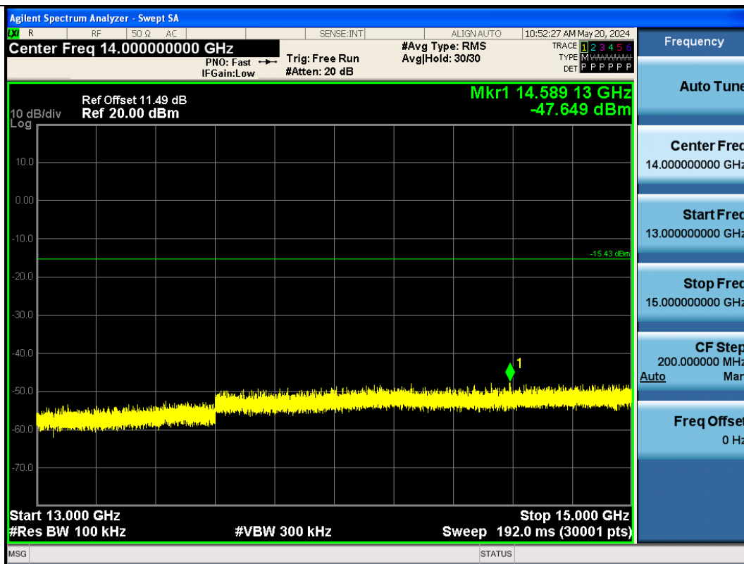
BLE_125K-Ant1-2480-13000~15000-PASS
