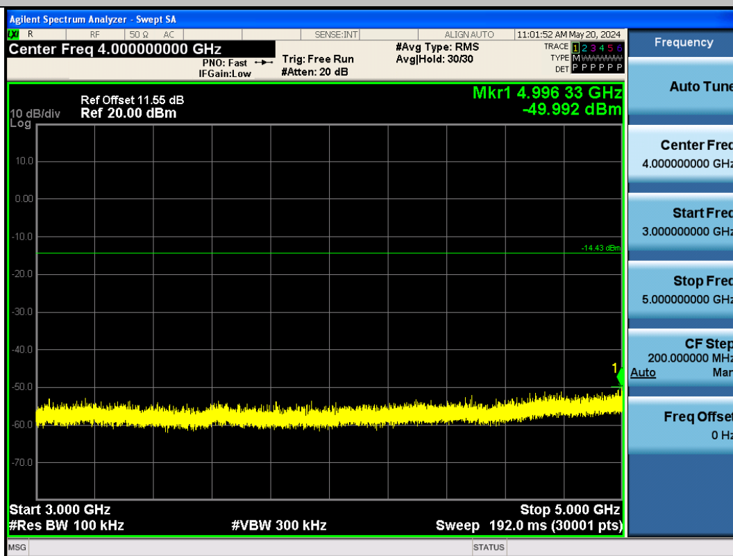
BLE_500K-Ant1-2440-3000~5000-PASS
