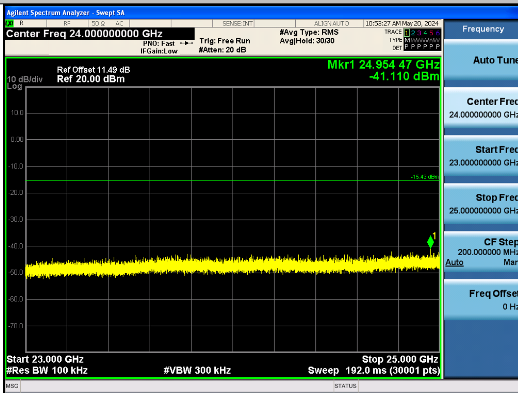
BLE_125K-Ant1-2480-23000~25000-PASS
