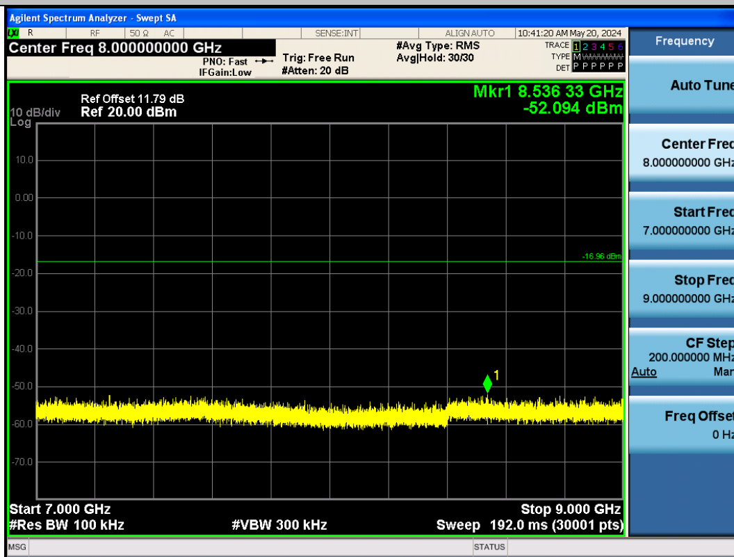
BLE_125K-Ant1-2402-7000~9000-PASS
