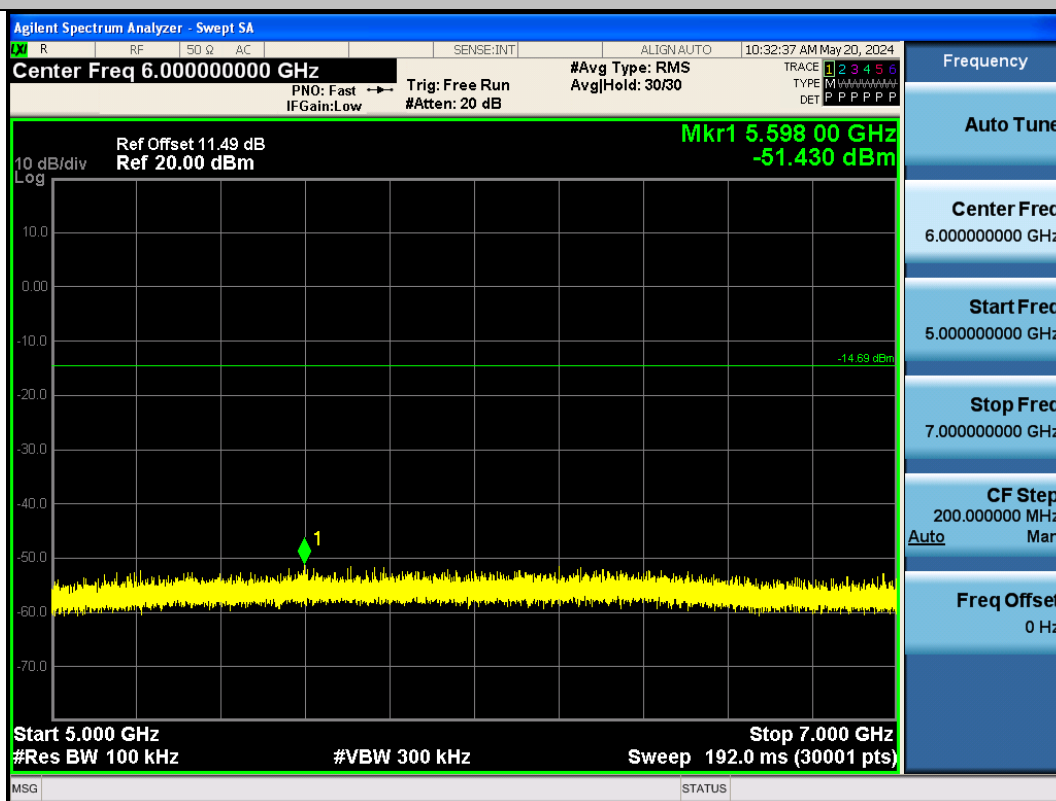
BLE_2M-Ant1-2480-5000~7000-PASS
