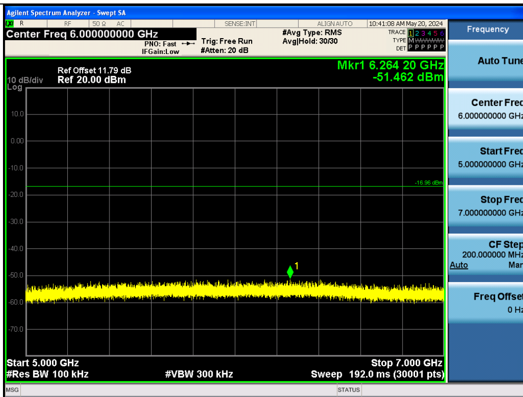
BLE_125K-Ant1-2402-5000~7000-PASS
