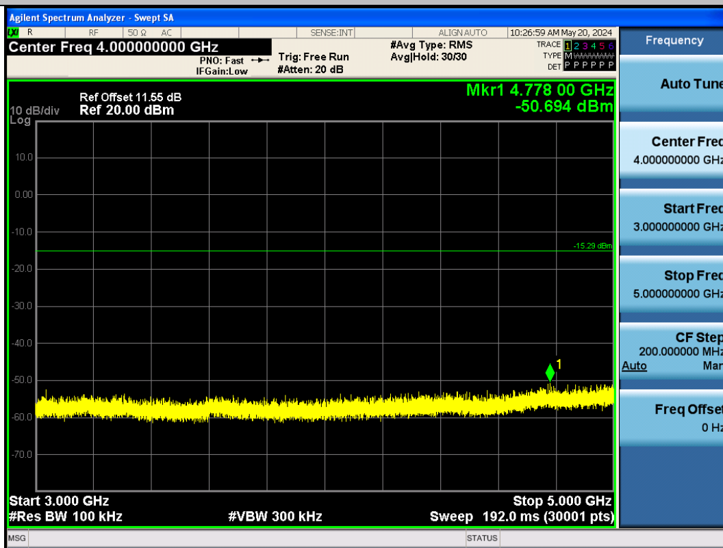
BLE_2M-Ant1-2440-3000~5000-PASS
