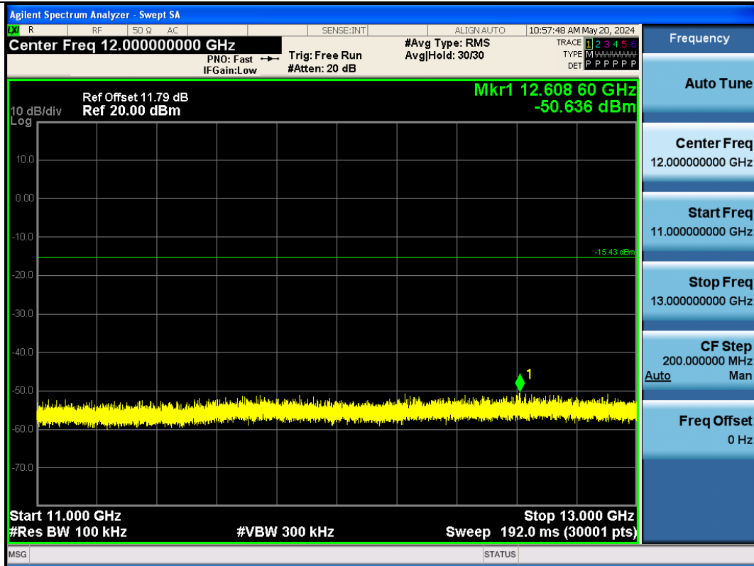
BLE_500K-Ant1-2402-11000~13000-PASS
