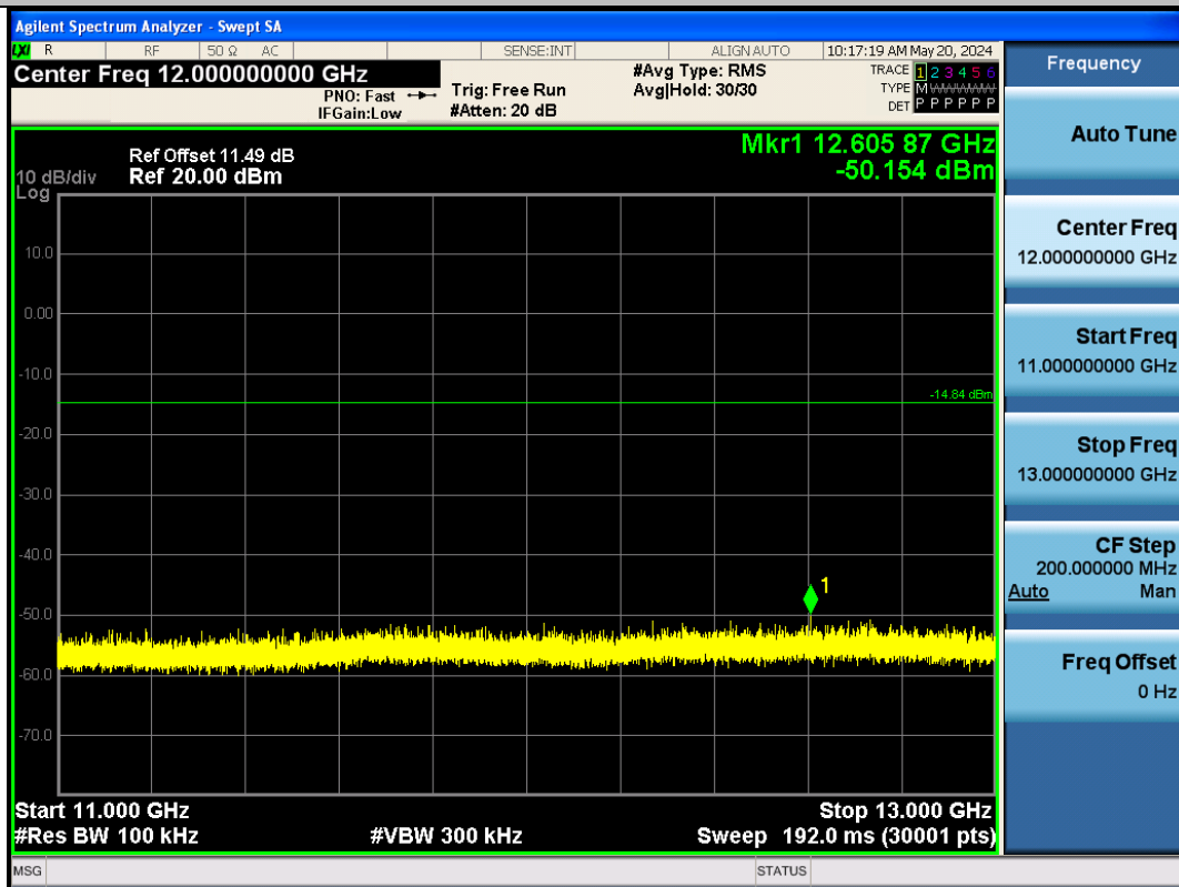
BLE_1M-Ant1-2480-11000~13000-PASS
