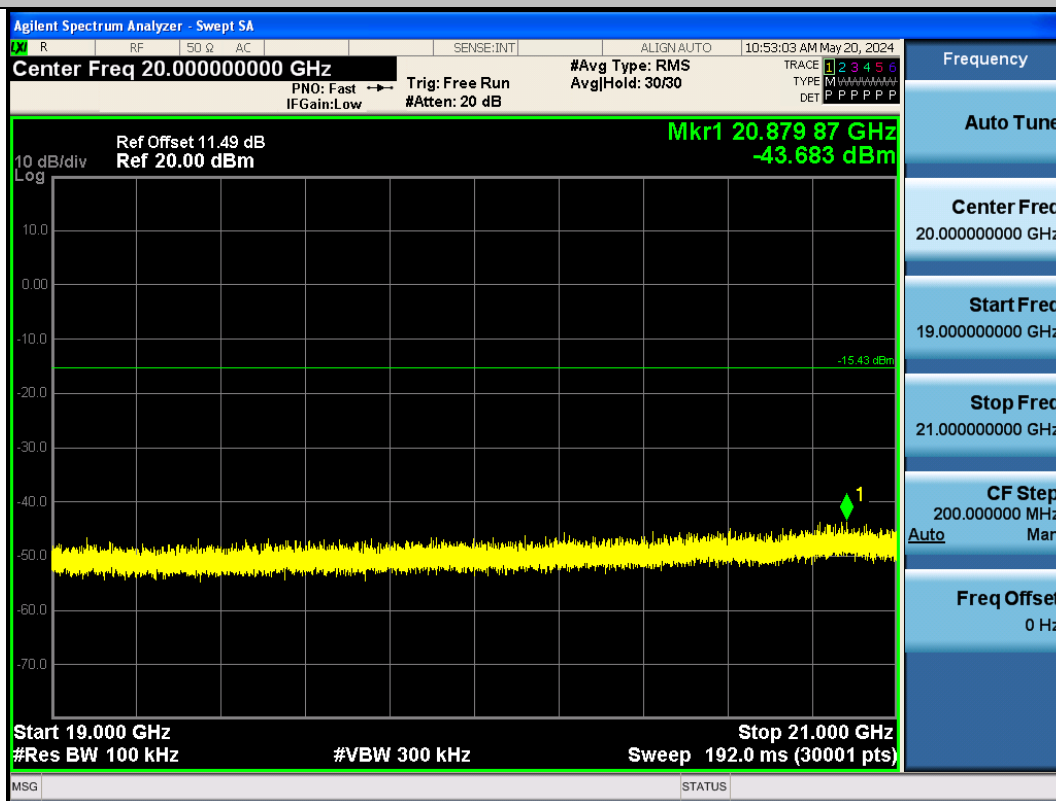
BLE_125K-Ant1-2480-19000~21000-PASS
