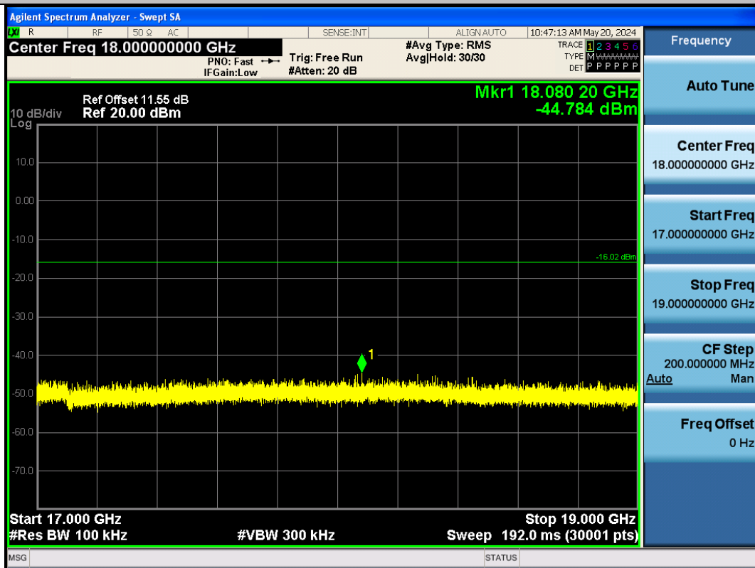
BLE_125K-Ant1-2440-17000~19000-PASS
