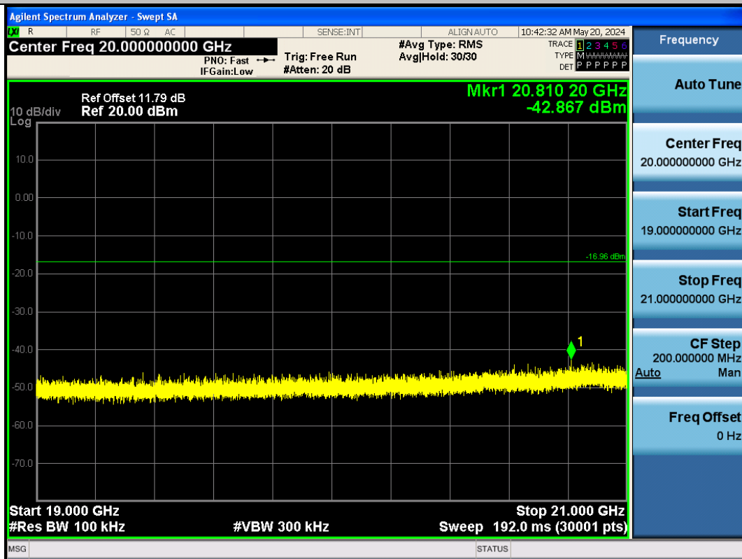
BLE_125K-Ant1-2402-19000~21000-PASS
