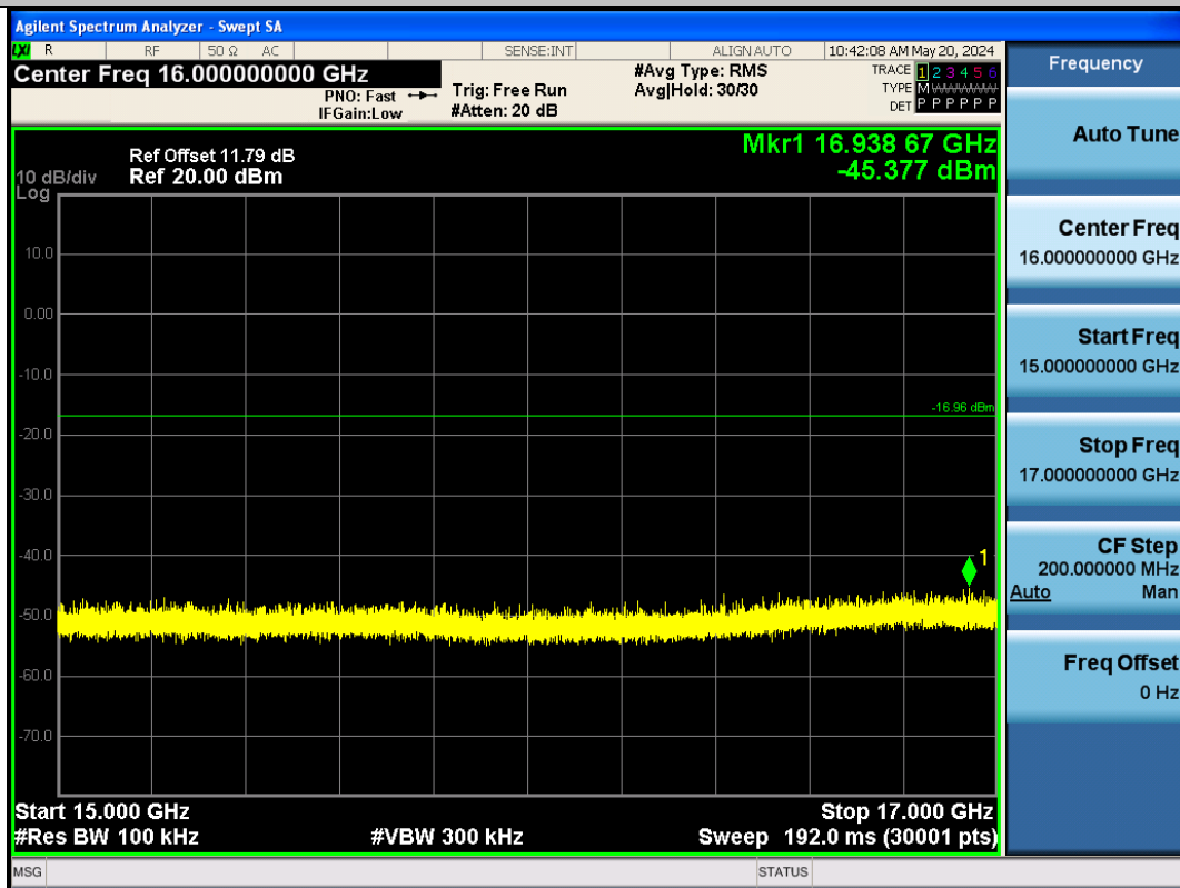
BLE_125K-Ant1-2402-15000~17000-PASS
