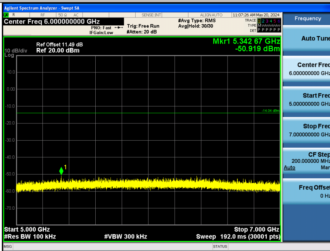
BLE_500K-Ant1-2480-5000~7000-PASS
