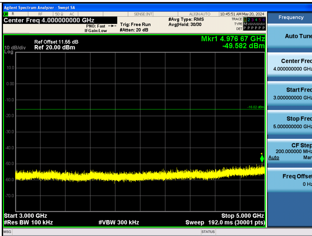
BLE_125K-Ant1-2440-3000~5000-PASS
