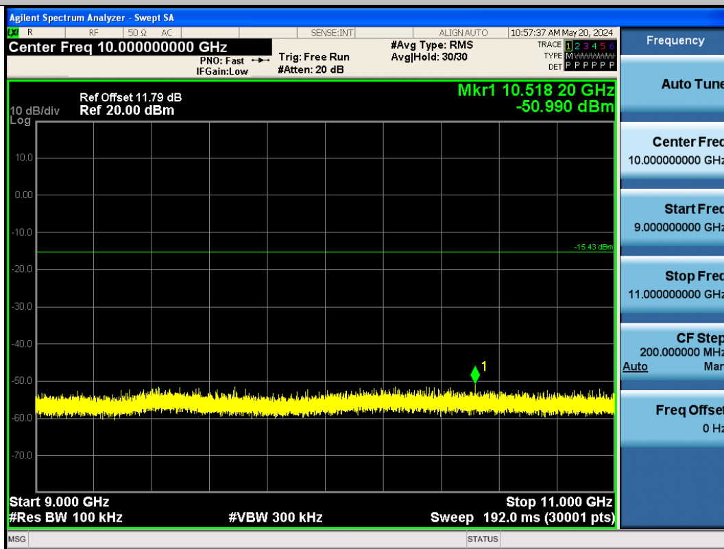
BLE_500K-Ant1-2402-9000~11000-PASS
