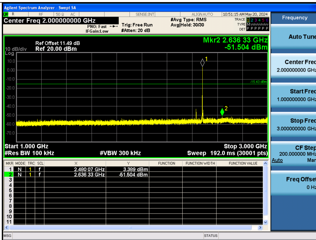
BLE_125K-Ant1-2480-1000~3000-PASS
