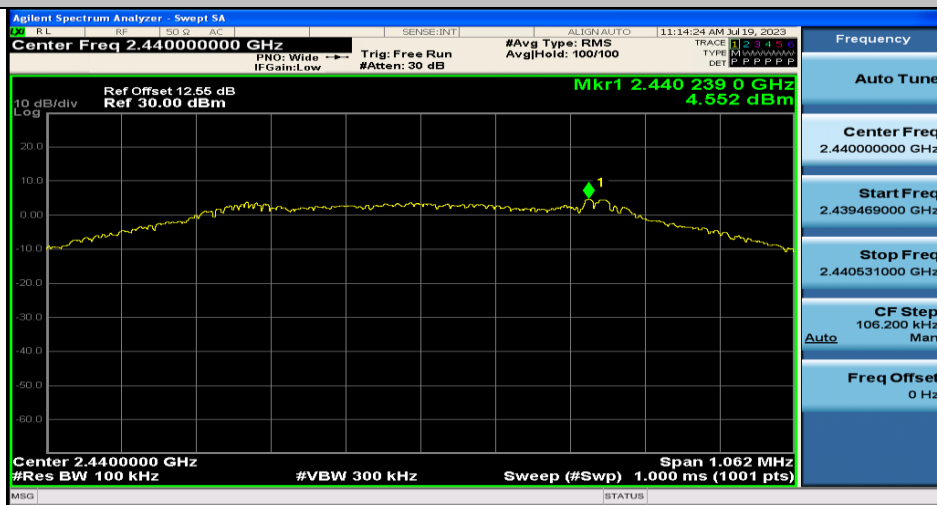
BLE_1M-Ant1-2440
