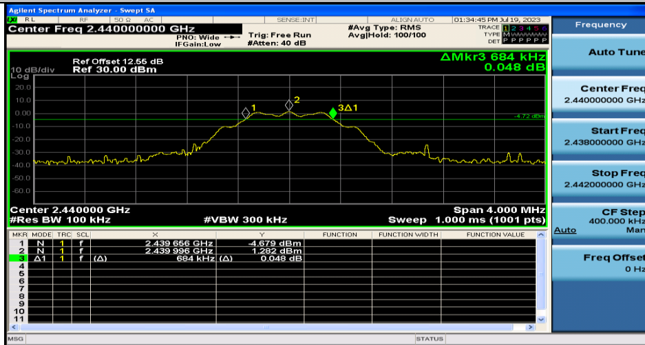
BLE_125K-Ant1-2440
