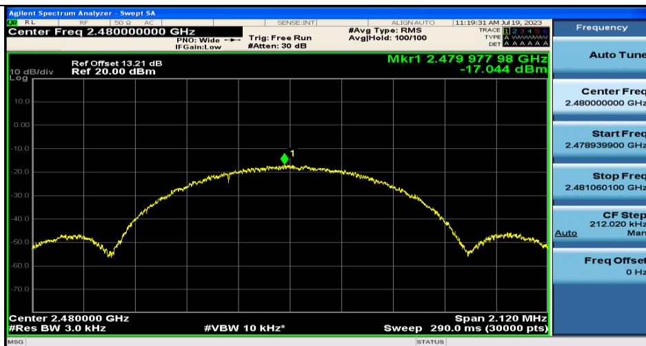
BLE_1M-Ant1-2480
