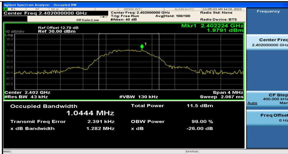
BLE_1M-Ant1-2402
