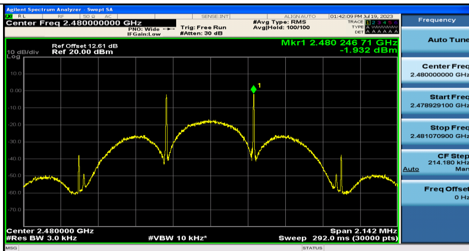
BLE_125K-Ant1-2480
