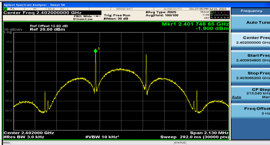
BLE_125K-Ant1-2402
