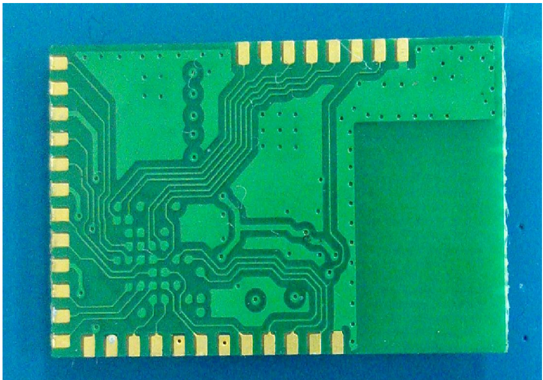
(2) EUT Photo (CYBLE-224110-00)
