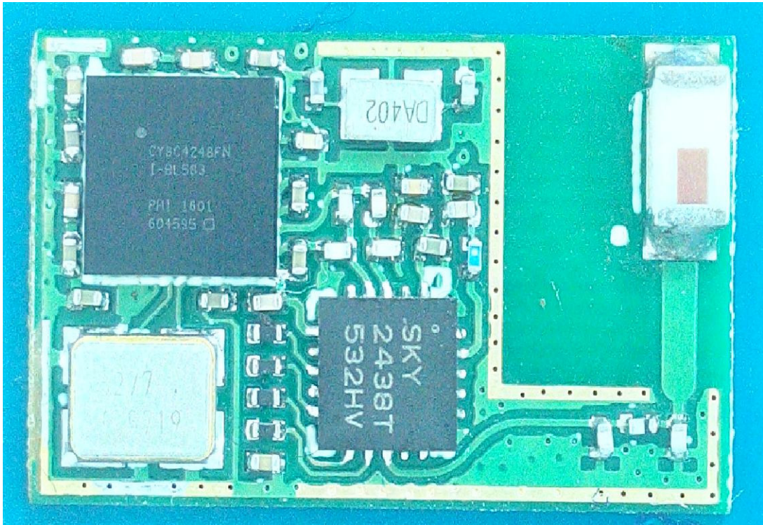
(3) EUT Photo (CYBLE-224116-01)
