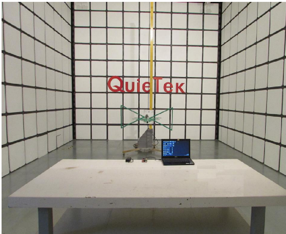
Description: Radiated Emission Test Setup for Below 1GHz
