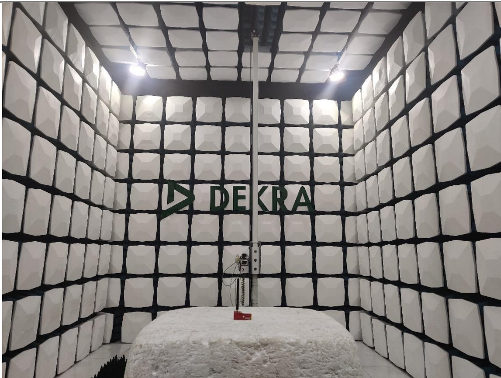
Description: Radiated emission(Above 18G)
