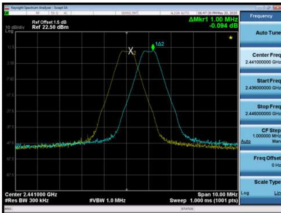
Mode 1 CH39(2441MHz)
