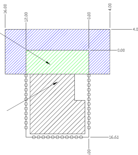
Figure 4. Optional Additional Host PCB Keep Out Area Around the CYBT-243053-02 PCB Antenna
