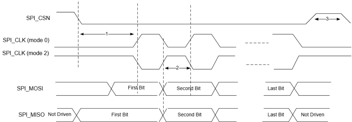
Figure 14. SPI Timing, Mode 0 and 2
