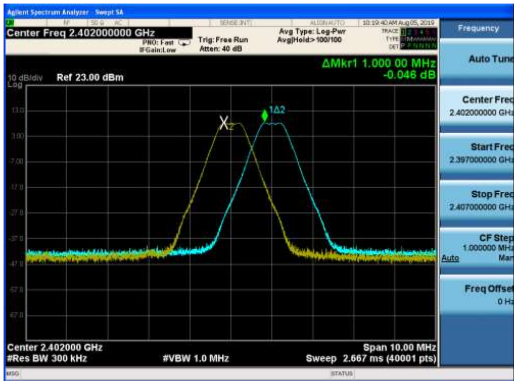
Channel 00 (2402MHz)
