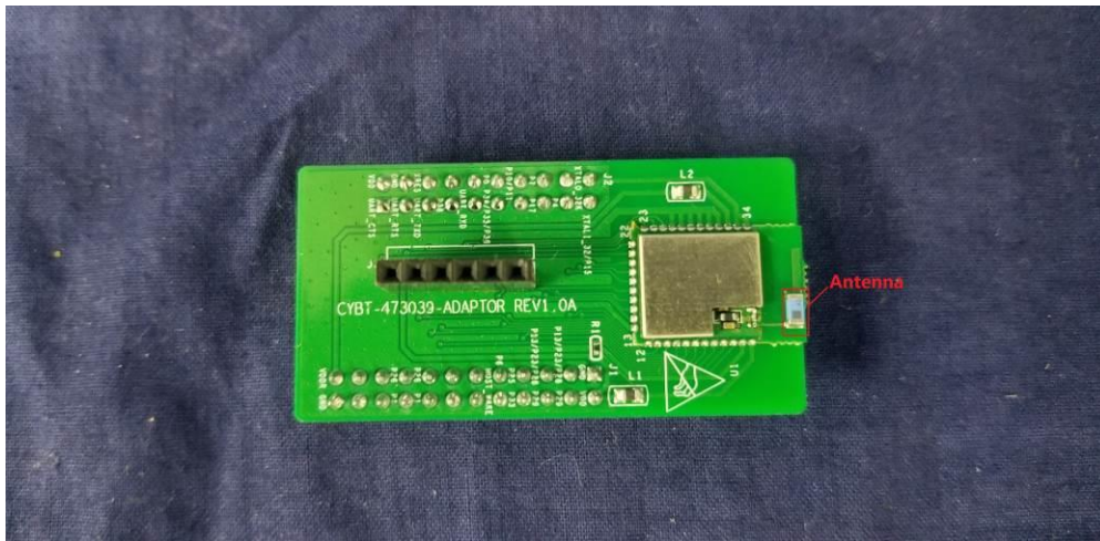
(1) EUT Photo
