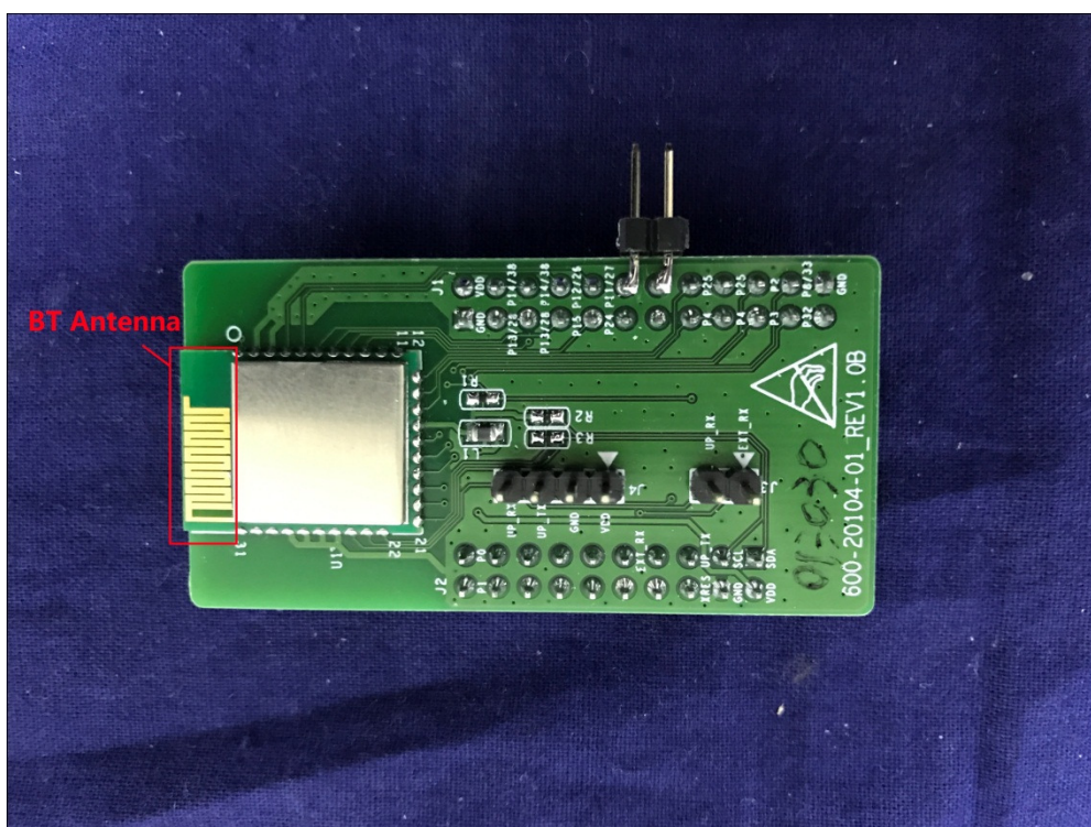
(6) EUT Photo(CYBLE-013030-00)
