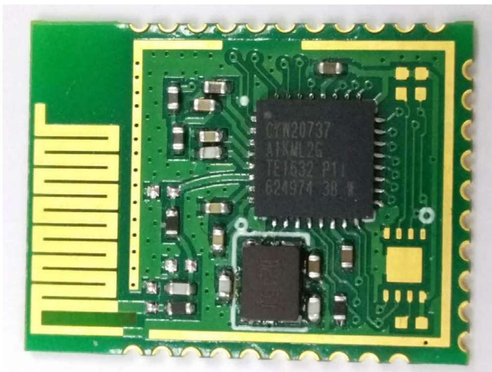
(10) EUT Photo(CYBLE-013030-00)
