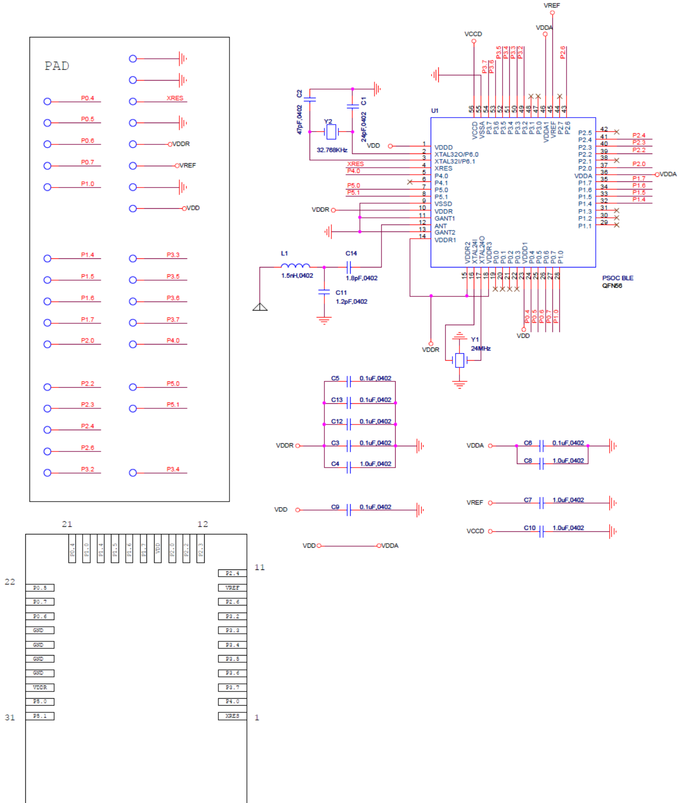
Figure 7. CYBLE-212019-00 Schematic Diagram
