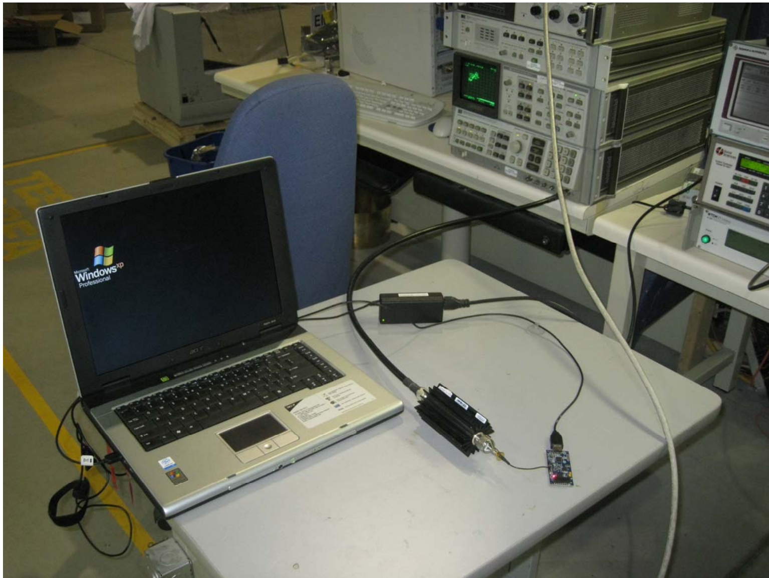
Figure 3 – Antenna port conducted emissions
