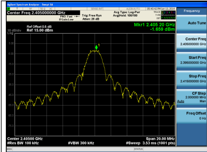
PSD-Zigbee 2405
