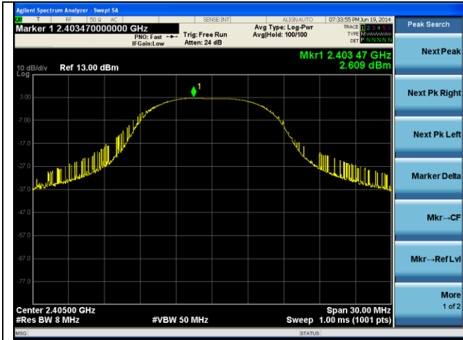
PWR-Zigbee 2405
