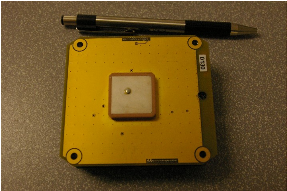
GPS / RADIO BOARD TOP
