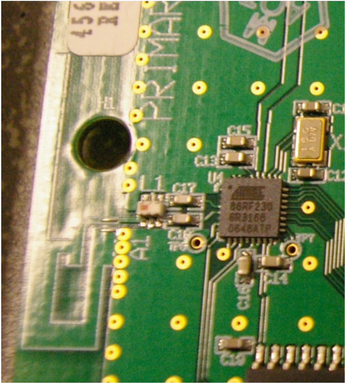
RADIO CIRCUIT WITH ATMEL AT86RF230 IC
