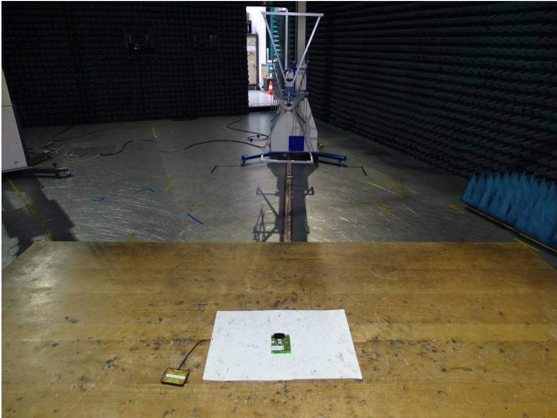
Photo 2: Test setup for radiated measurements (stand alone, EUT supplied by a battery) 30 MHz - 1 GHz
