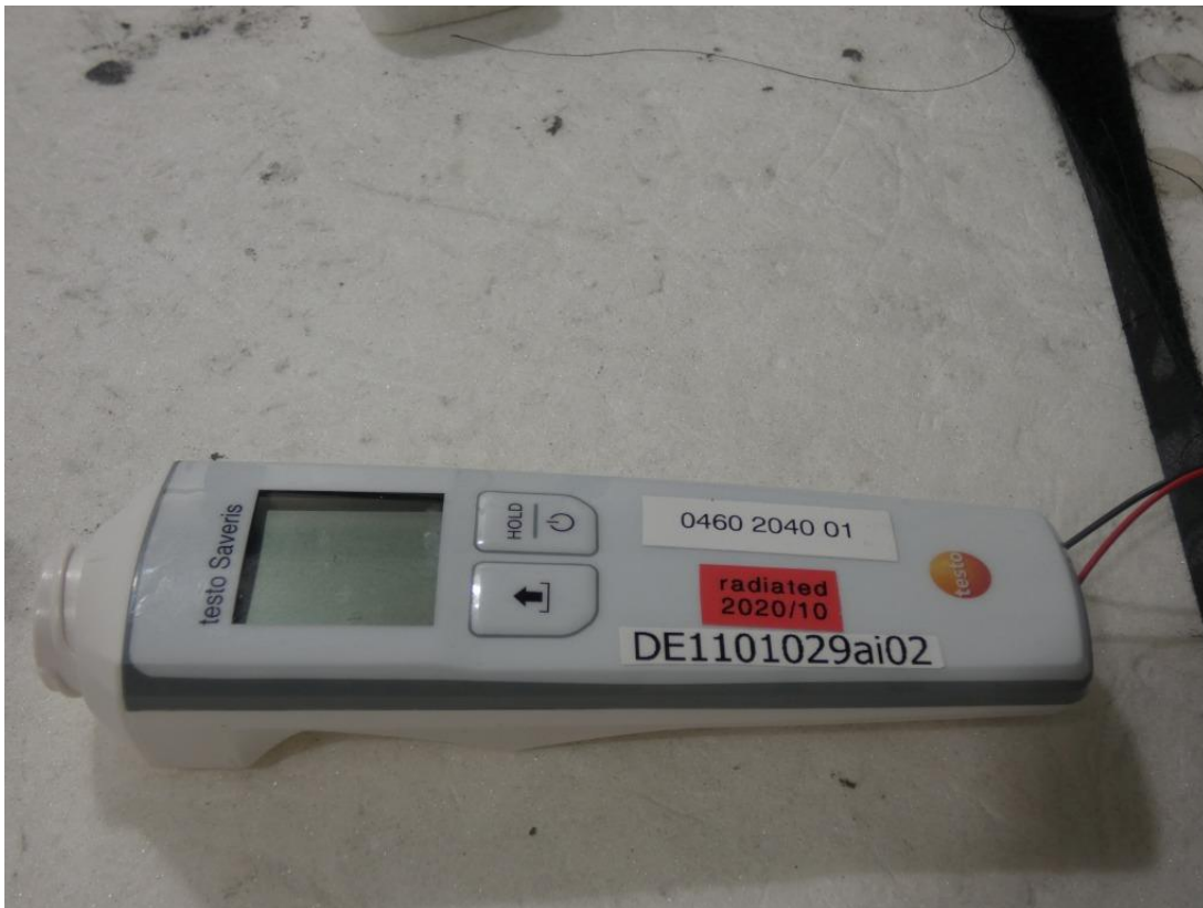
Photo 4: Test setup for radiated measurements, EUT
