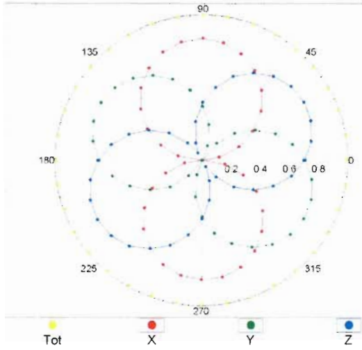
f=600 MHz,TEM
