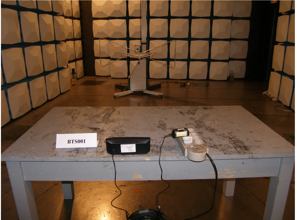
Photograph 1: Set-up for Radiation Measurement below 1GHz
