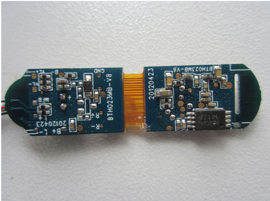
4. Mainboard rear view with shielding
