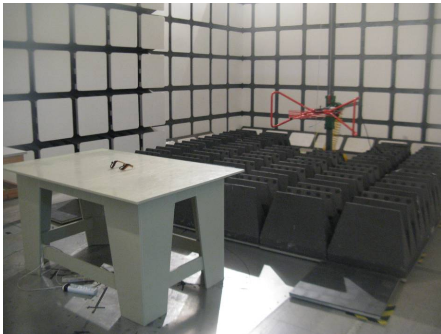
Below 1 GHz: Radiated Emissions - Rear View (Transmitting mode)
