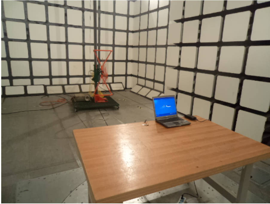
Radiated Emissions - Front View (Charging mode)
