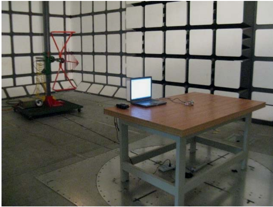
Below 1 GHz: Radiated Emissions (TX Mode) - Rear View
