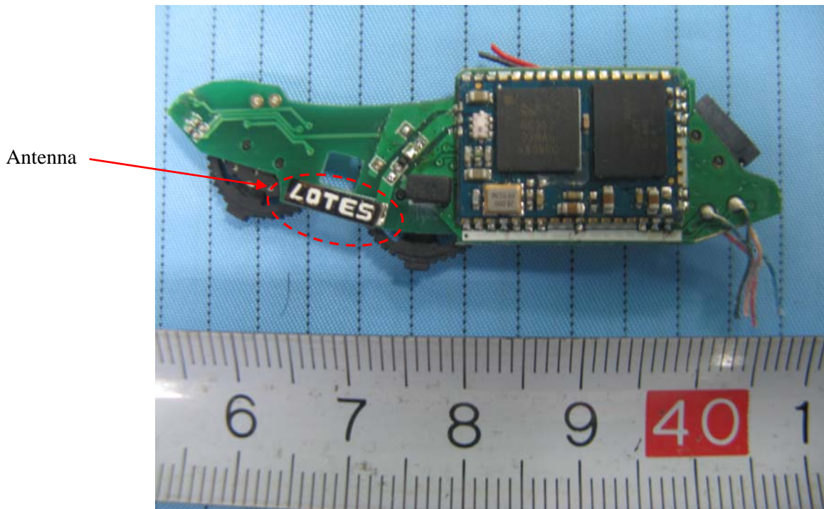
EUT- Main Board Components Bottom View
