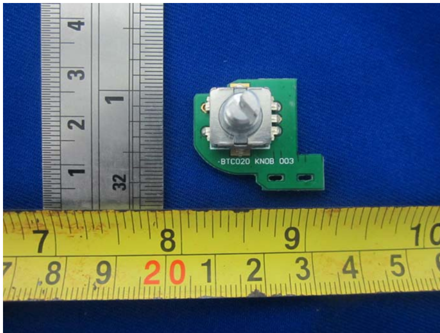
EUT –Knob Board Top View
