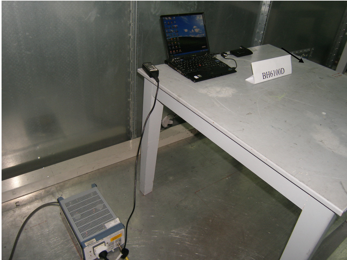
Photograph 1: Set-up for Conducted Emission Measurement
