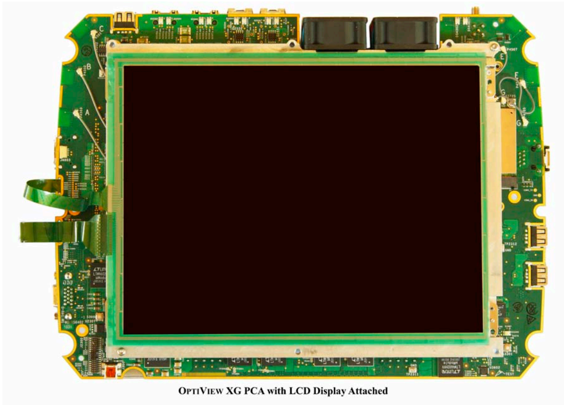
Figure 1: Internal Photo of OptiView XG PCA with LCD Display
