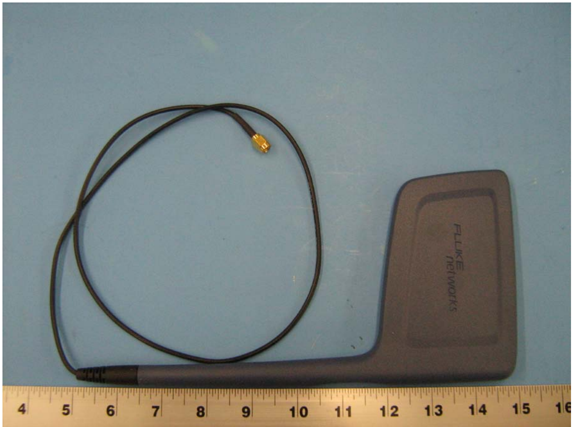
Figure 6: External Photo of EUT – External Receiving Antenna (Omni Directional)
