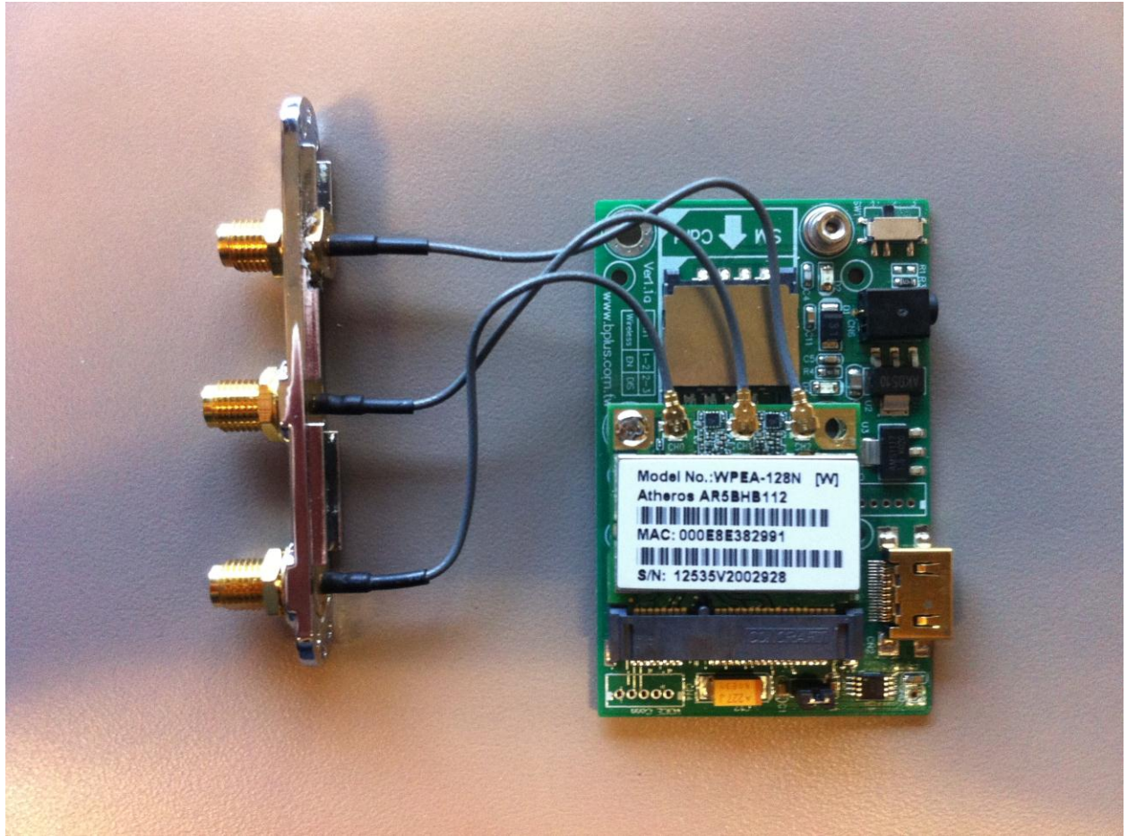
Complete Assembly - Internal
