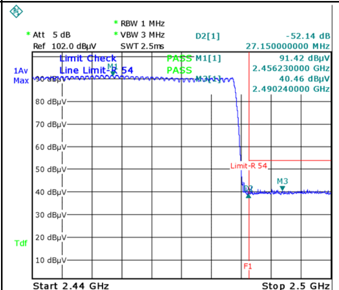
GFSK-Hopping Right Side-AV
