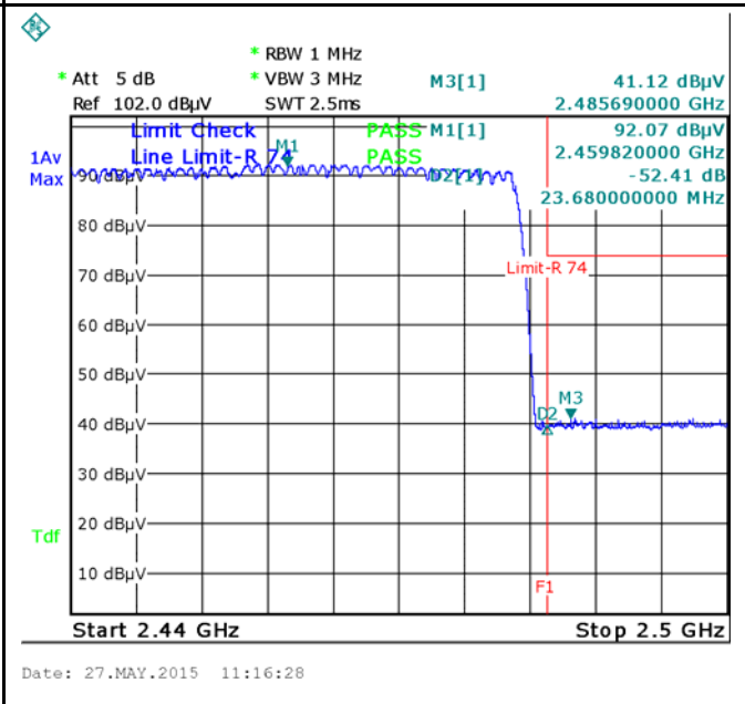
8DPSK-Hopping Right-AV
