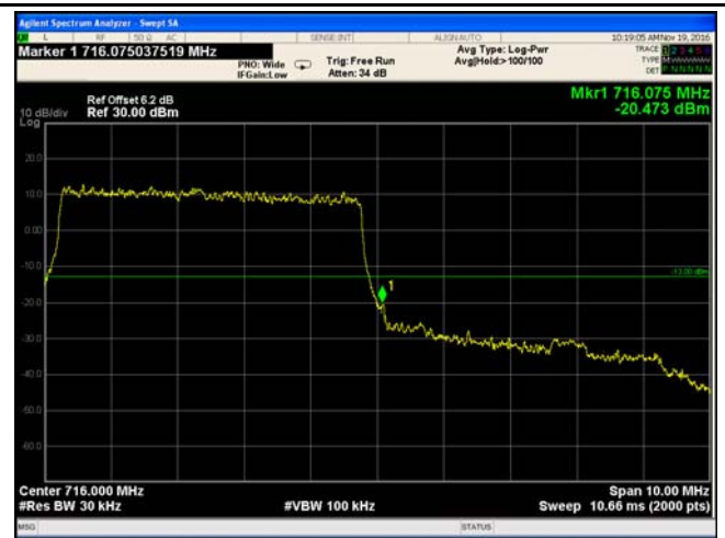
LTE Band XVII - High Channel 16QAM-5
