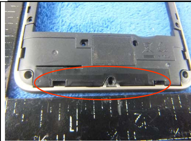
GSM/PCS/UMTS-FDD-Antenna View
