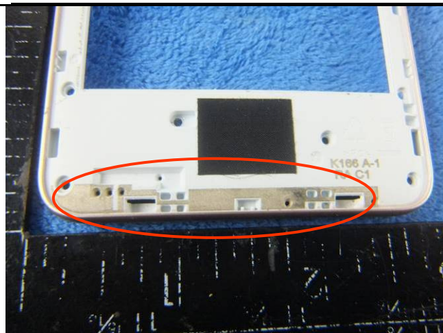
GSM/PCS/UMTS-FDD-Antenna View
